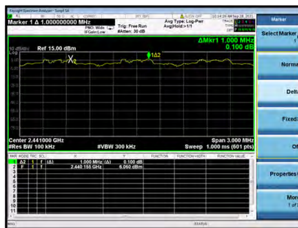
8-DPSK
