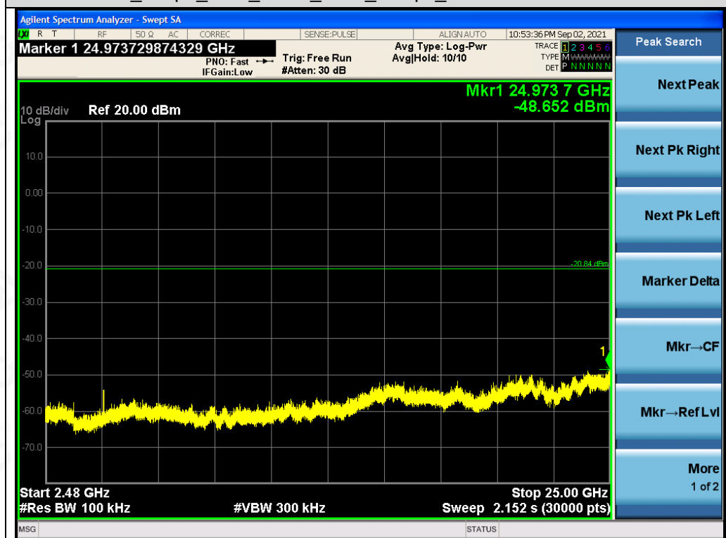
Test Graph EDR ANT1 2402 2Mbps Higher Band Emissions
