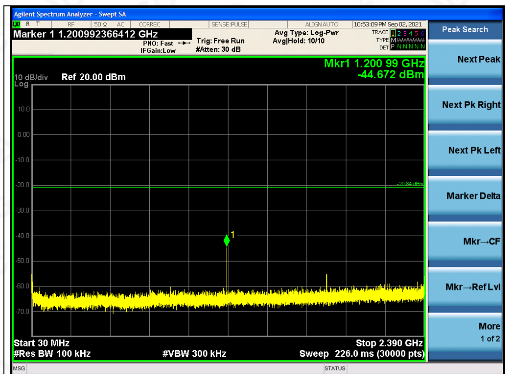
Test Graph EDR ANT1 2402 2Mbps Lower Band Emissions
