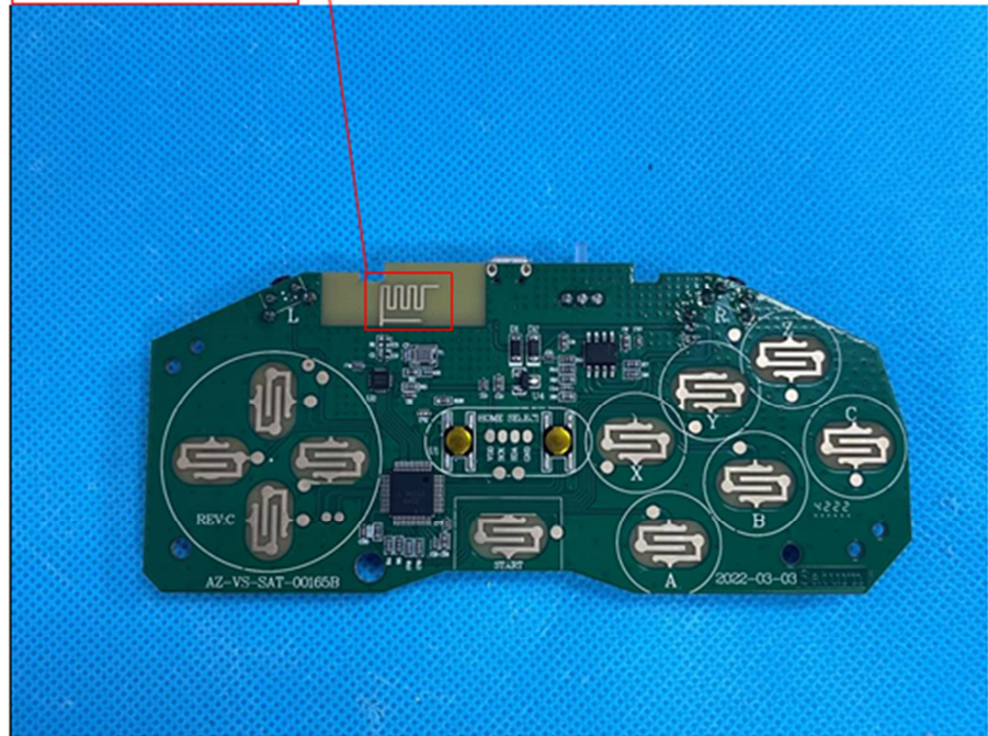
Transmitter Antenna
