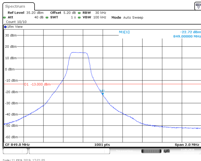
BAND 26 3MHz 16QAM 27025 15RB#0
