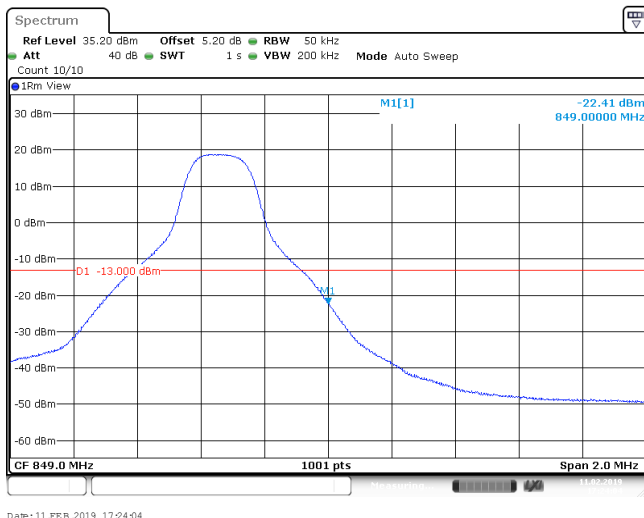
BAND 26_5MHz_QPSK_27015_25RB#0
