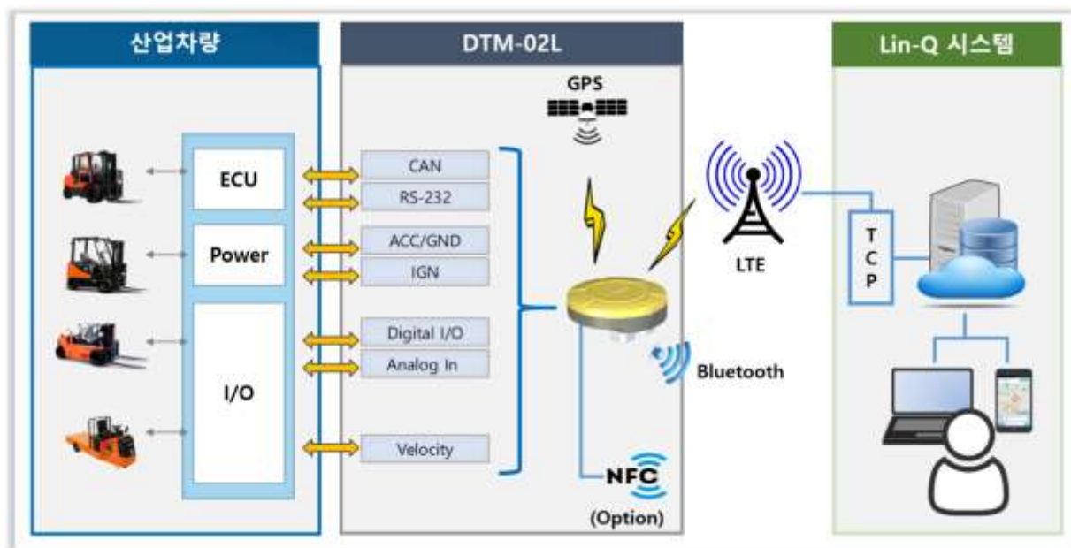
Figure 1 Lin-Q System
