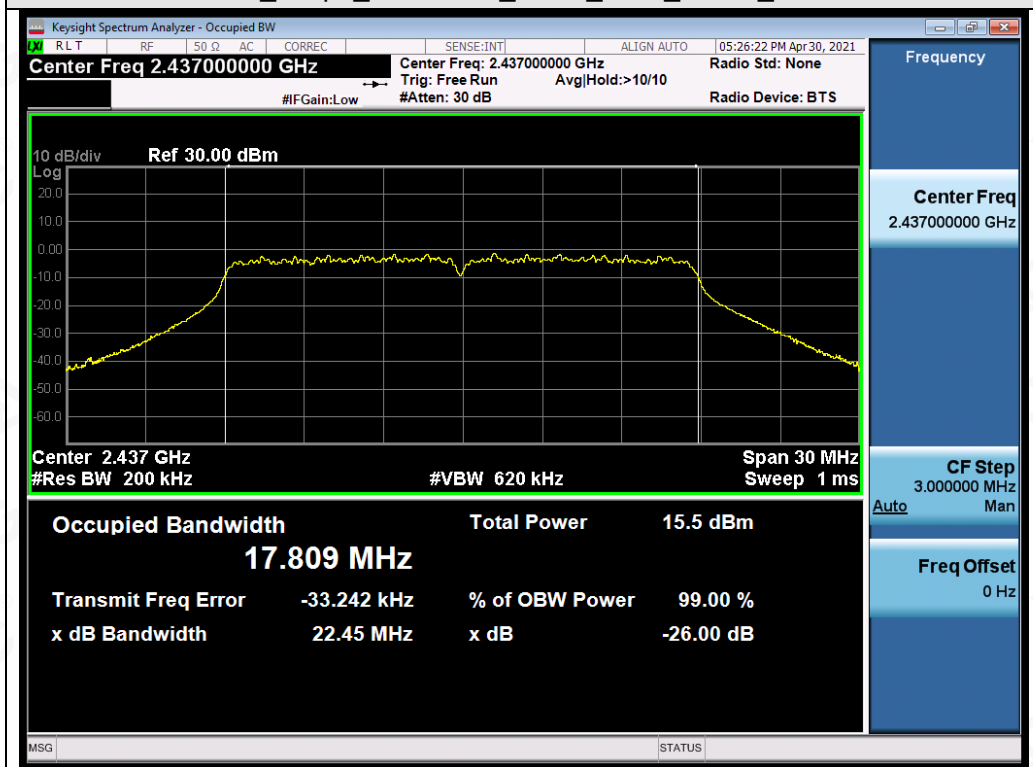
Test_Graph_802.11n20_ANT1_2437_MCS0_OBW
