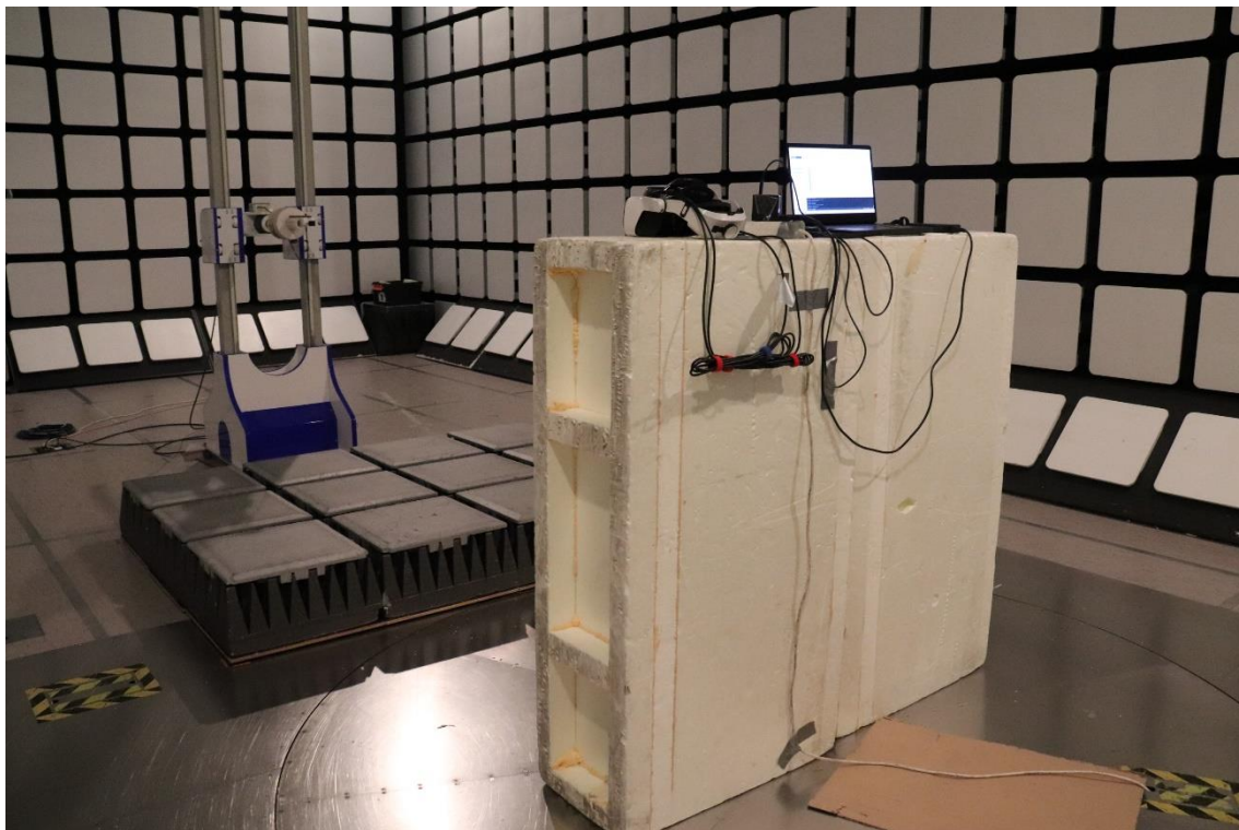
Photograph 6. Test setup for radiated emissions 18 – 26.5 GHz
