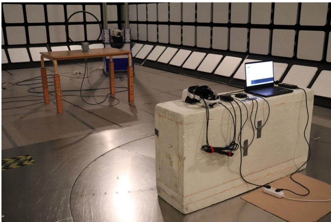
Photograph 3. Test setup for radiated emissions 9 kHz – 30 MHz
