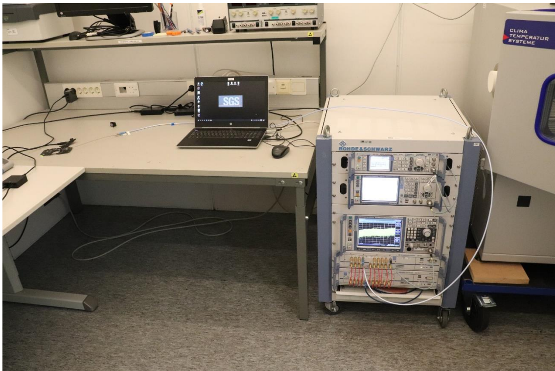
Photograph 1. Test setup for conducted RF tests
