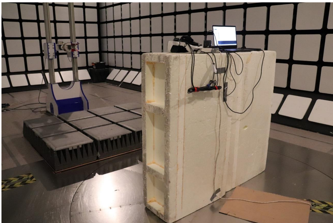
Photograph 5. Test setup for radiated emissions 1 – 18 GHz
