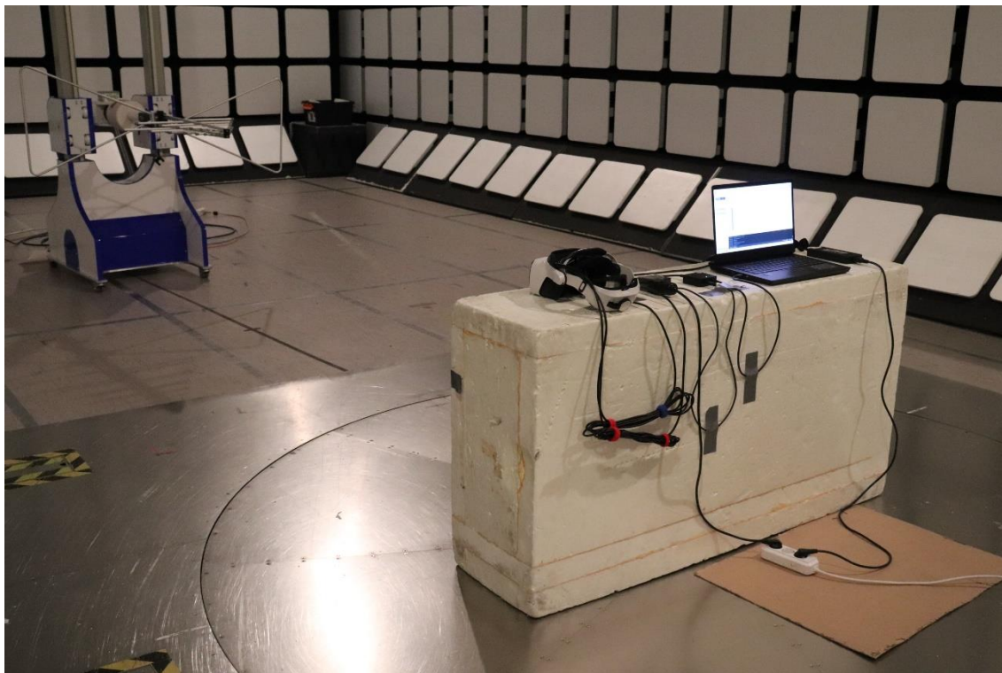
Photograph 4. Test setup for radiated emissions 30 – 1000 MHz
