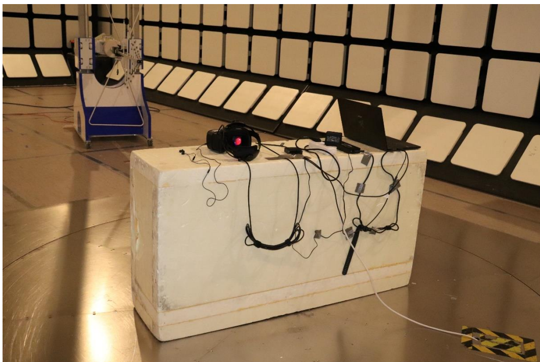
Photograph 3: Radiated emission test setup 30 MHz – 1000 MHz
