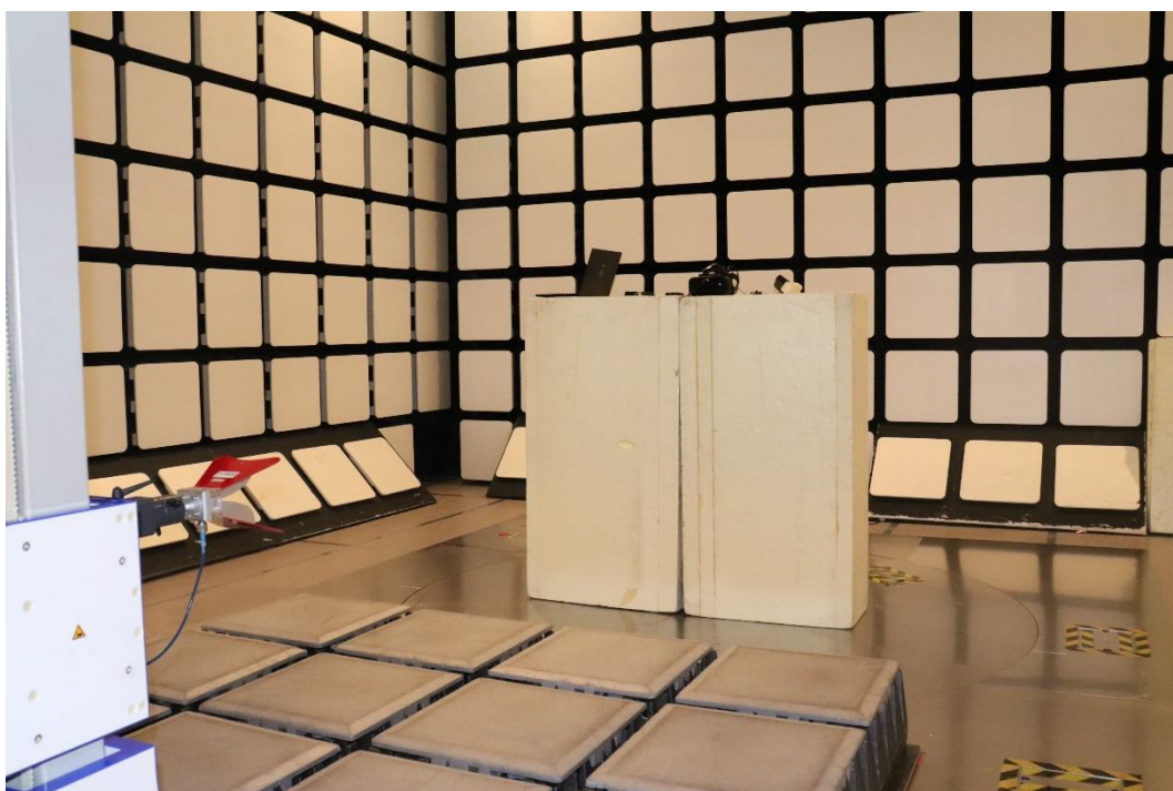
Photograph 4: Radiated emission test setup 1 GHz – 18 GHz
