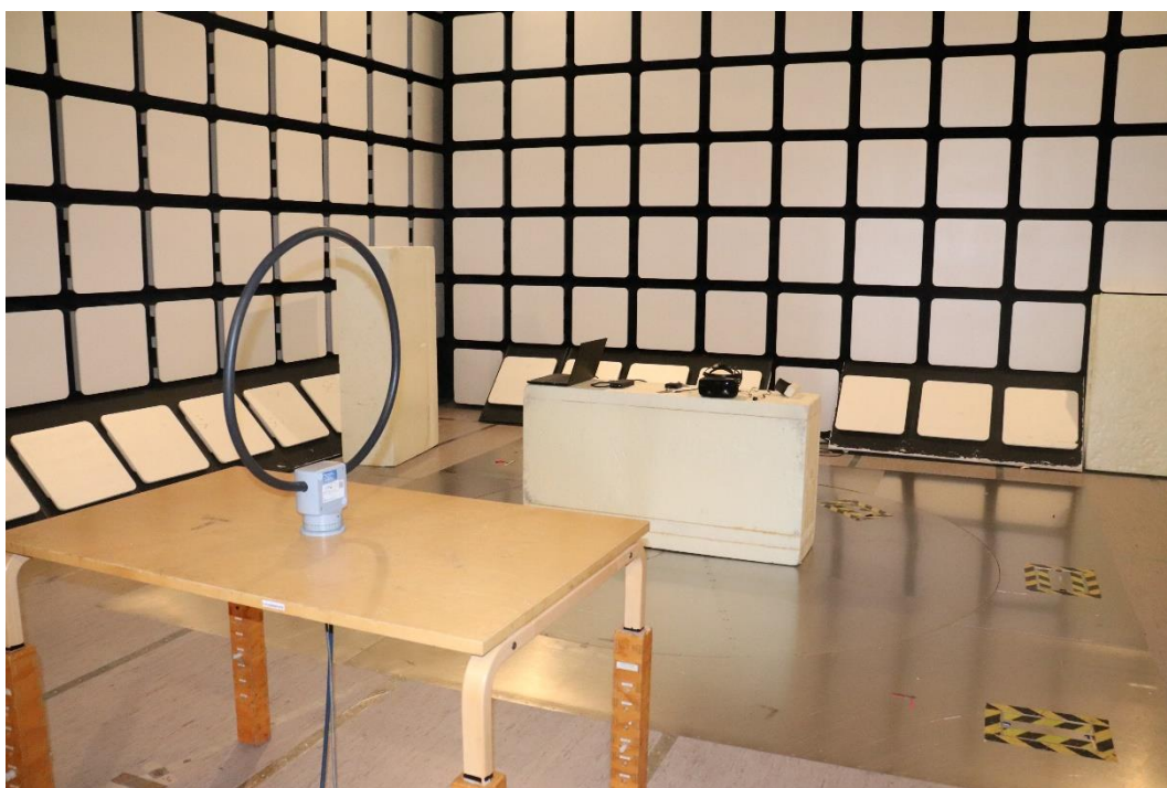
Photograph 2: Radiated emission test setup 9 kHz – 30 MHz
