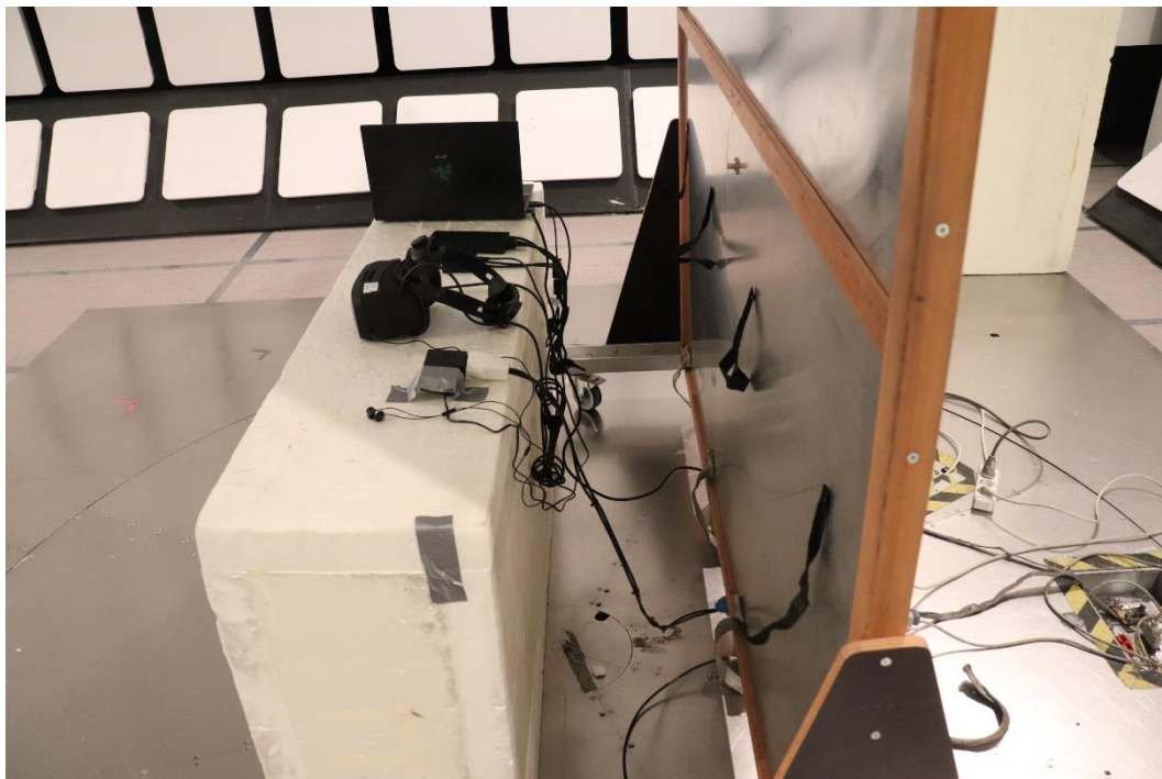
Photograph 1: Conducted emission test setup
