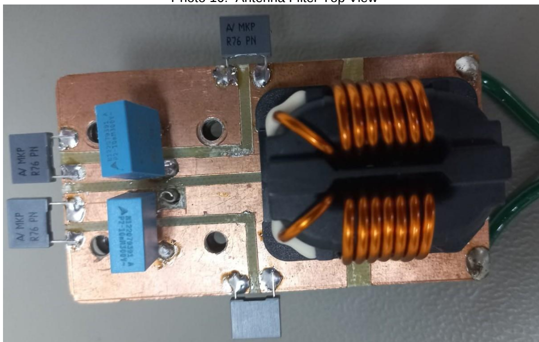
Photo 10: Antenna Filter Top View
