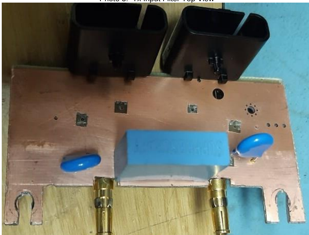
Photo 5: Tx Input Filter Top View
