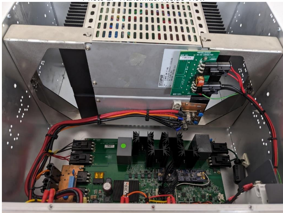
Photo 2: Transmitter Inside View
