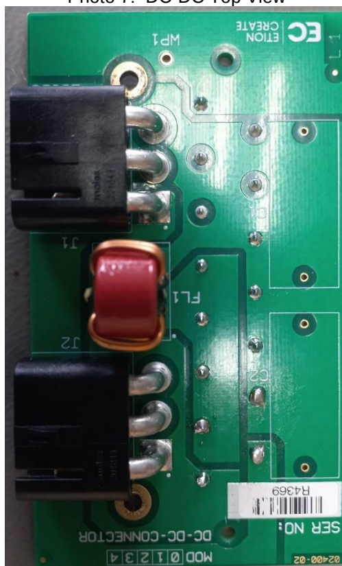
Photo 7: DC-DC Top View
