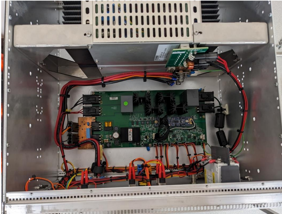
Photo 1: Transmitter Inside View
