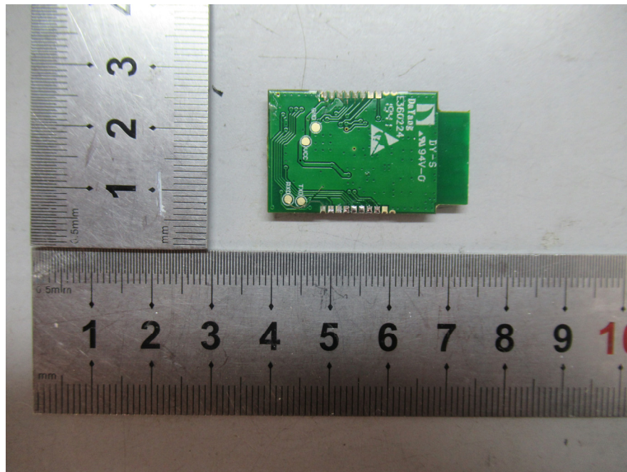
EUT – Bottom View (Model: HM2401)
