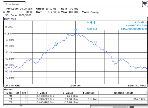
GFSK_Middle
