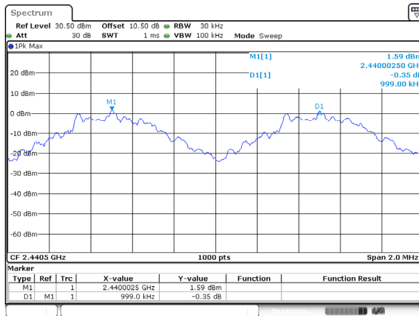
GFSK_Middle
