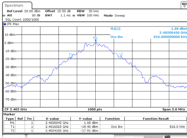
GFSK_Low
