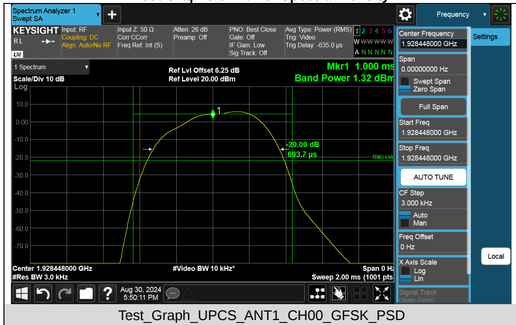
Test Graphs of Power Spectral Density
