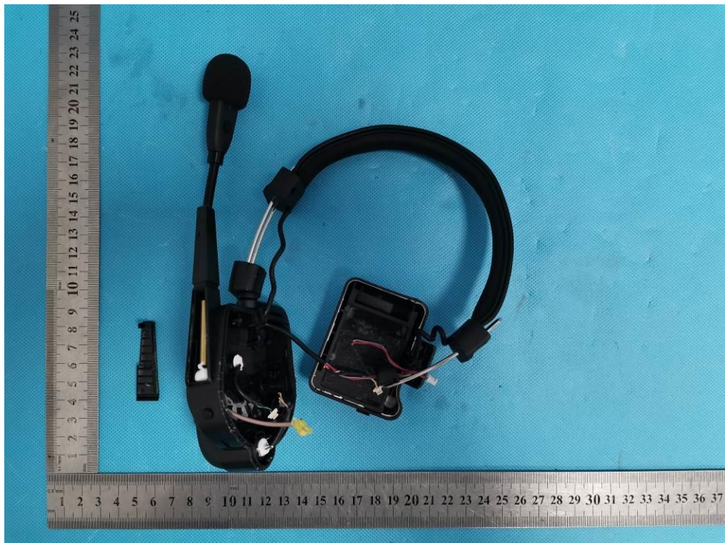
OPEN VIEW OF EUT (FIGURE 6)
