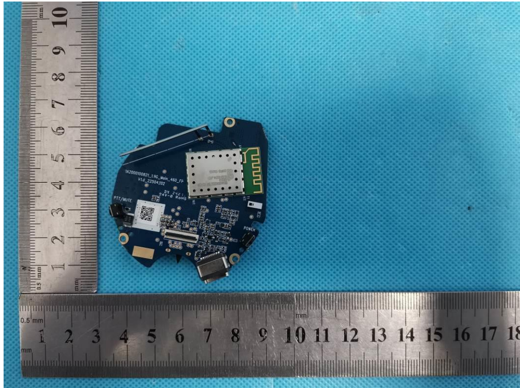
INTERNAL VIEW OF EUT (FIGURE 13)
