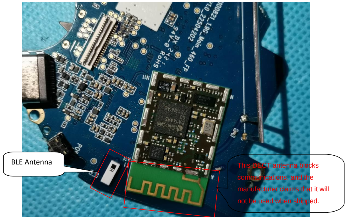
INTERNAL VIEW OF EUT (FIGURE 19)
