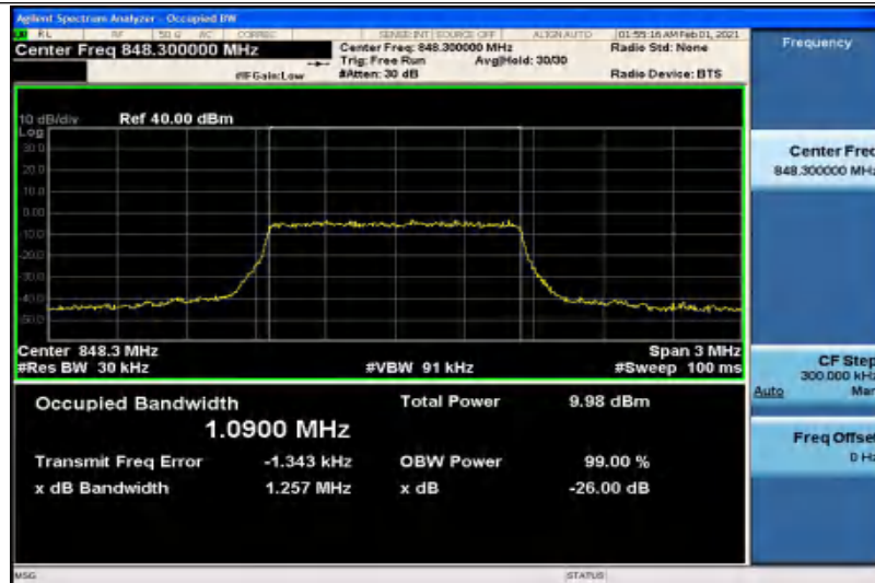
Band5-1.4MHz-16QAM-20407-6RB#0-1.0897
