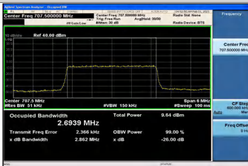
Band12-3MHz-QPSK-23165-15RB#0-2.6943
