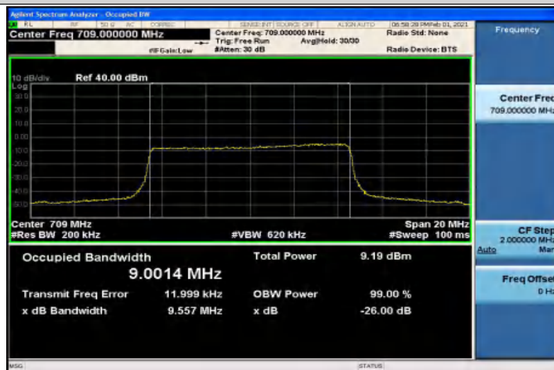
Band17-10MHz-QPSK-23790-50RB#0-8.9600
