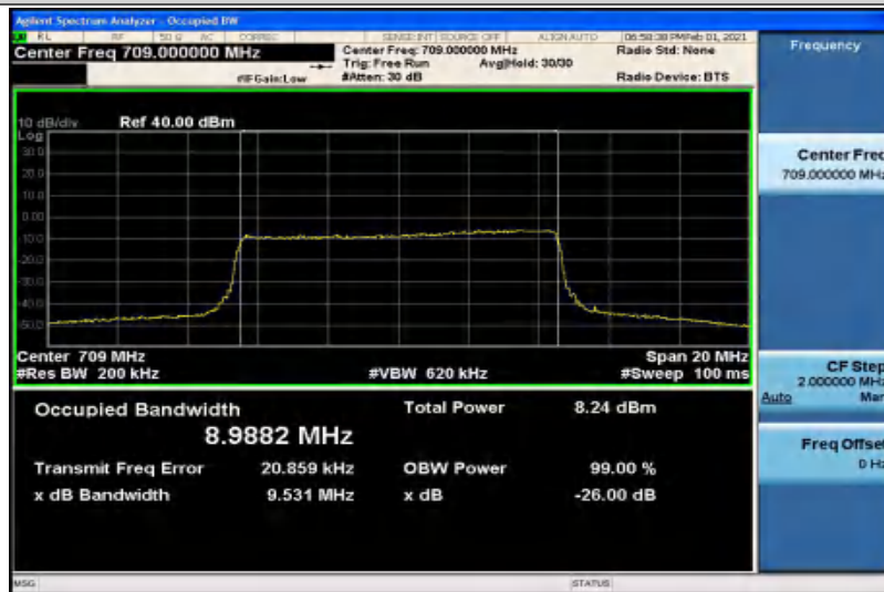
Band17-10MHz-16QAM-23790-50RB#0-8.9708
