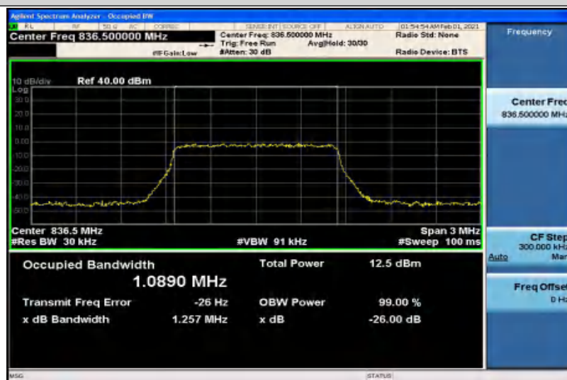
Band5-1.4MHz-QPSK-20643-6RB#0-1.0900
