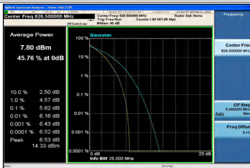
Band5-5MHz-QPSK-20525-1RB#0
