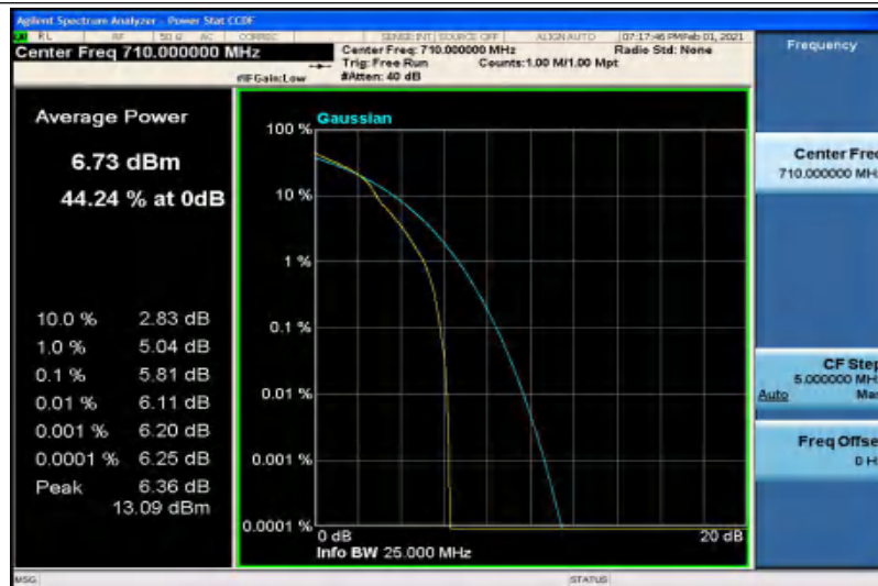
Band17-10MHz-16QAM-23790-50RB#0
