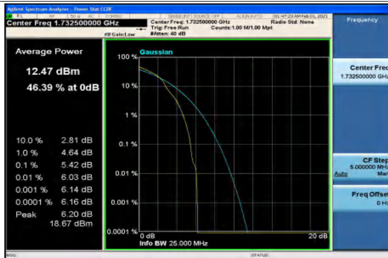
Band4-20MHz-16QAM-20175-100RB#0
