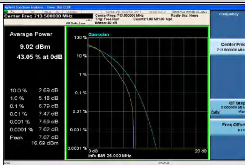
Band12-5MHz-16QAM-23155-25RB#0
