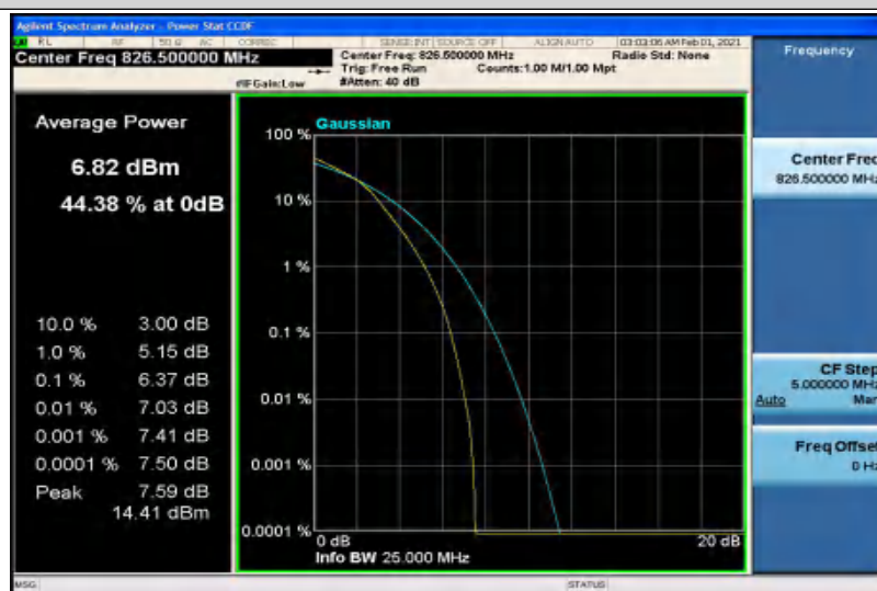
Band5-5MHz-16QAM-20525-1RB#0
