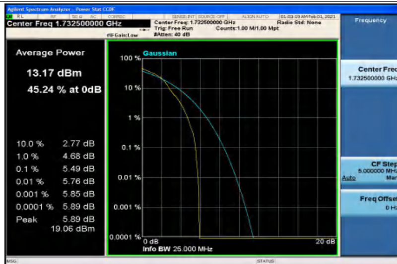
Band4-15MHz-16QAM-20175-75RB#0
