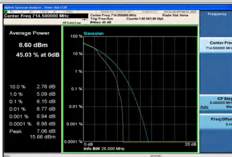
Band12-3MHz-16QAM-23165-15RB#0
