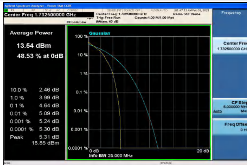
Band4-20MHz-QPSK-20175-100RB#0
