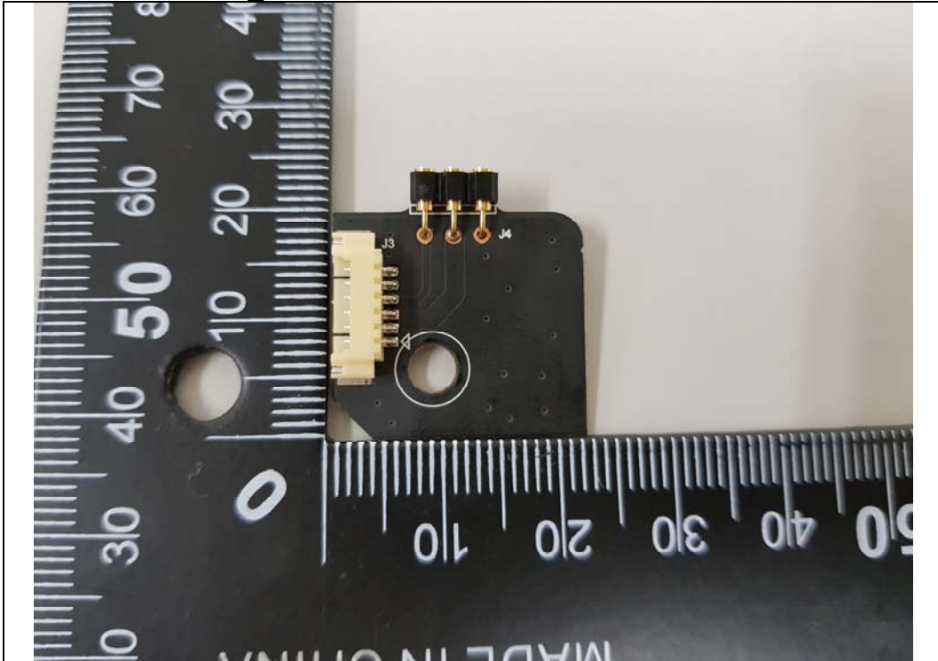
Connector Board Front
