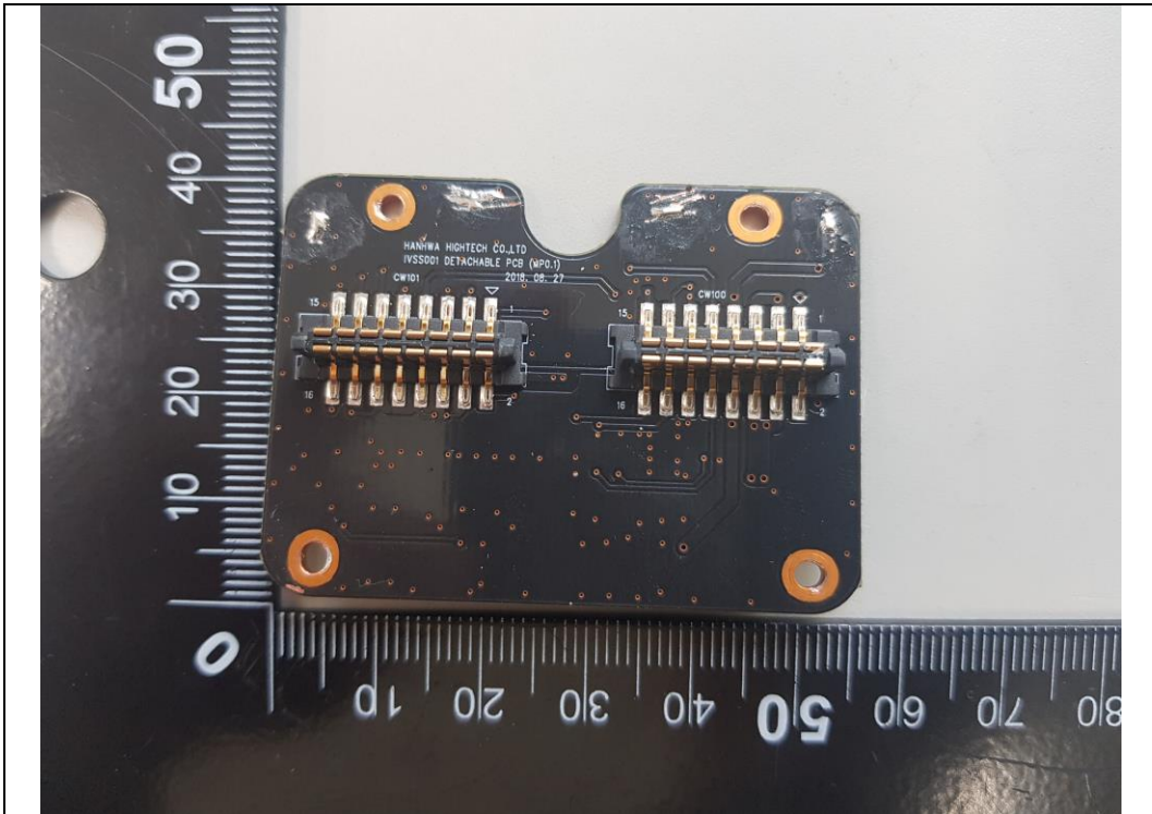
Power Connector_Front
