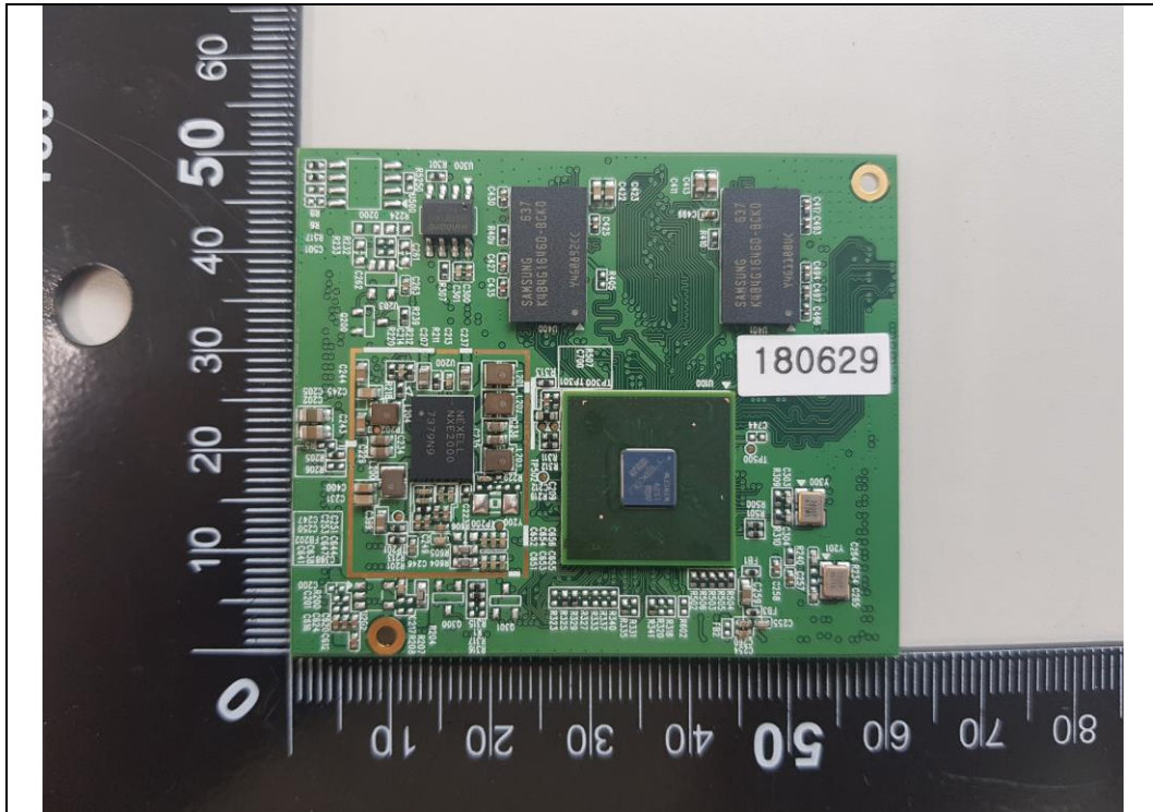
CPU Board_Front
