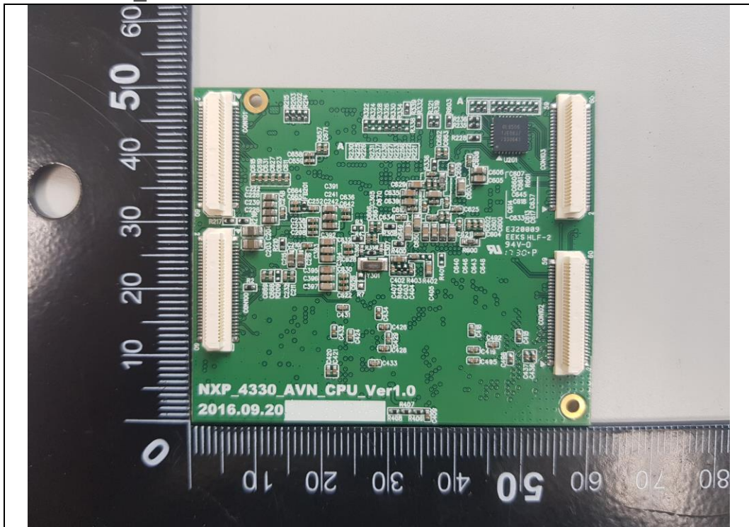
CPU Board_Rear
