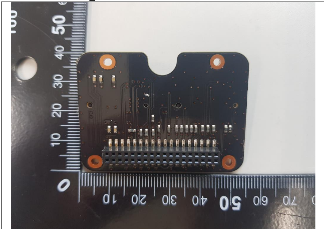
Power Connector_Rear
