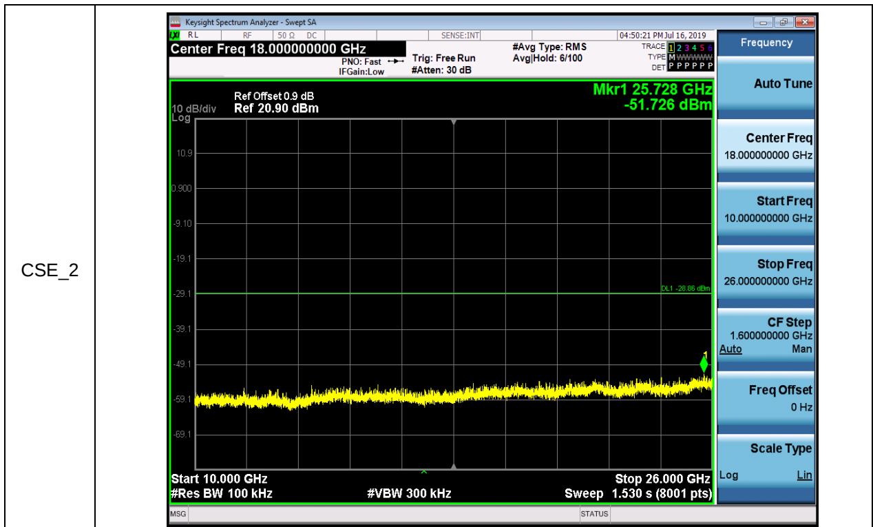
RF Conducted Spurious Emissions_11N40SISO_2452_Ant1
