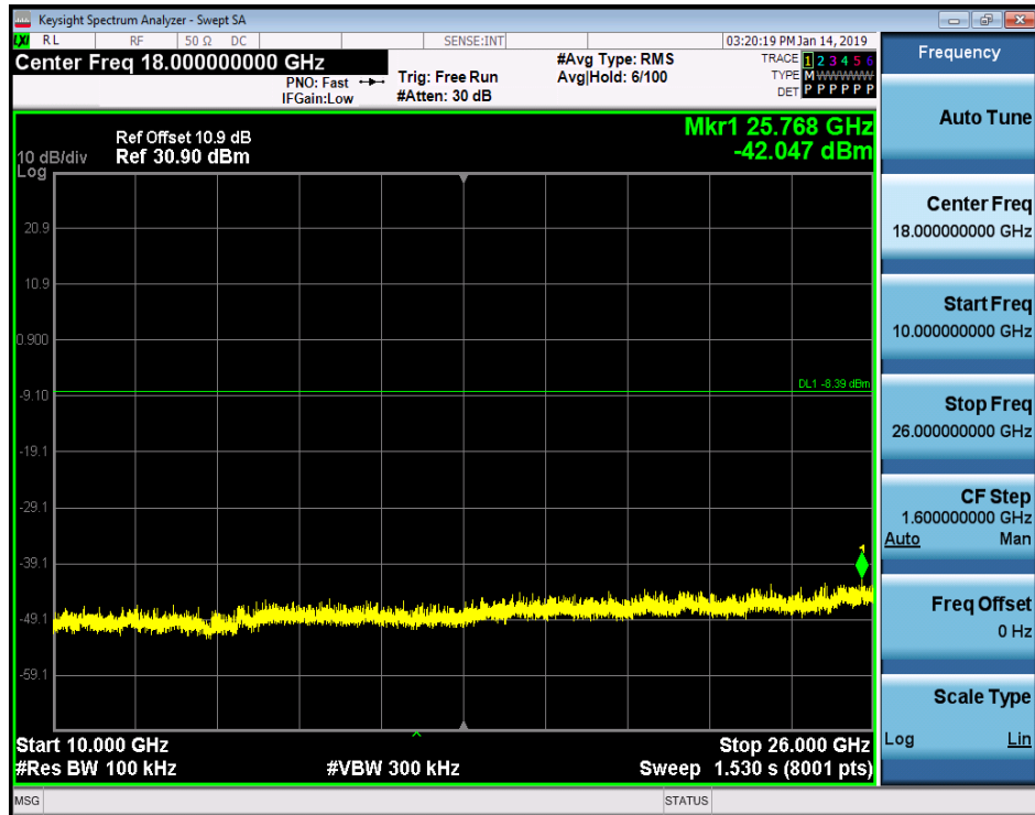
RF Conducted Spurious Emissions_OFDM_2442_Ant2
