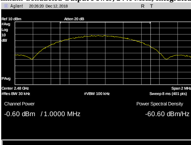
Plot 6. Maximum Conducted Output Power, 2480 MHz, Integrated Band Power
