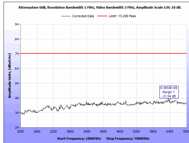
Plot 10. Radiated Emissions, 2402, 1 - 7 GHz, Peak, Horizontal
