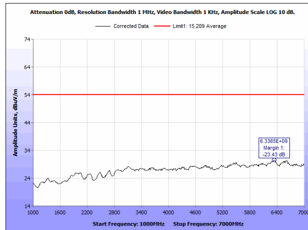
Plot 35. Radiated Emissions, 2480 MHz, 1 - 7 GHz, Average, Vertical
