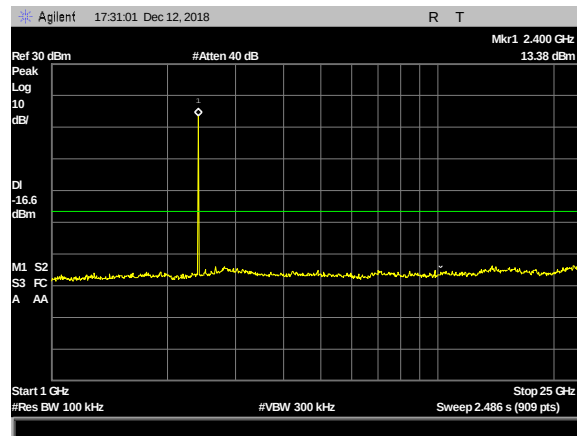
Plot 52. 100 kHz Spurious Emissions, 2440 MHz, 1 –25 GHz
