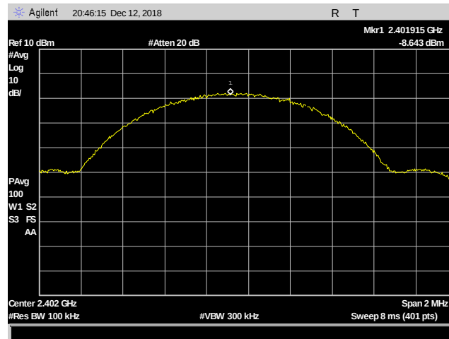
Plot 57. Power Density, 2402 MHz, 100 kHz RBW
