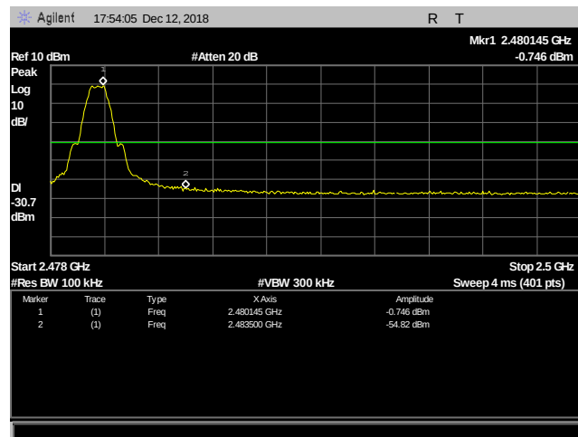
Plot 56. Conducted Bandedge, 2480 MHz
