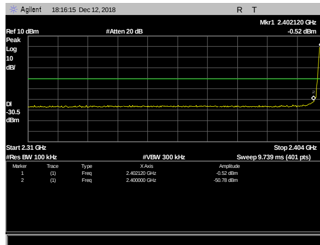
Plot 55. Conducted Bandedge, 2402 MHz
