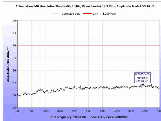
Plot 34. Radiated Emissions, 2480 MHz, 1 - 7 GHz, Peak, Horizontal
