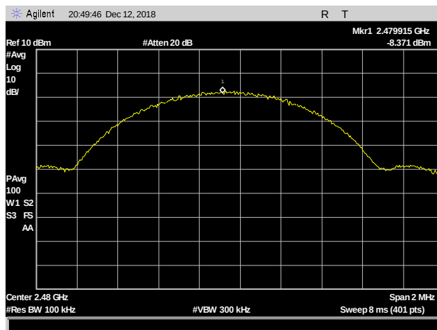
Plot 59. Power Density, 2480 MHz, 100 kHz RBW
