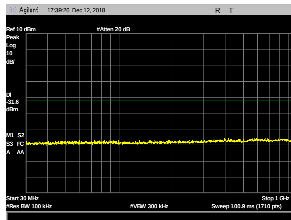
Plot 53. 100 kHz Spurious Emissions, 2480 MHz, 30 – 1000 MHz
