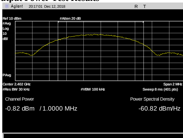
Plot 4. Maximum Conducted Output Power, 2402 MHz, Integrated Band Power
