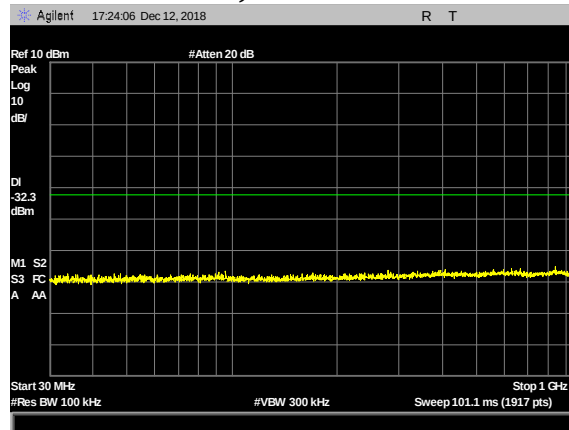
Plot 49. 100 kHz Spurious Emissions, 2402 MHz, 30 – 1000 MHz
