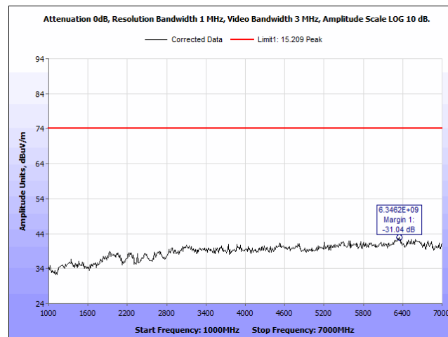
Plot 9. Radiated Emissions, 2402, 1 - 7 GHz, Peak, Vertical
