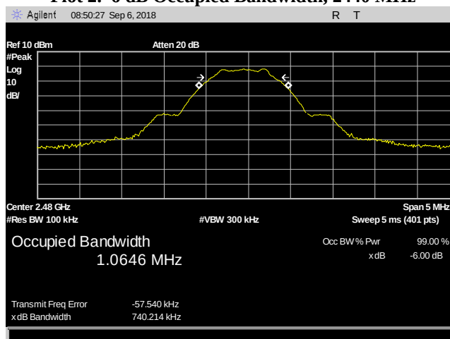
Plot 3. 6 dB Occupied Bandwidth, 2480 MHz
