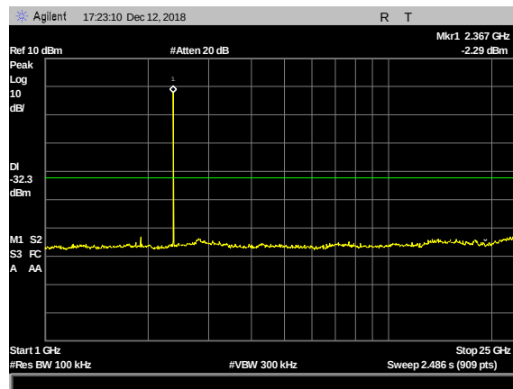
Plot 50. 100 kHz Spurious Emissions, 2402 MHz, 1 – 25 GHz
