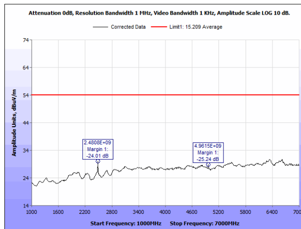
Plot 36. Radiated Emissions 2480 MHz, 1 - 7 GHz, Average, Horizontal
