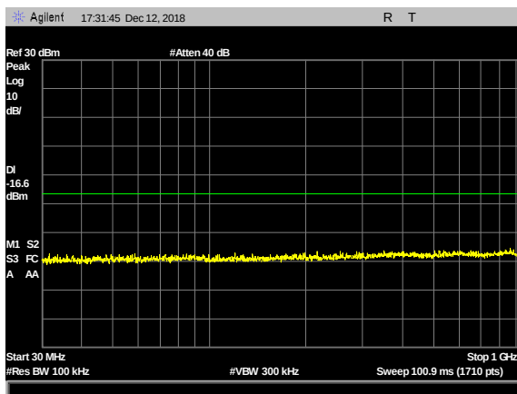
Plot 51. 100 kHz Spurious Emissions, 2440 MHz, 30 – 1000 MHz
