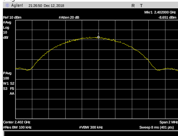
Plot 57. Power Density, 2402 MHz, 100 kHz RBW
