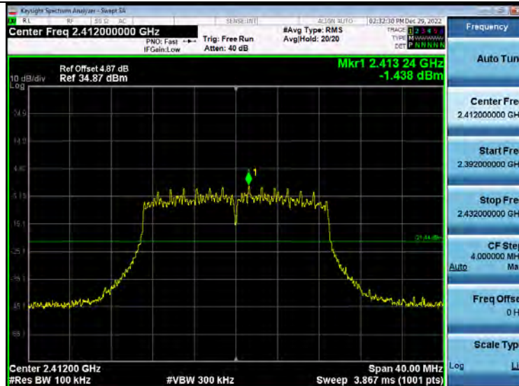
2_Bandedge_2_4GWiFi_NVNT_ANT2_802_11n(HT20)_2412
