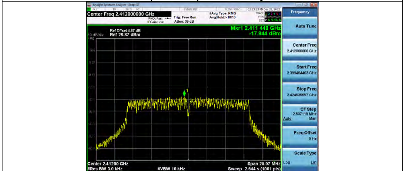
Power_Spectral_Density_2_4GWiFi_802_11g_2412
