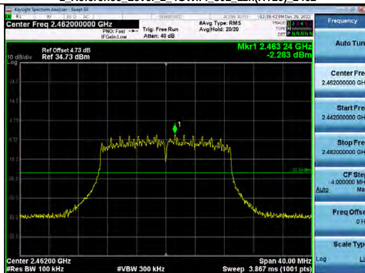
2_Bandedge_2_4GWiFi_NVNT_ANT2_802_11n(HT20)_2462
