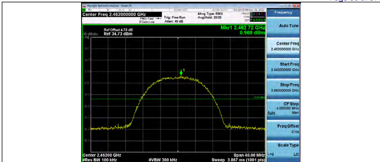
2_Bandedge_2_4GWiFi_NVNT_ANT2_802_11b_2462
