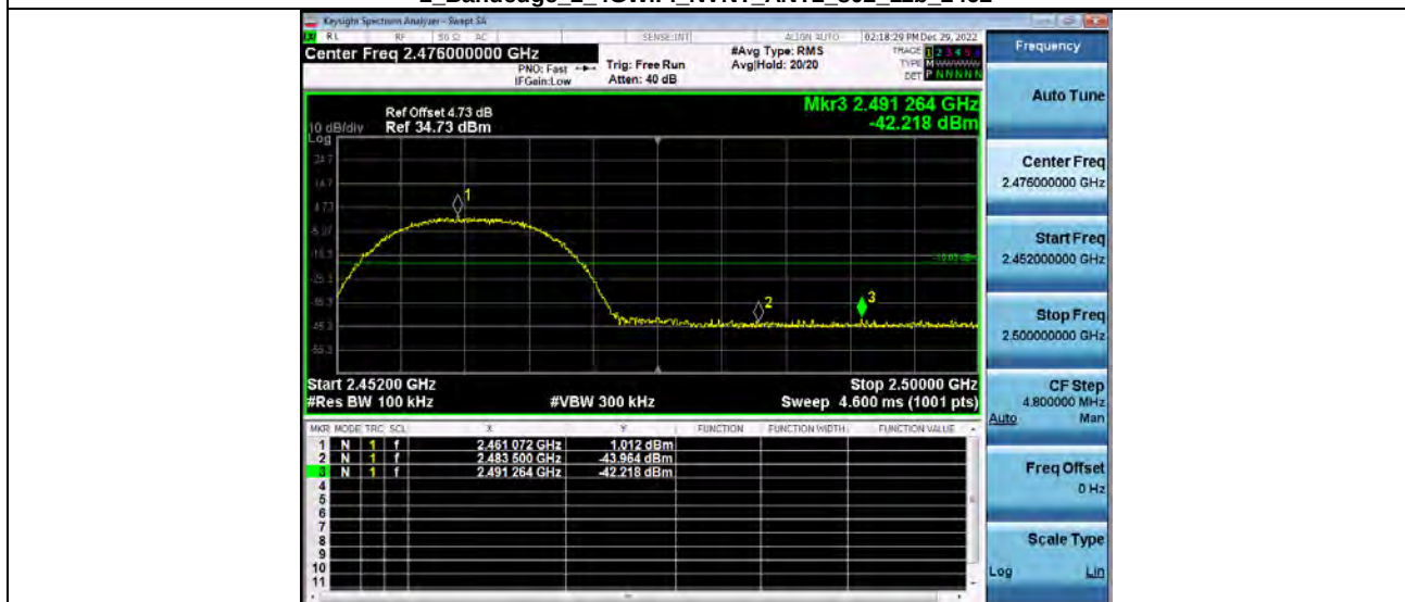
2_Bandedge_2_4GWiFi_NVNT_ANT2_802_11b_2462
