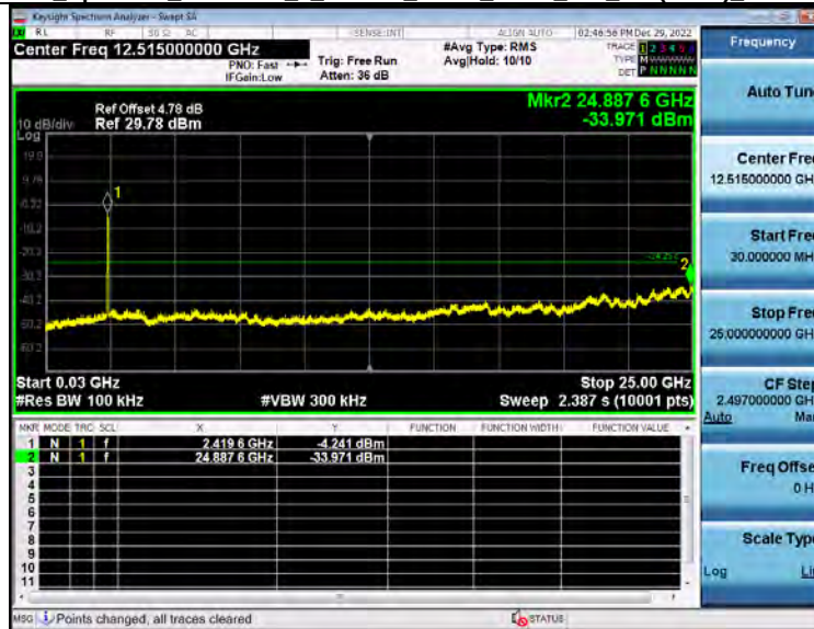
2_Spurious Emission 2_4GWiFi_NVNT_ANT2_802_11n(HT40)_2422
