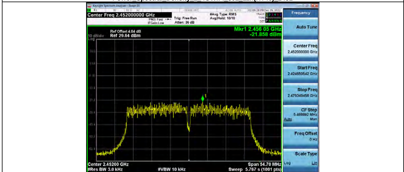
Power_Spectral_Density_2_4GWiFi_802_11n(HT40)_2452
