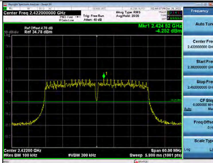
2_Spurious Emission 2_4GWiFi_NVNT_ANT2_802_11n(HT40)_2422
