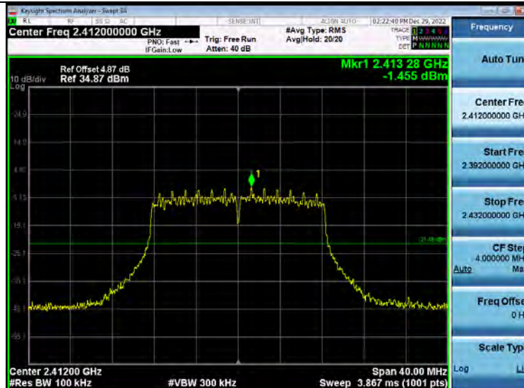
2_Spurious Emission 2_4GWiFi_NVNT_ANT2_802_11g_2412
