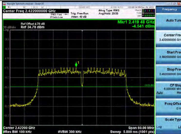
2_Bandedge_2_4GWiFi_NVNT_ANT1_802_11n(HT40)_2422
