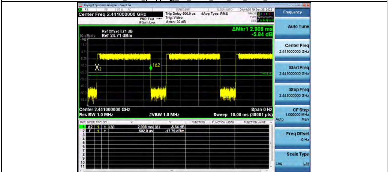
Dwell Time (Hopping) BT 3-DH5 2441 One Burst Time
