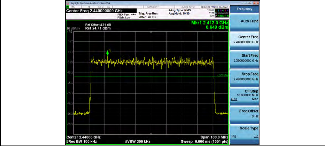
2_Band_Edge_(Hopping)_BT_2-DH5_Hopping
