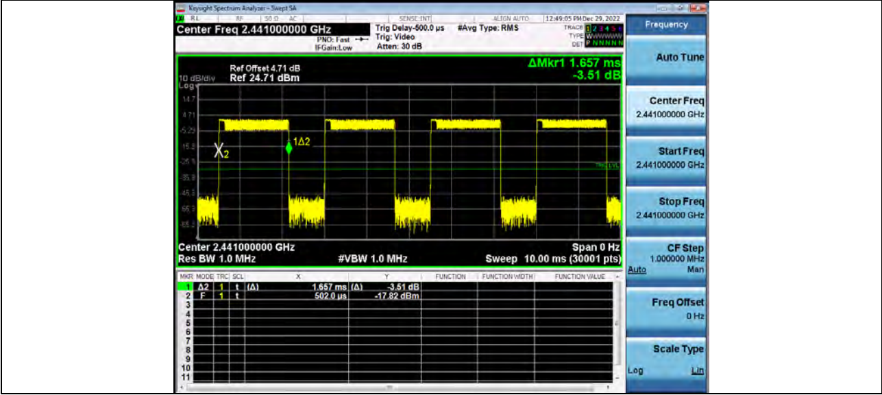
Dwell Time (Hopping) BT 2-DH3_2441_One_Burst_Time
