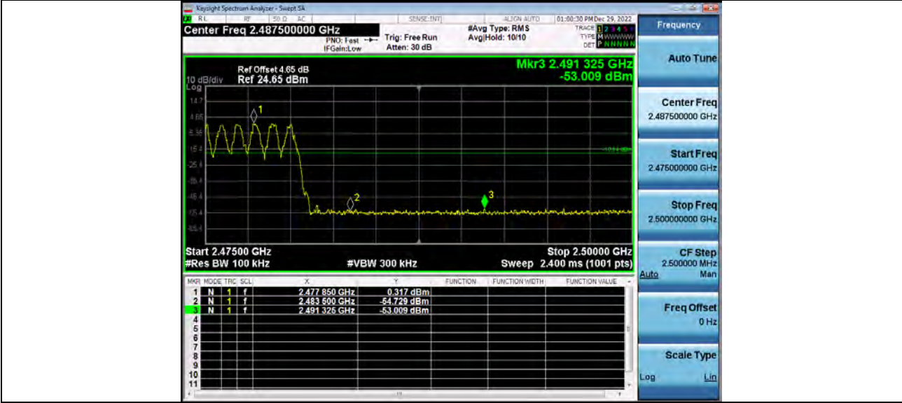
2_Band_Edge (Hopping) BT 1-DH5 Hopping
