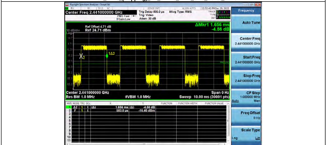
Dwell Time (Hopping) BT 3-DH1 2441 One Burst Time
