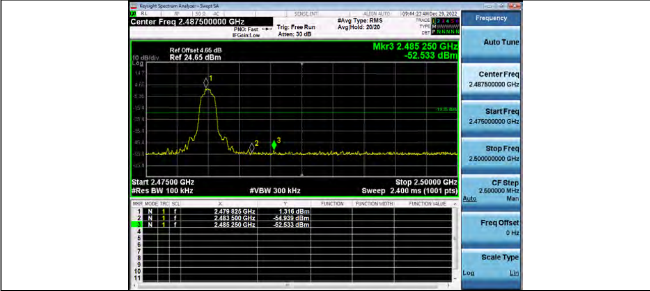
2_Bandedge_BT_2-DH5_2480
