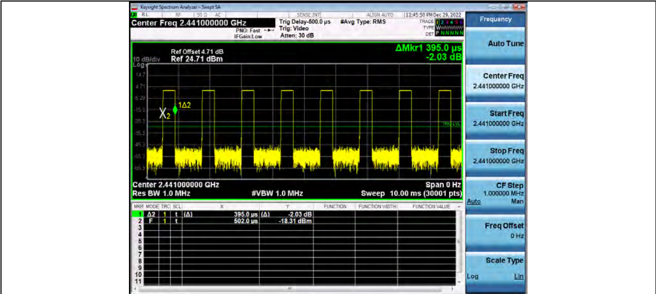
Dwell Time (Hopping) BT 2-DH5_2441_One_Burst_Time
