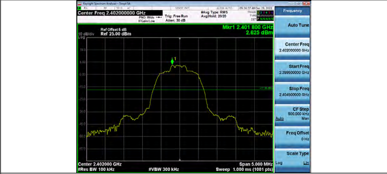
2_Bandedge BT 2-DH5 2402
