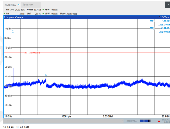
11G_Ant2_2437_0~Reference
