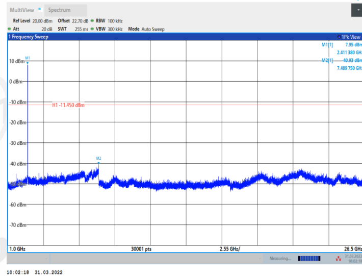
11B_Ant2_2412_0~Reference
