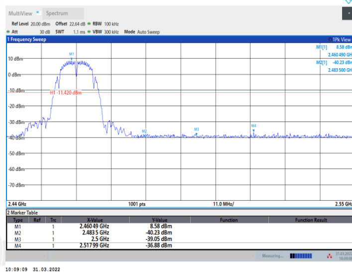
11B_Ant2_High_2462
