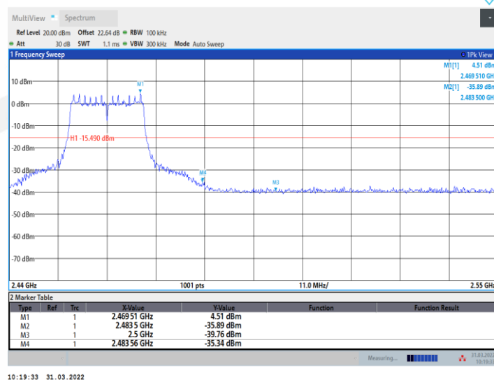
11G_Ant2_High_2462
