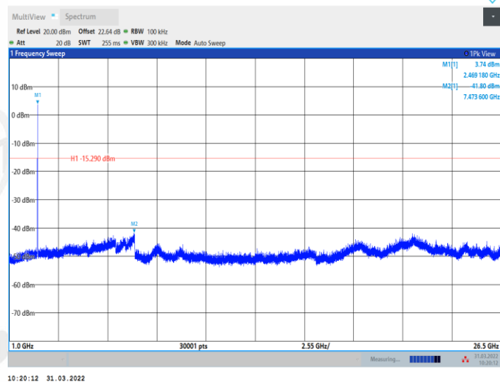
11G_Ant2_2462_0~Reference
