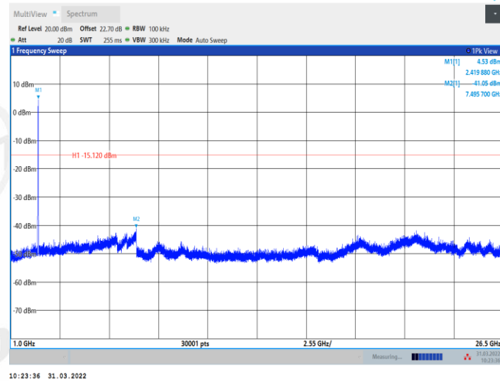
11G_Ant2_2412_0~Reference
