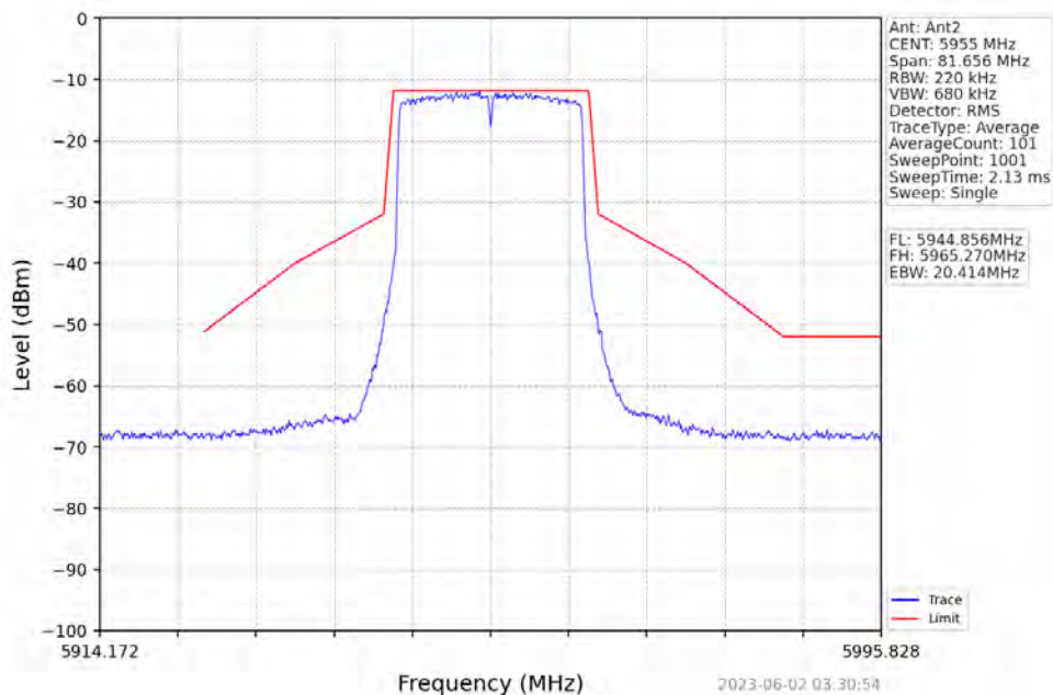
802.11ax(HEW20)_LCH_5955MHz_SU_Ant2_NTNV
