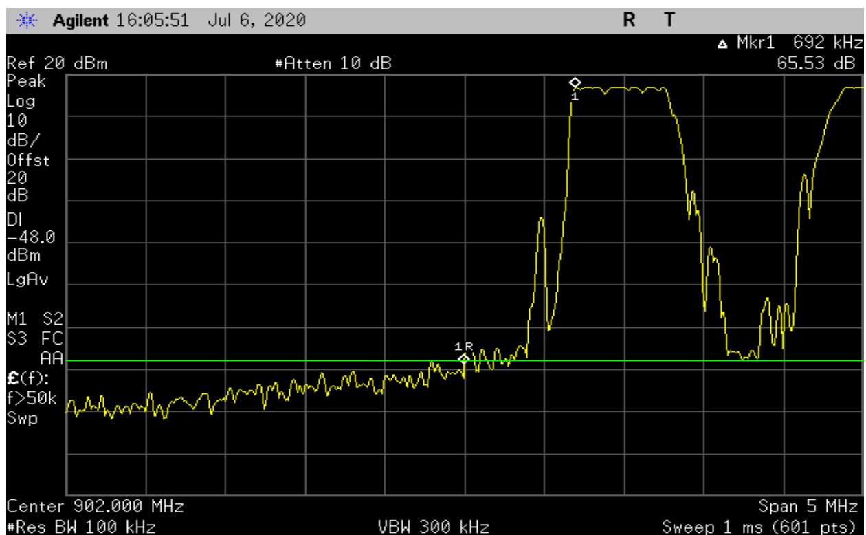
Plot 32 - Band Edge – Low Channel (500kHz BW) – Hopping On
