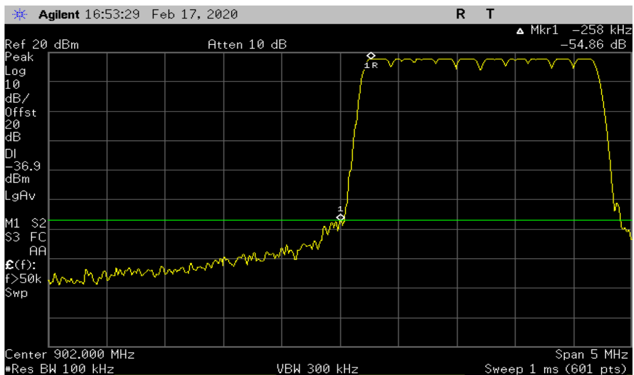
Plot 30 - Band Edge – Low Channel (500kHz BW) – Hopping Off
