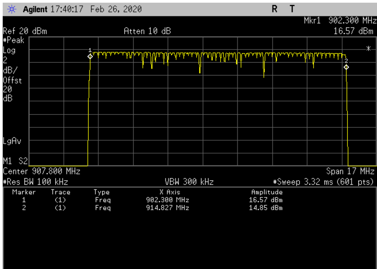
Plot 44 – Number of Frequency Hops – 902.3MHz to 914.9MHz (72Hops)
