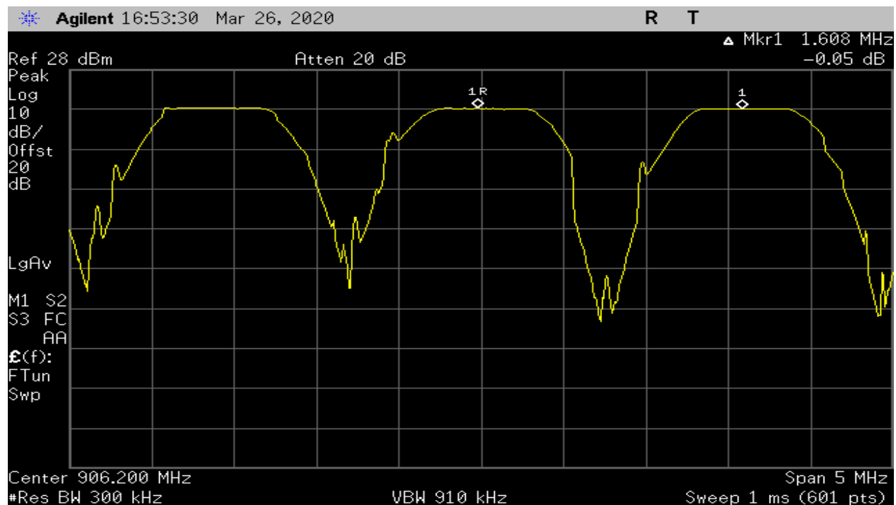
Plot 46 – Carrier Frequency Separation (Using Delta Marker Method) – 500kHz BW
