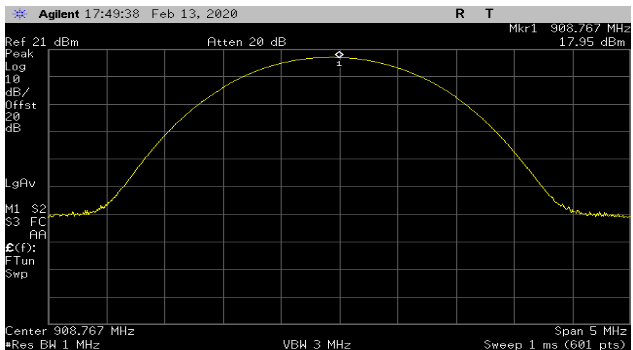
Plot 14 – Output Power – Highest Channel (500kHz)
