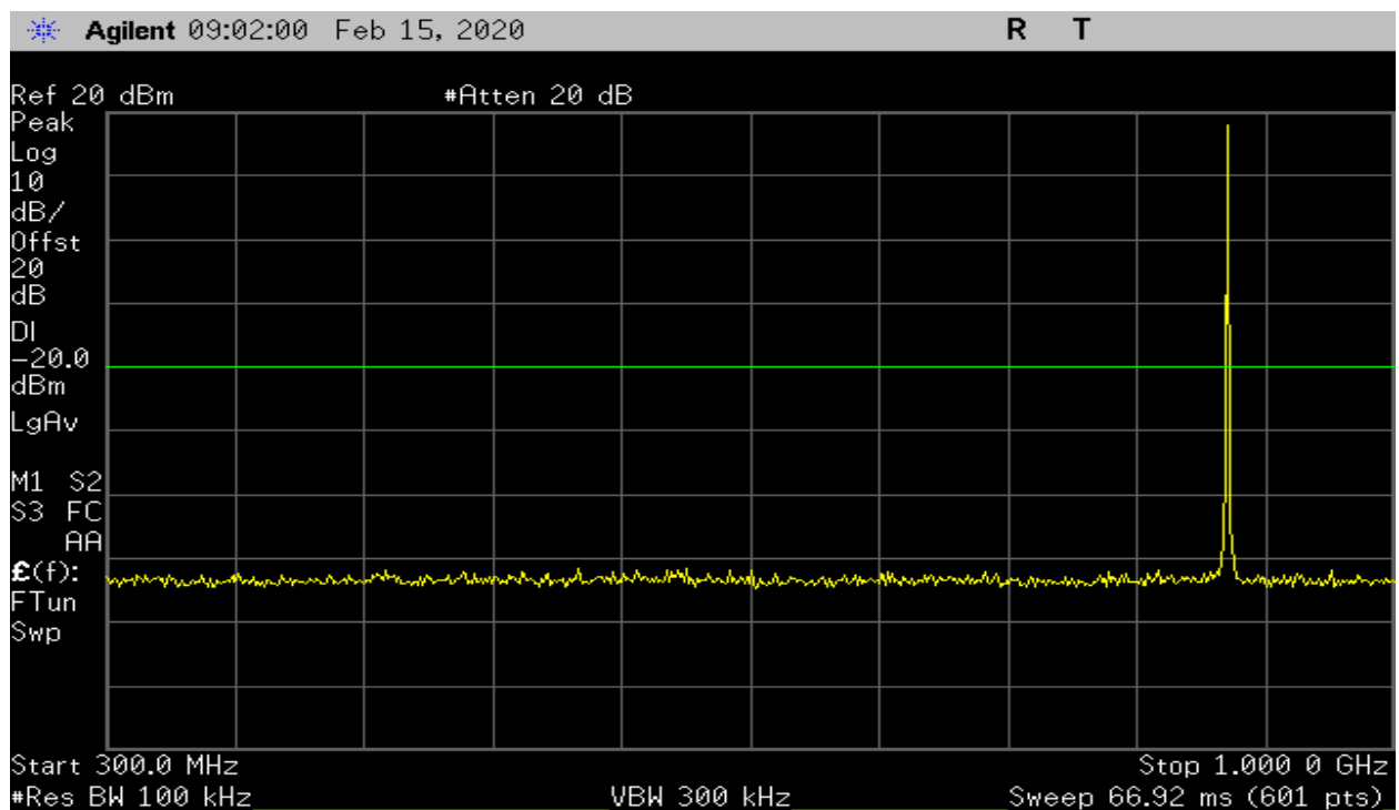
Plot 24 – High Band – 300MHz to 1GHz (Channel 71)
