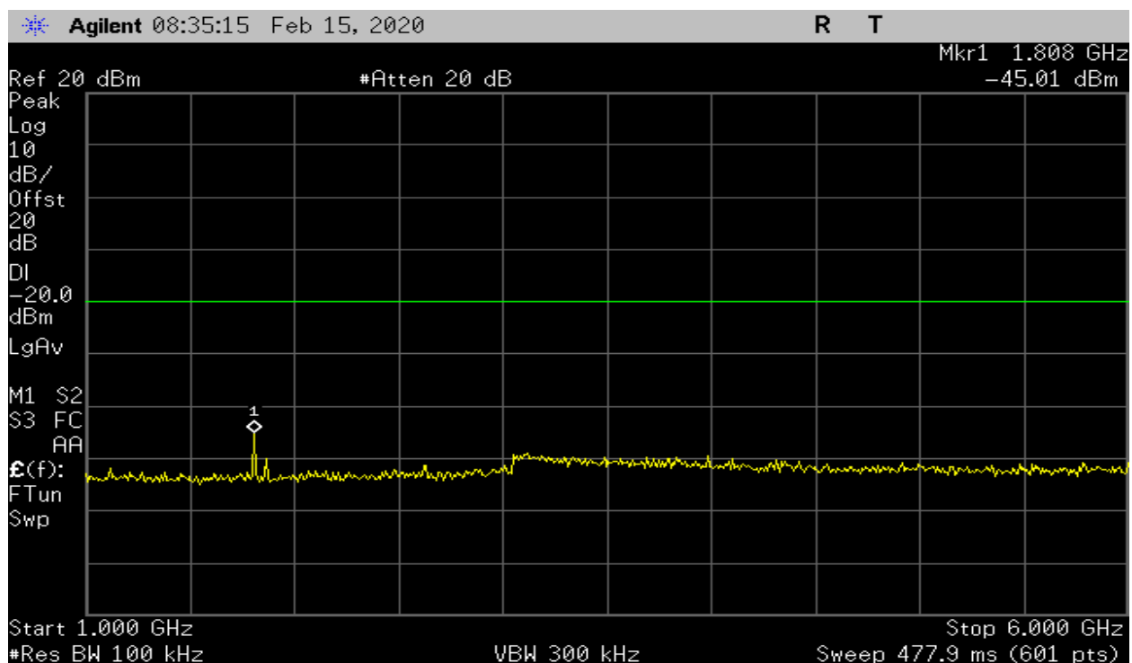
Plot 17 – Low Band – 1GHz to 6GHz
