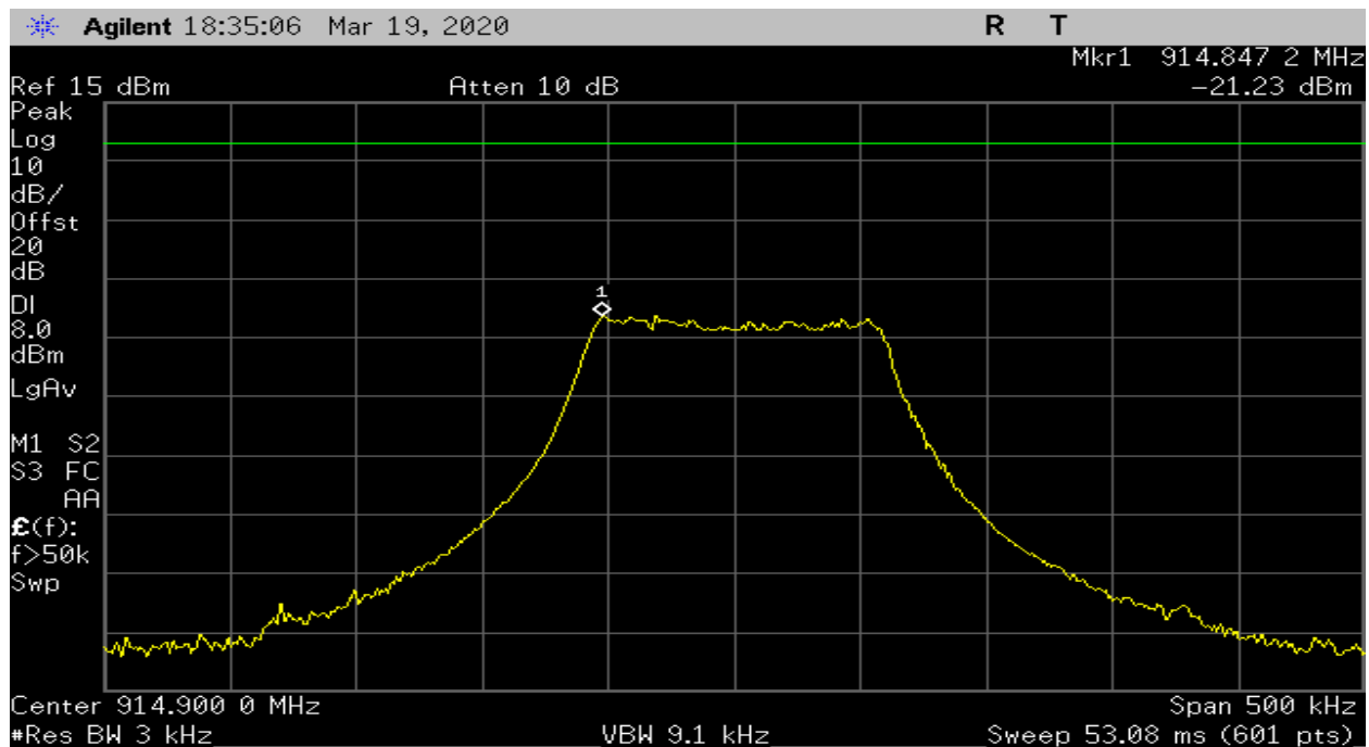
Plot 39 – Power Spectral Density – Highest Channel – 500kHz BW
