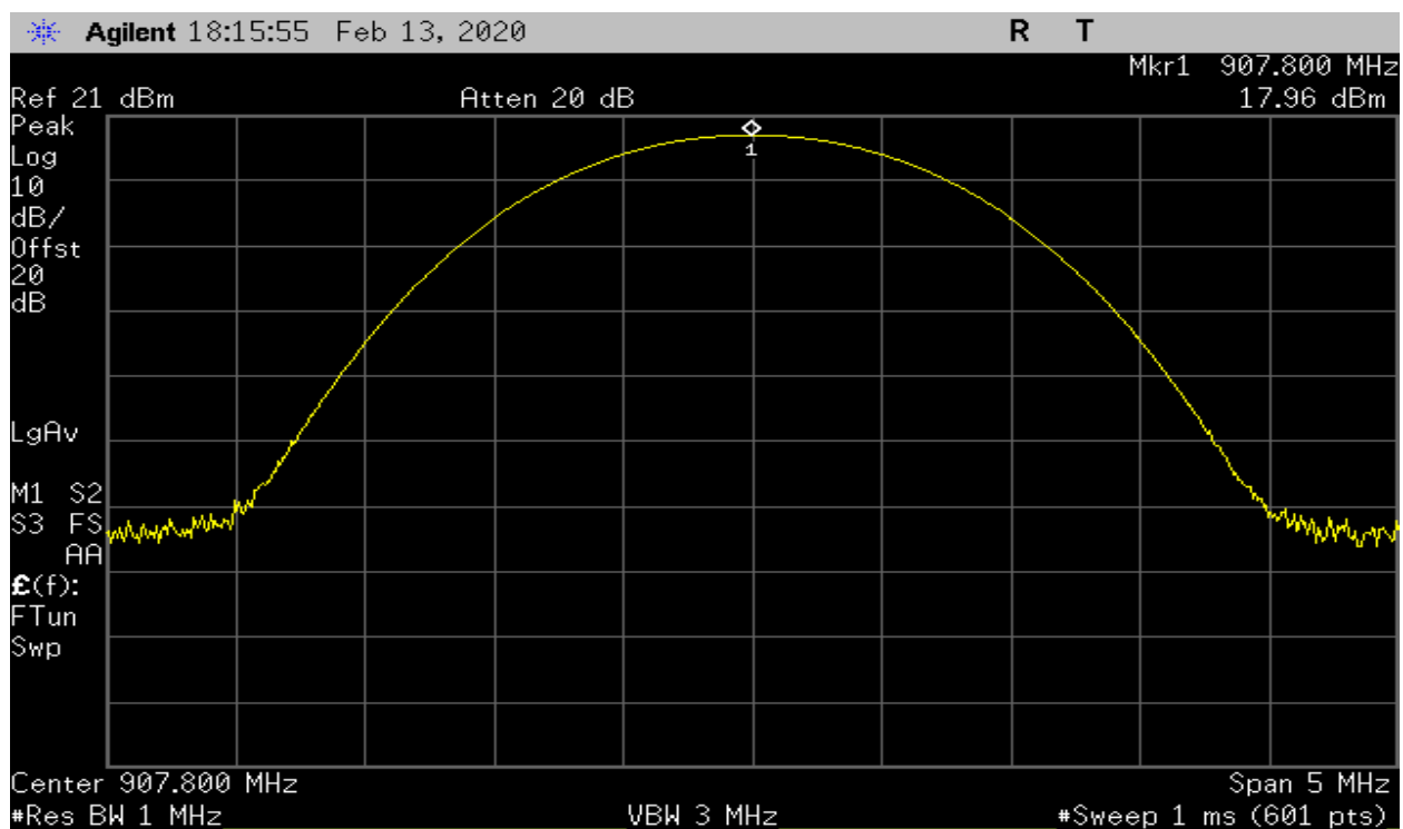
Plot 13 – Output Power – Middle Channel (500kHz BW)
