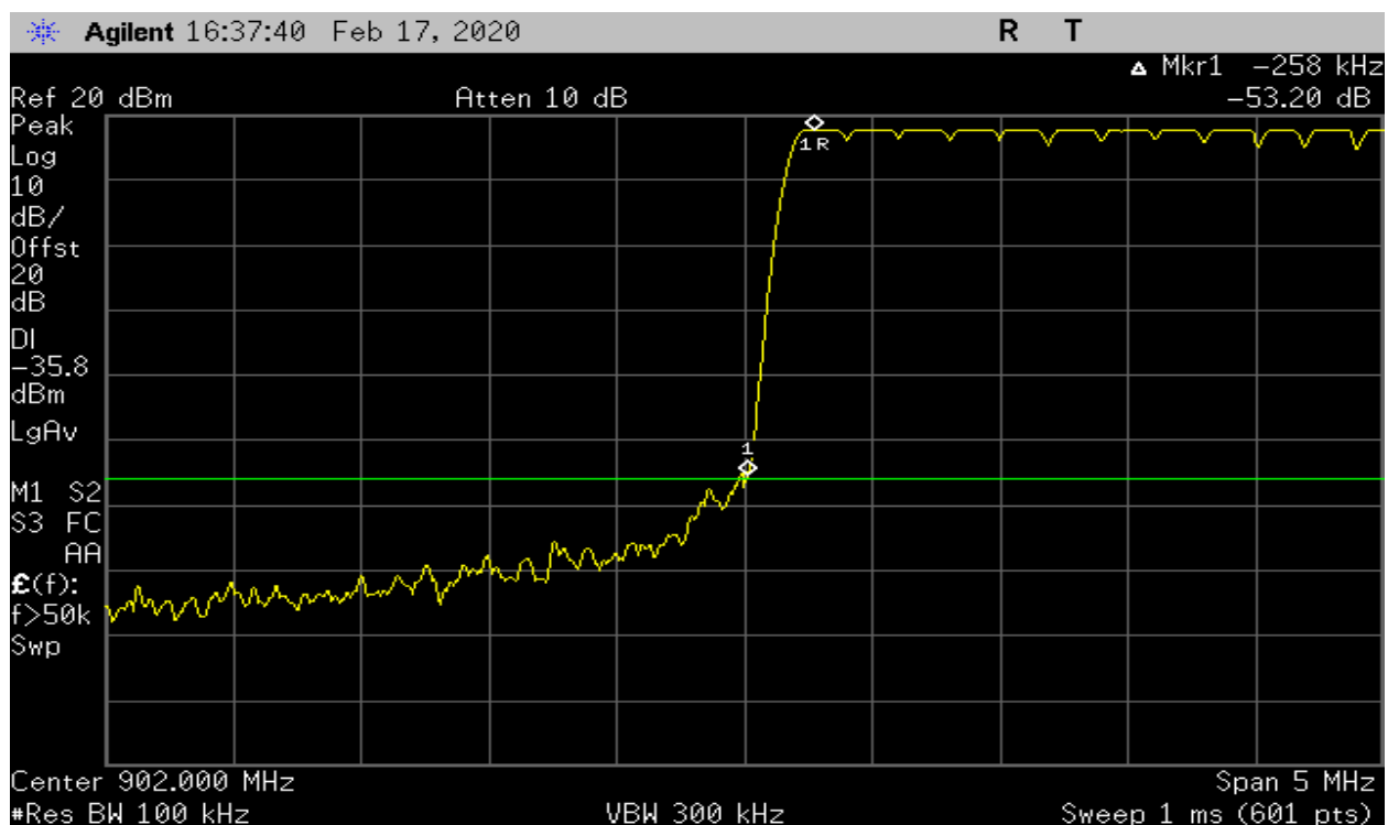
Plot 27 - Band Edge – Low Channel (125kHz BW) – Hopping Off
