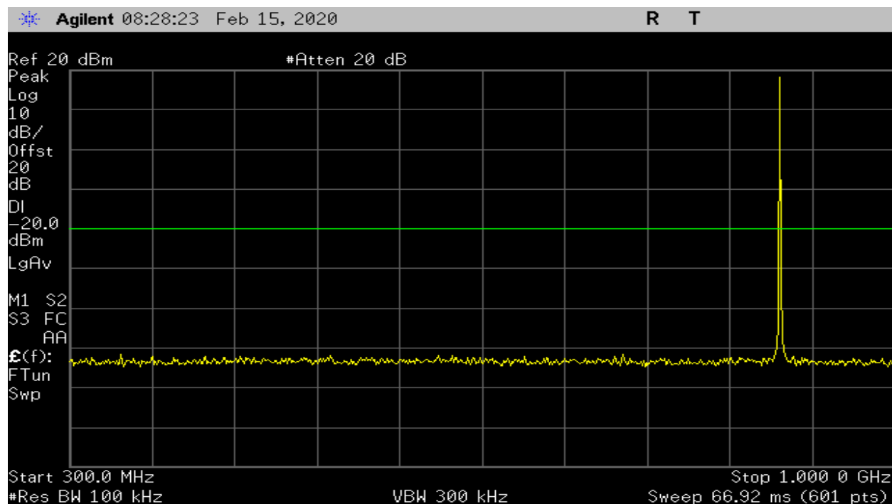
Plot 16 – Low Band – 300MHz to 1GHz (Channel 0)
