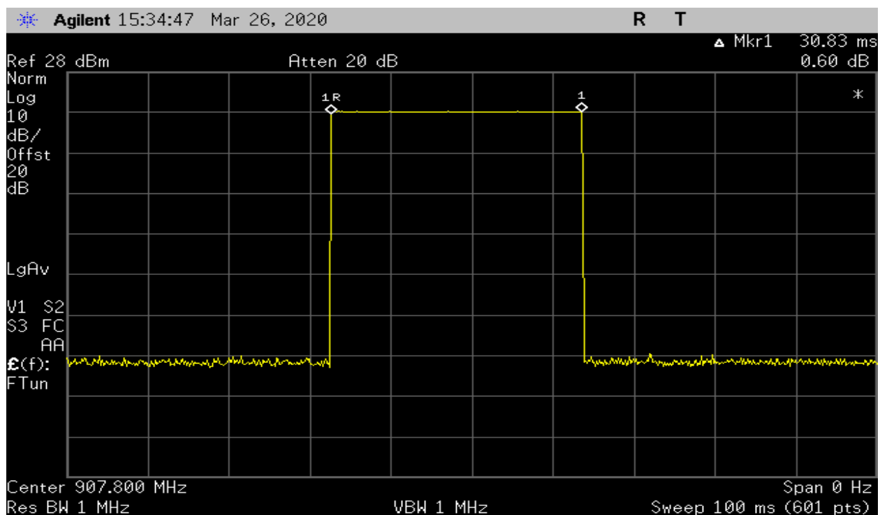
Plot 42 – Dwell Time (500kHz BW)
