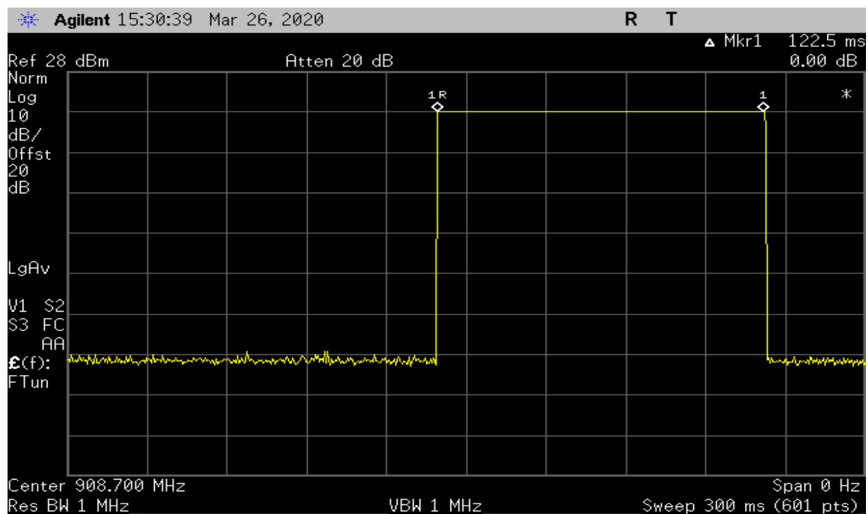
Plot 40 – Dwell Time (125kHz BW)
