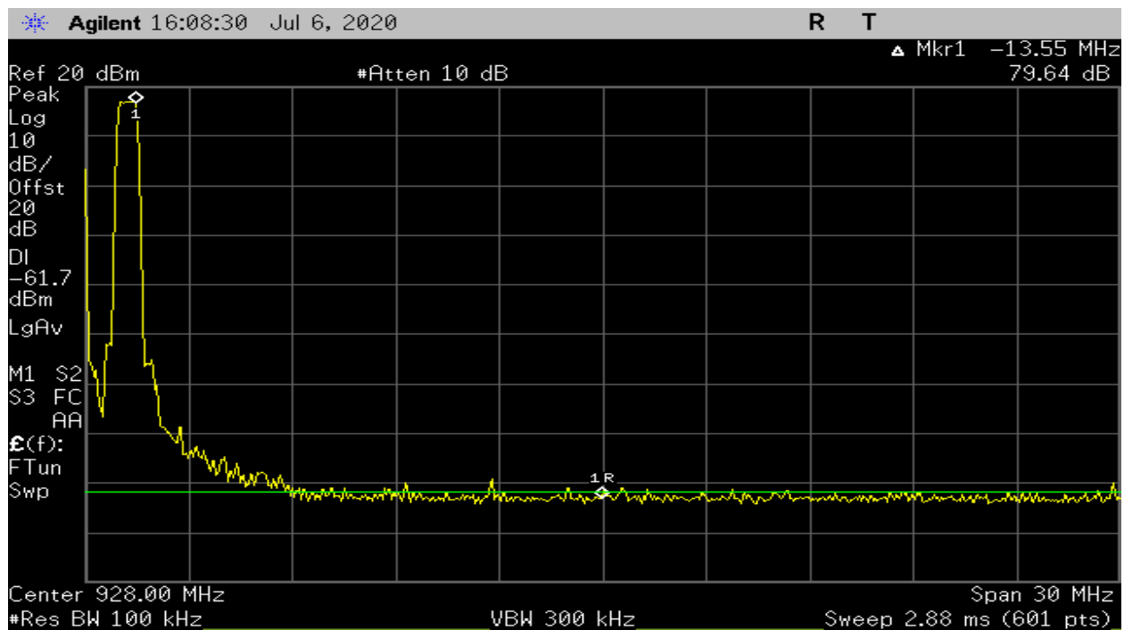
Plot 33 - Band Edge – High Channel (500 kHz BW) – Hopping On
