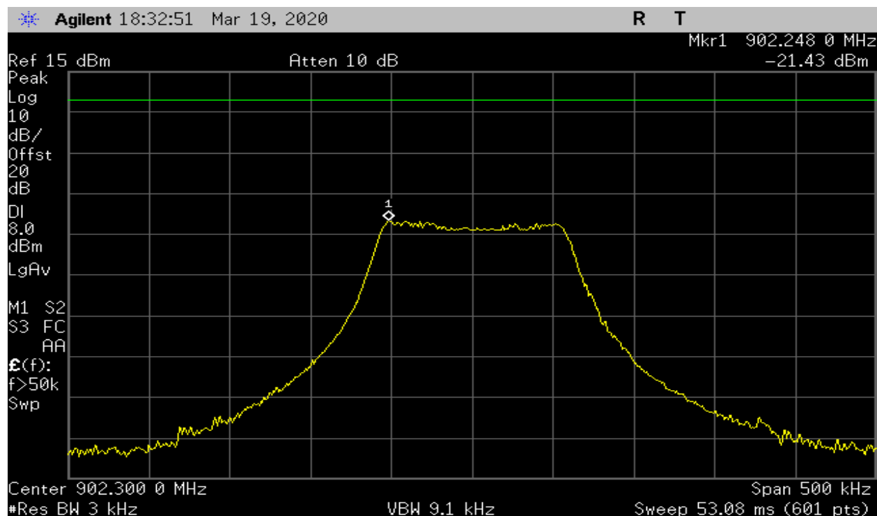
Plot 37 – Power Spectral Density – Lowest Channel – 500kHz BW
