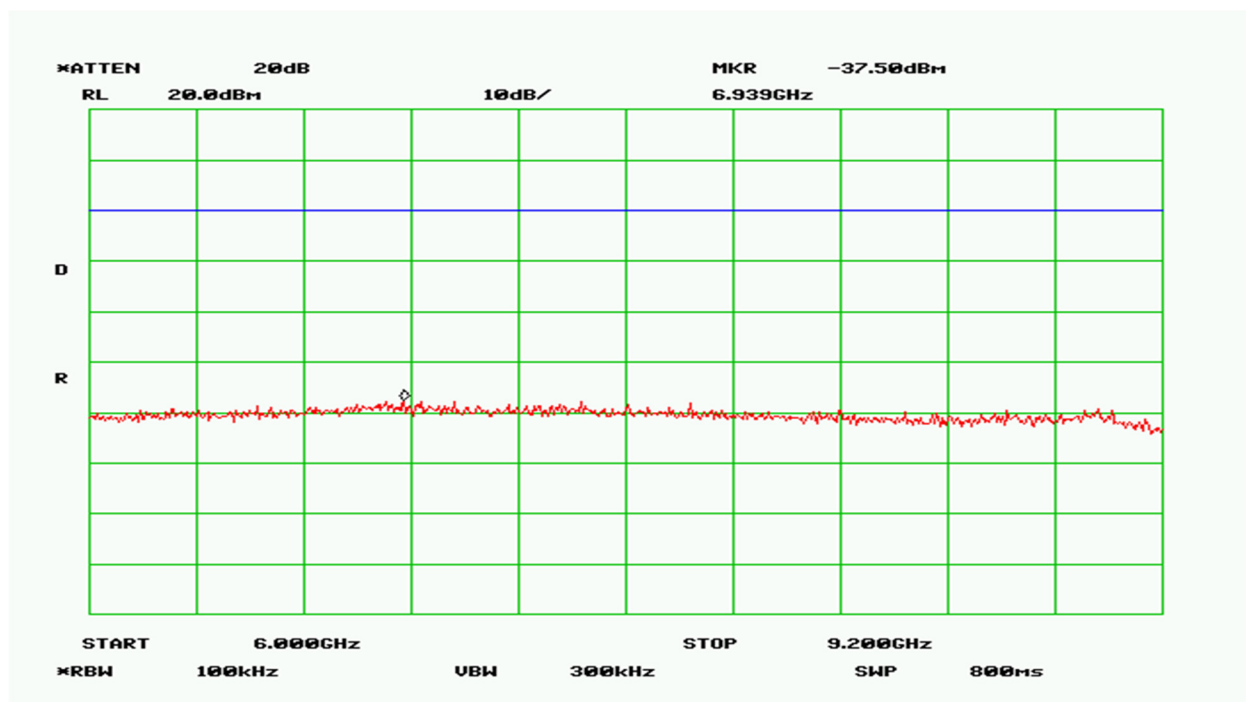
Plot 18 – Low Band – 6GHz to 9.2GHz (Channel 0)
