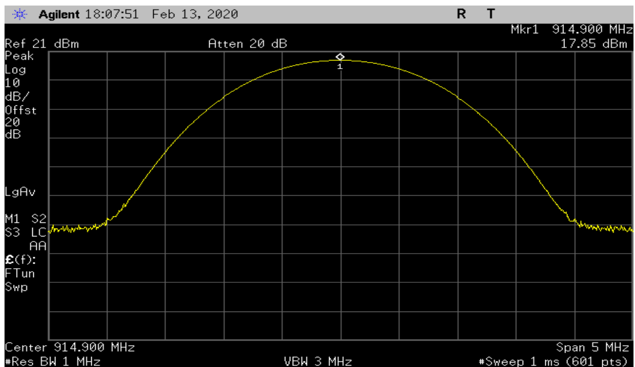
Plot 11 – Output Power – Highest Channel
