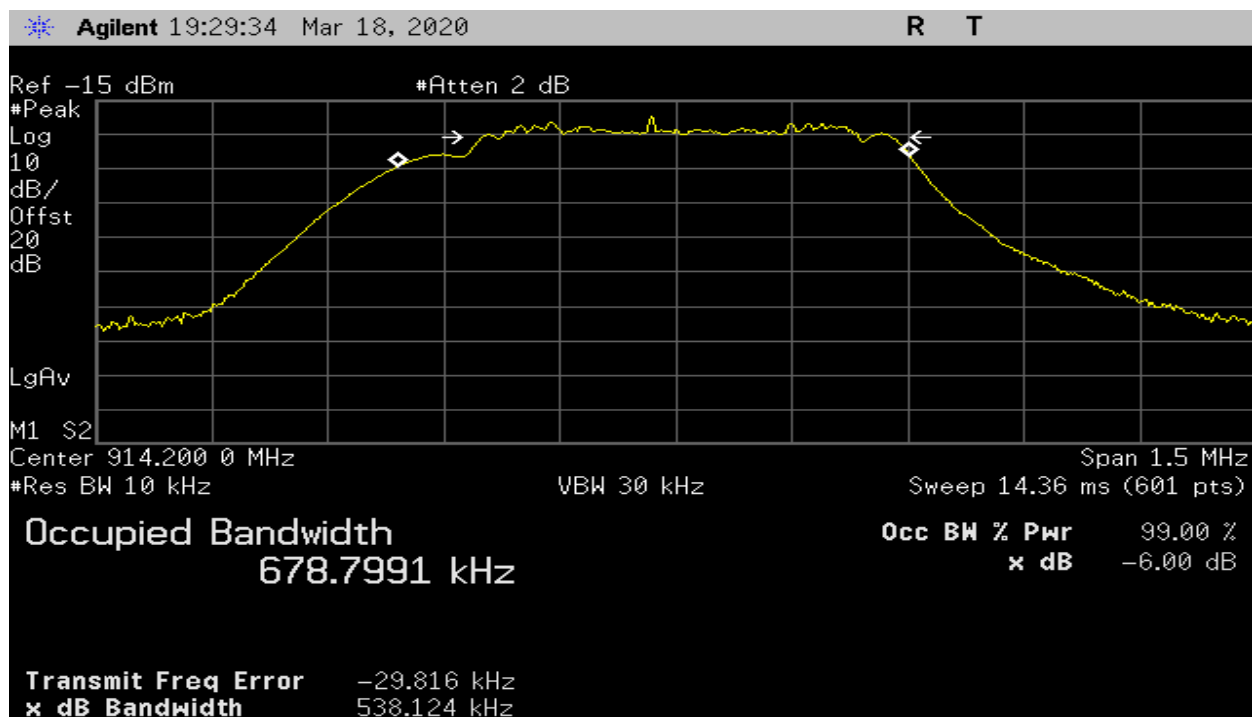
Plot 8 – Highest Channel – 6dB BW (500 kHz BW)
