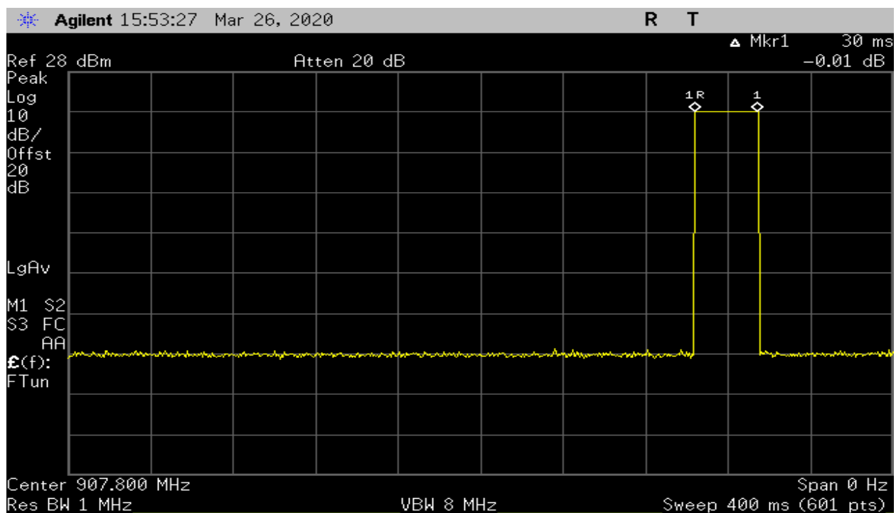
Plot 43 – # of Hops in 0.4 second period – 500kHz BW
