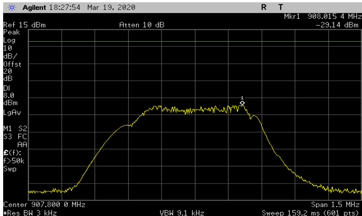
Plot 35 – Power Spectral Density – Middle Channel – 125kHz BW
