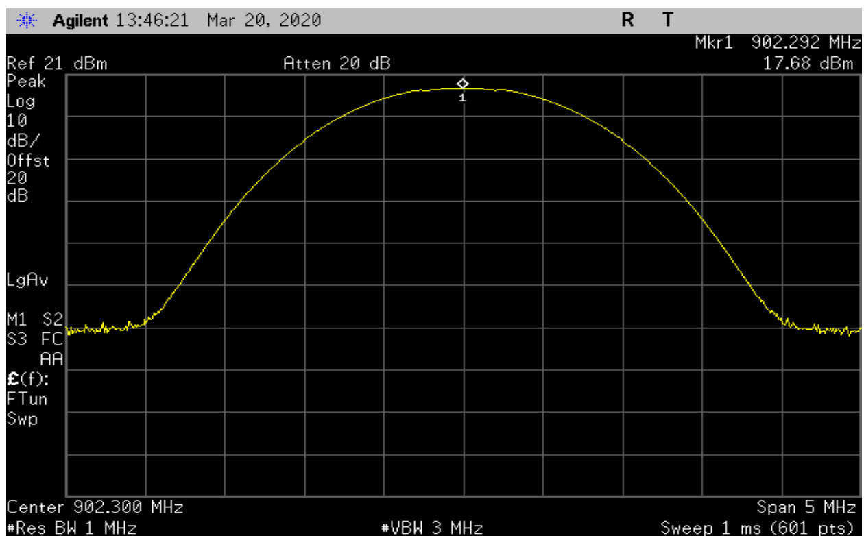
Plot 9 – Output Power – Lowest Channel
