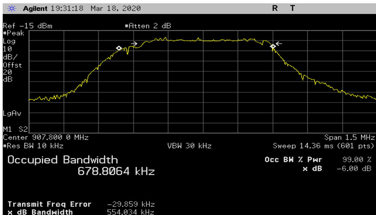
Plot 7 – Middle Channel – 6dB BW (500kHz BW)
