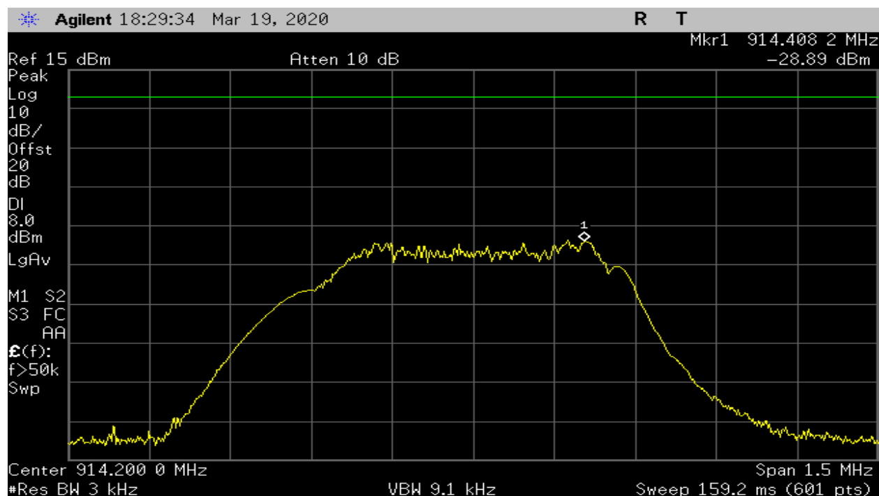
Plot 36 – Power Spectral Density – Highest Channel – 125kHz BW
