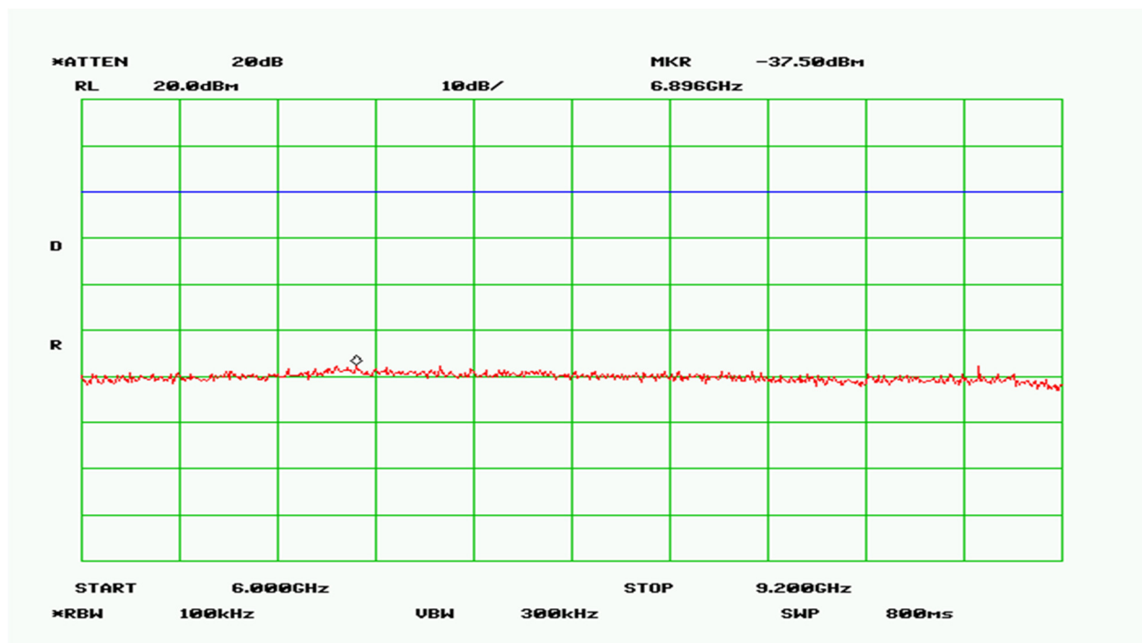
Plot 26 – High Band – 6GHz to 9.2GHz (Channel 71)
