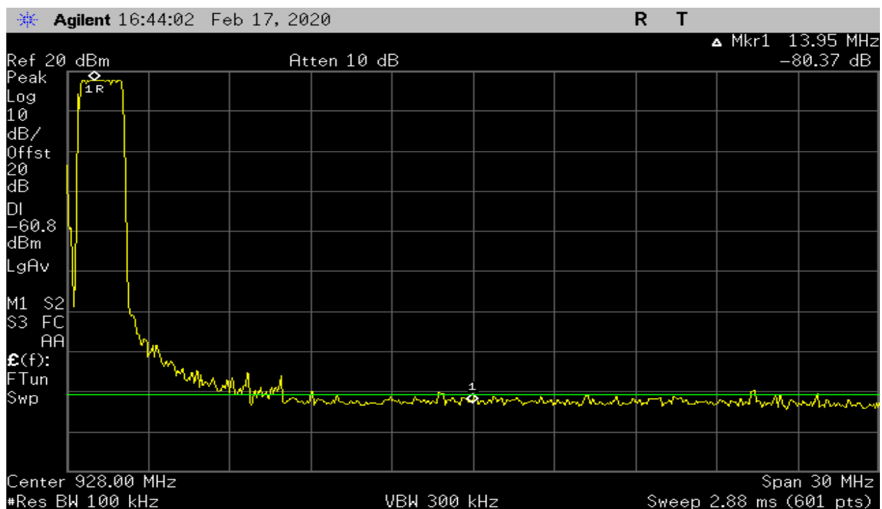
Plot 28 – Band Edge - High Channel (125kHz BW) – Hopping Off
