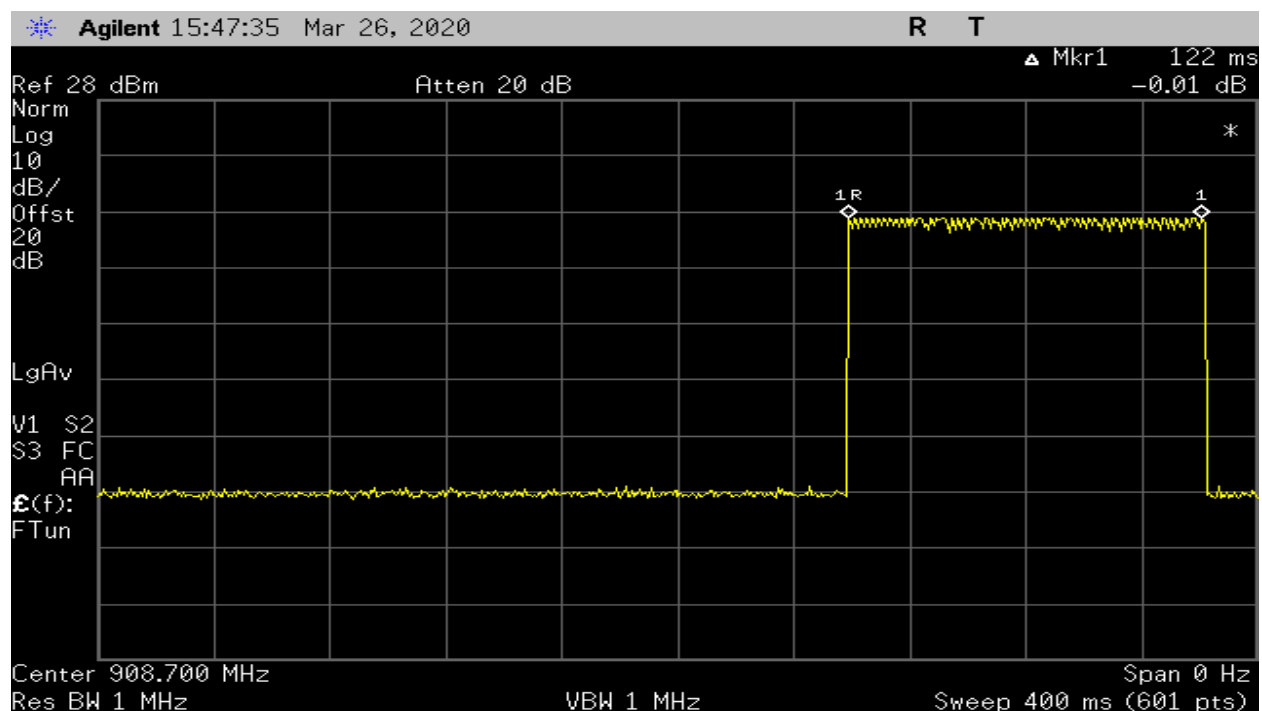
Plot 41 – # of Hops in 0.4 second period – 125kHz BW
