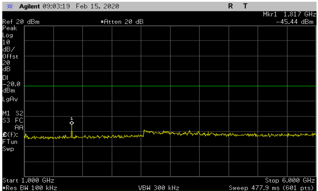
Plot 25 – High Band – 1GHz to 6GHz (Channel 71)
