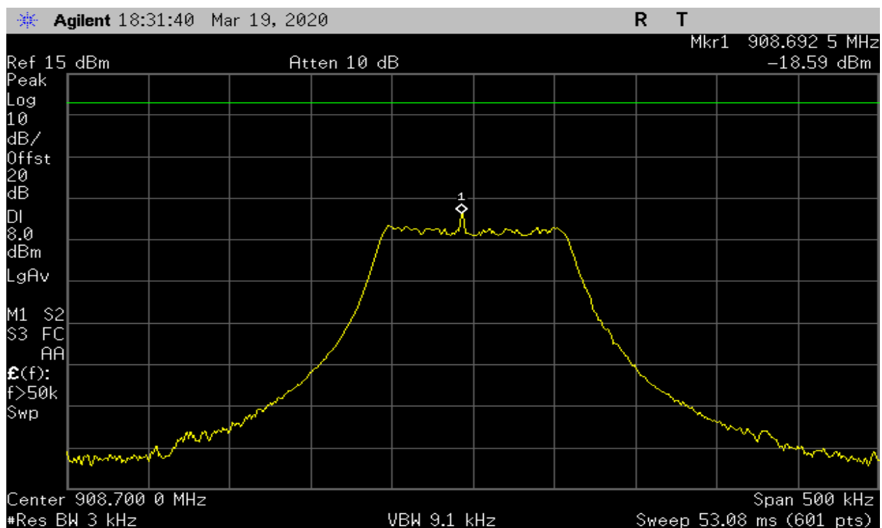
Plot 38 – Power Spectral Density – Middle Channel – 500kHz BW
