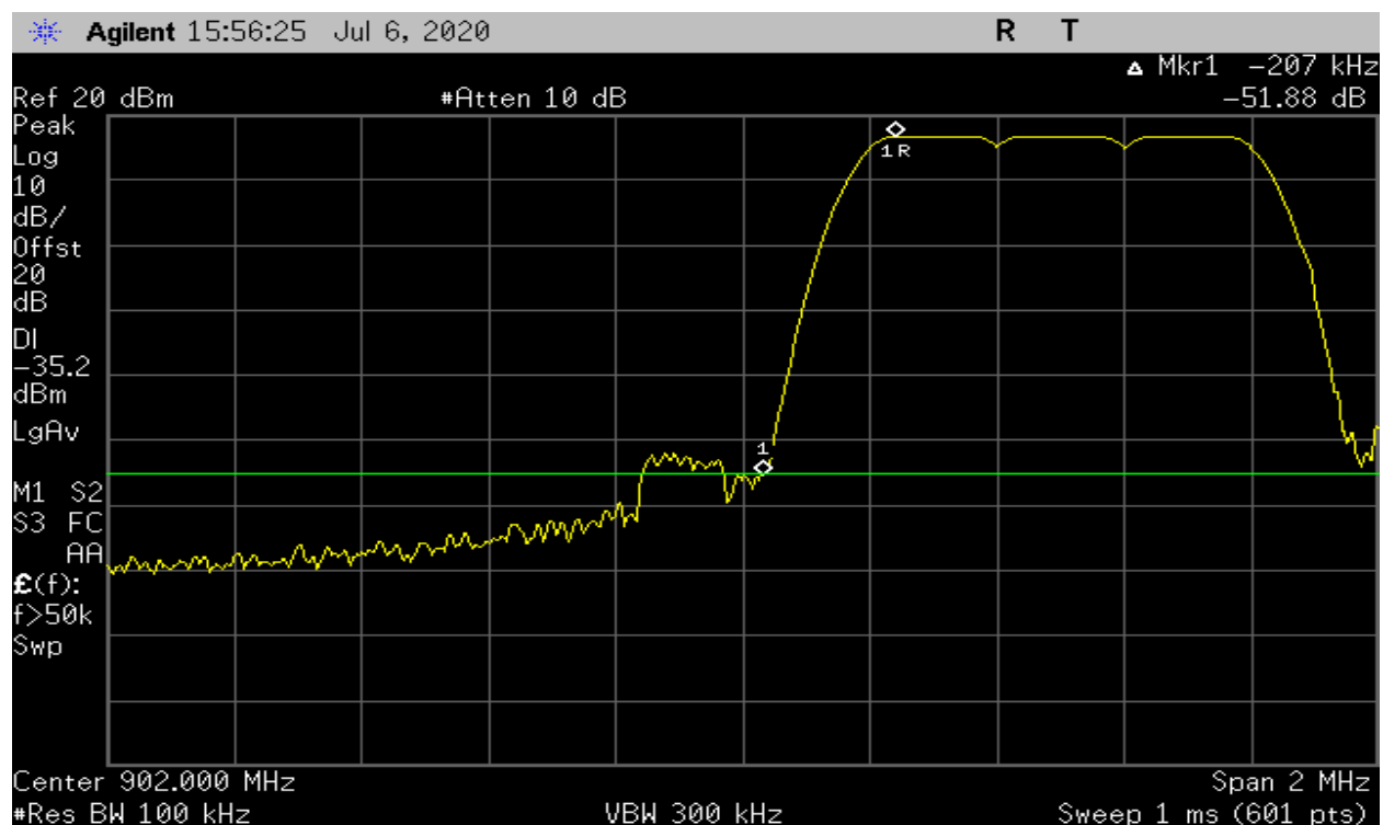
Plot 29 - Band Edge – Low Channel (125kHz BW) – Hopping On
