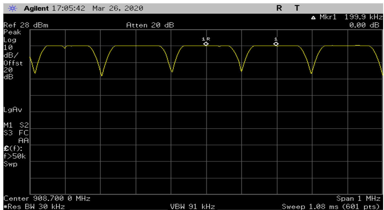
Plot 45 – Carrier Frequency Separation (Using Delta Marker Method) – 125kHz BW
