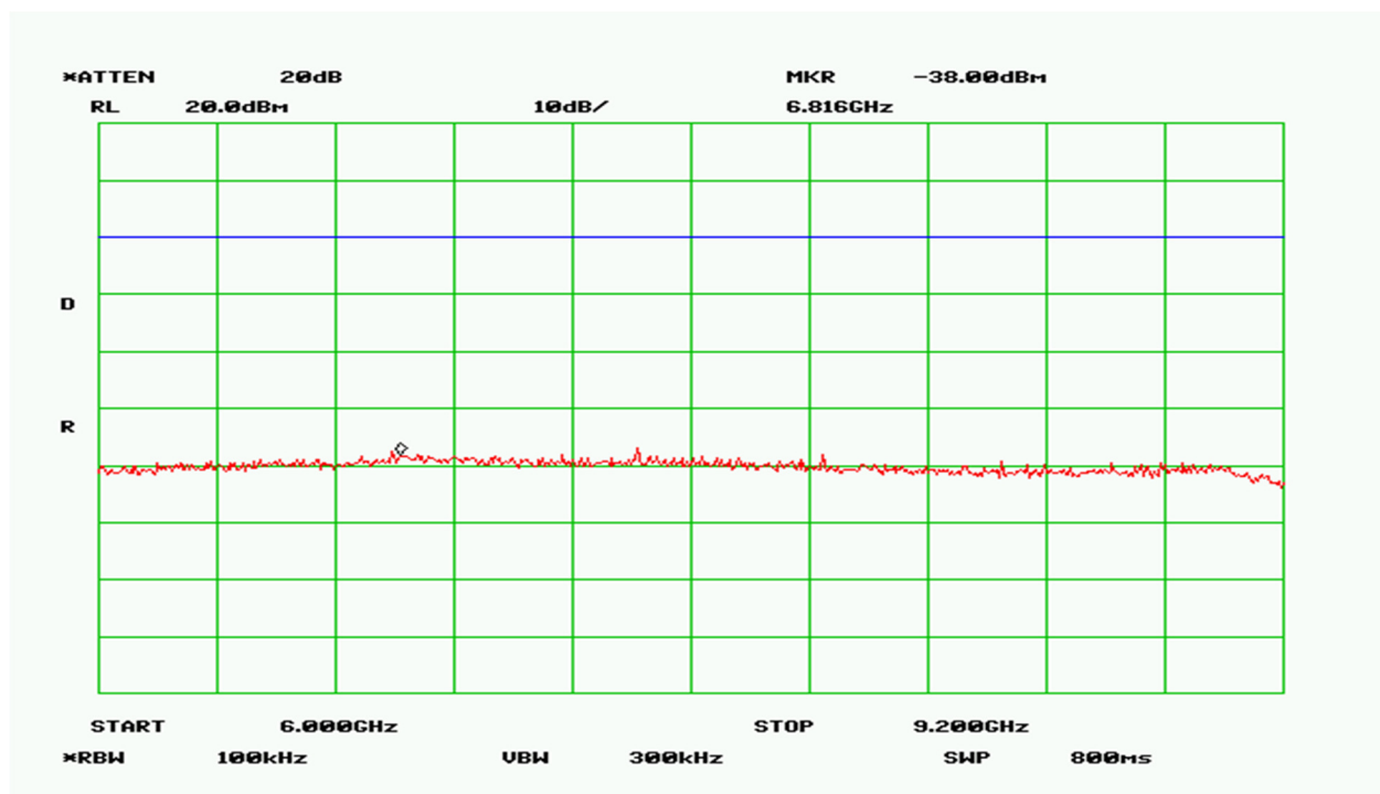
Plot 22 – Mid Band – 6GHz to 9.2GHz (Channel 32)
