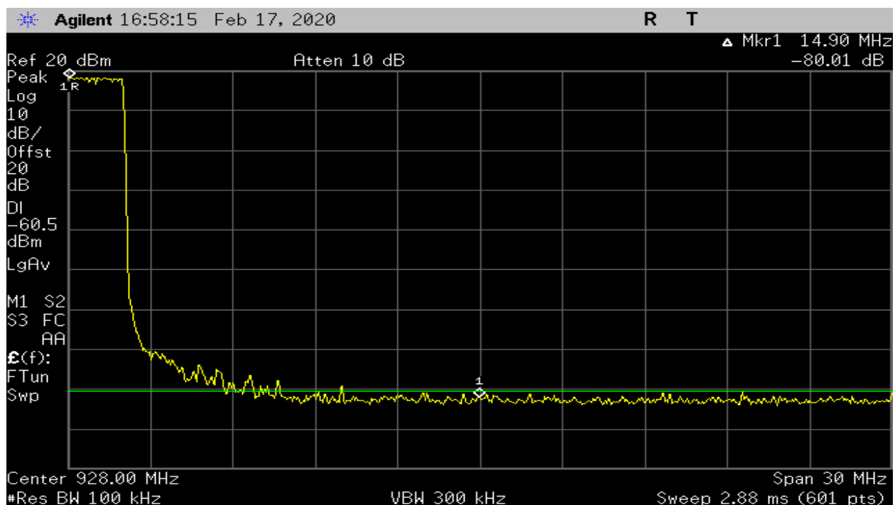
Plot 31 - Band Edge – High Channel (500 kHz BW) – Hopping Off
