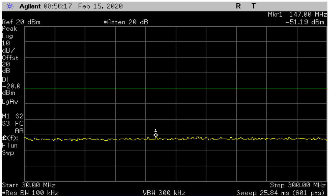
Plot 19 – Mid Band – 30MHz to 300MHz (Channel 32)
