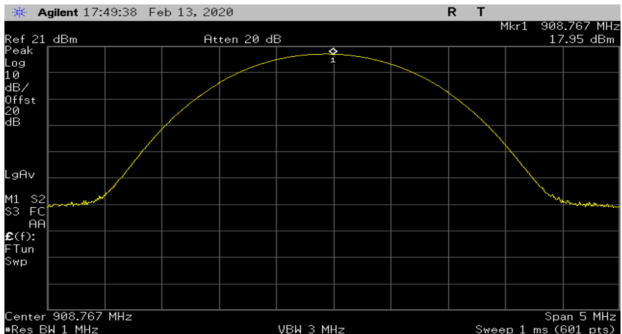
Plot 10 – Output Power – Middle Channel
