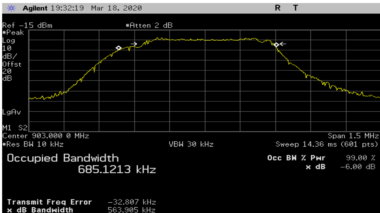
Plot 6 – Lowest Channel – 6dB BW (500kHz BW)
