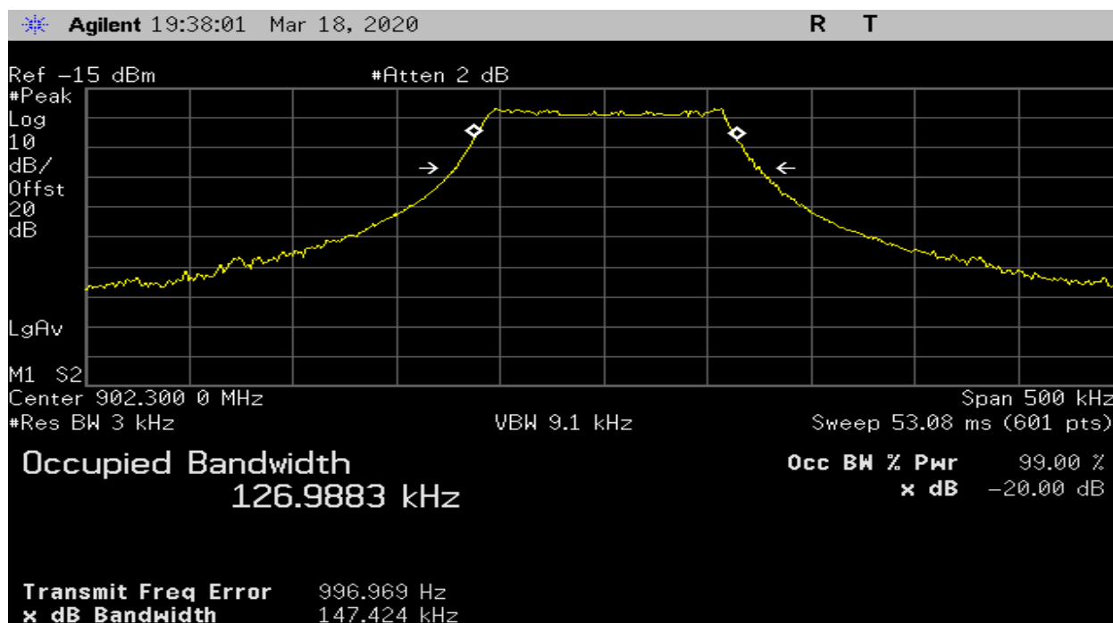
Plot 3 – Lowest Channel – 20dB BW (125kHz BW)
