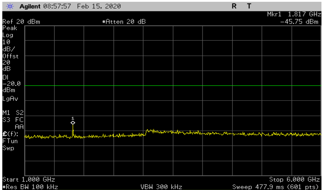
Plot 21 – Mid Band – 1GHz to 6GHz (Channel 32)
