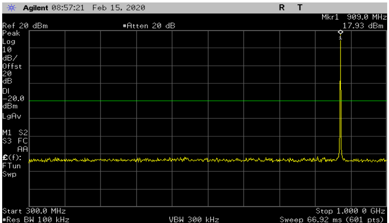
Plot 20 – Mid Band – 300MHz to 1GHz (Channel 32)
