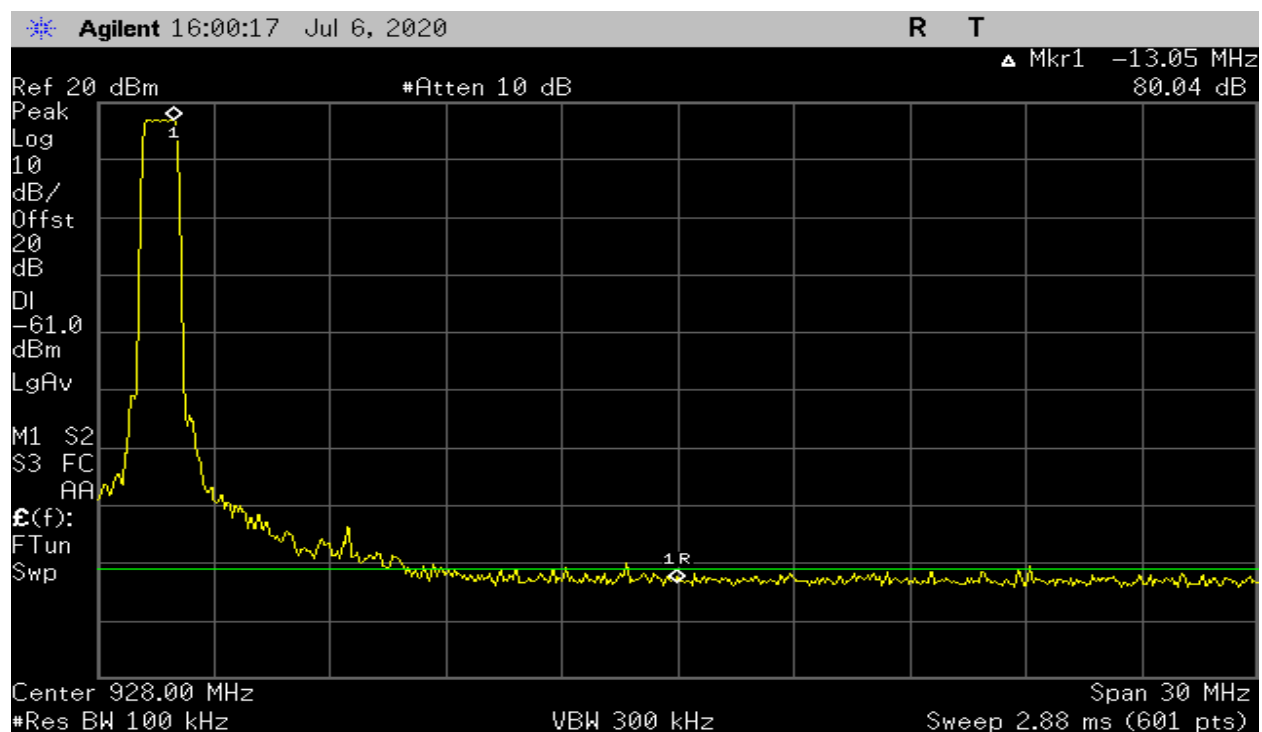
Plot 29 – Band Edge - High Channel (125kHz BW) – Hopping On
