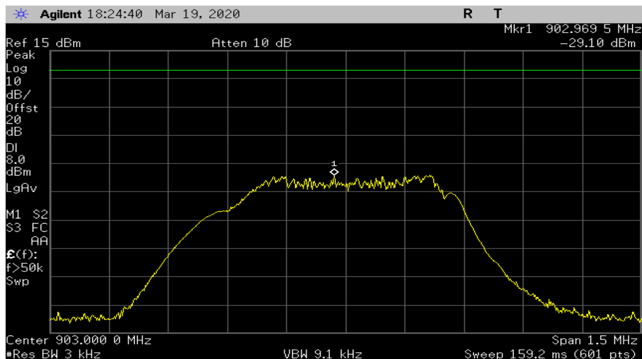
Plot 34 – Power Spectral Density – Lowest Channel – 125kHz BW
