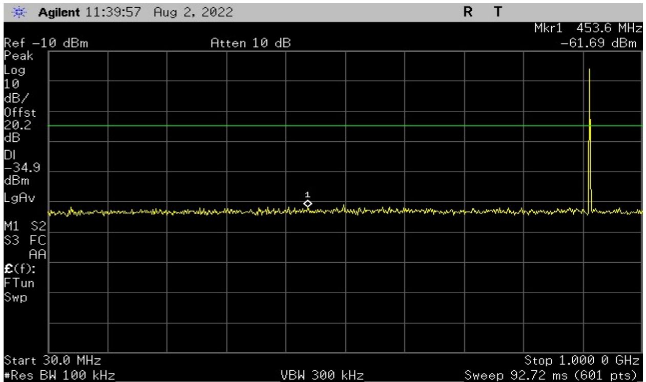
Plot 21 – High Band – 30MHz to 1GHz (Channel 71)
