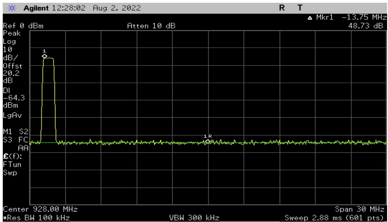
Plot 27 – Band Edge - High Channel (125kHz BW) – Hopping On
