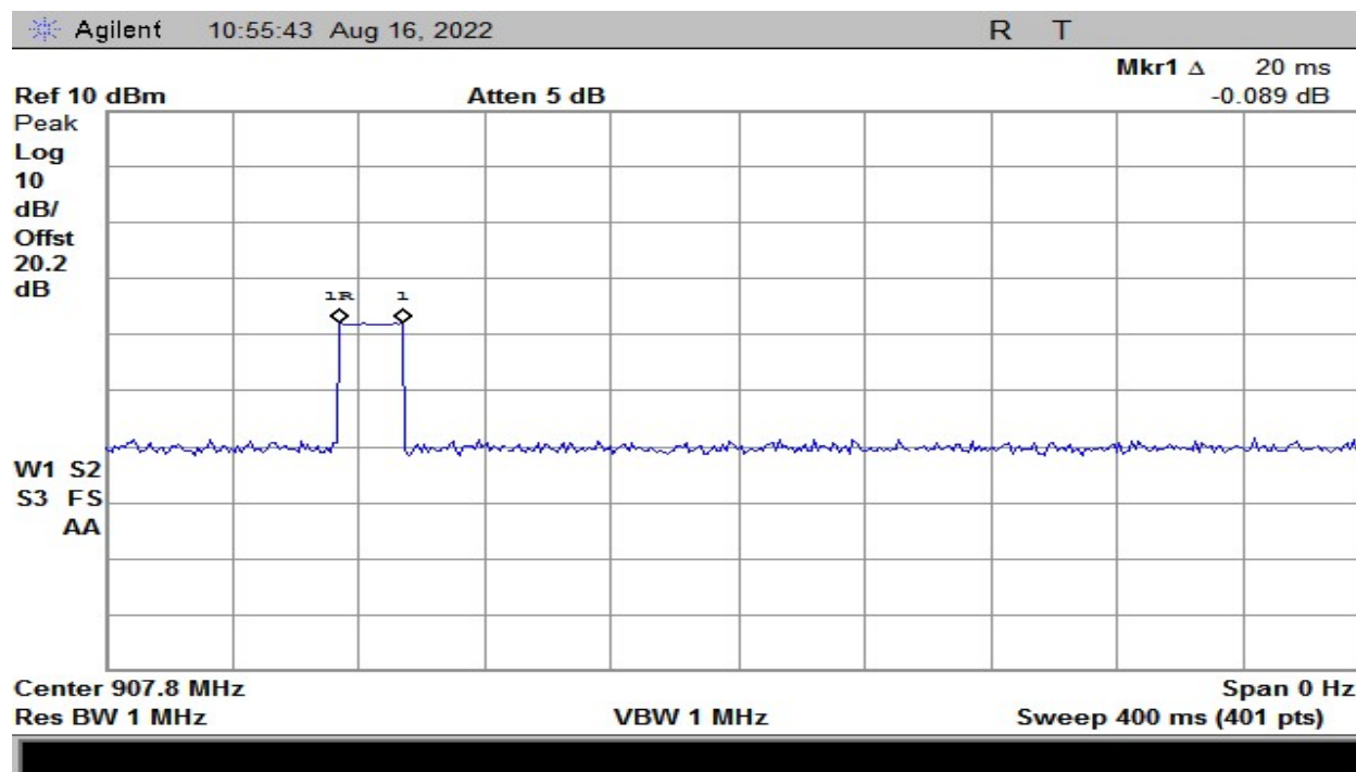
Plot 41 – # of Hops in 0.4 second period – 500kHz BW
