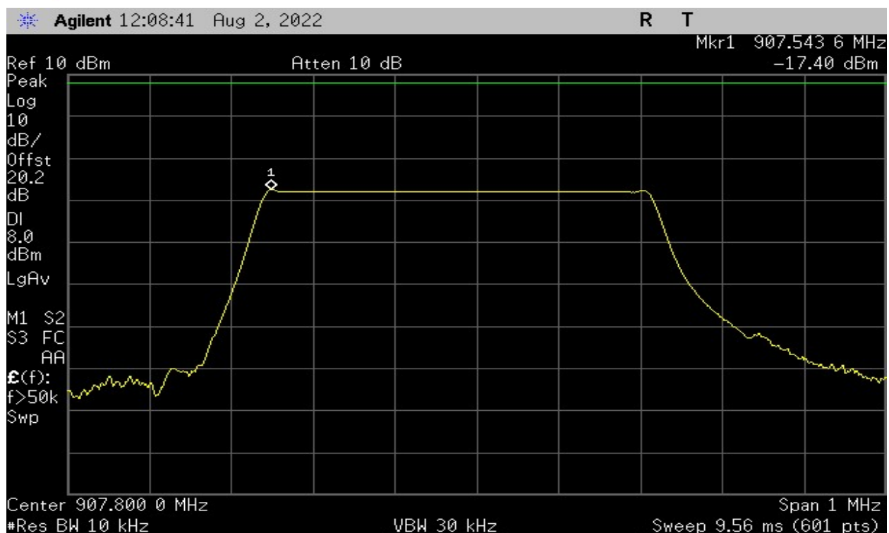
Plot 36 – Power Spectral Density – Middle Channel – 500kHz BW
