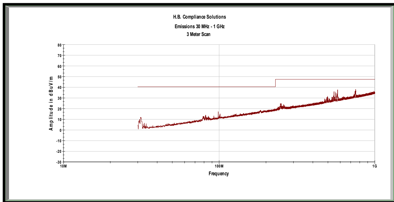
Plot 1 – Radiated Emissions – 30MHz to 1GHz
