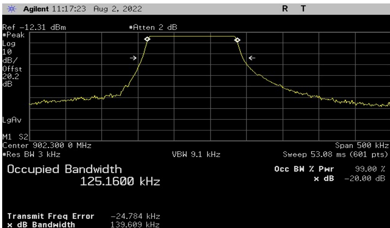
Plot 3 – Lowest Channel – 20dB BW (125kHz BW)
