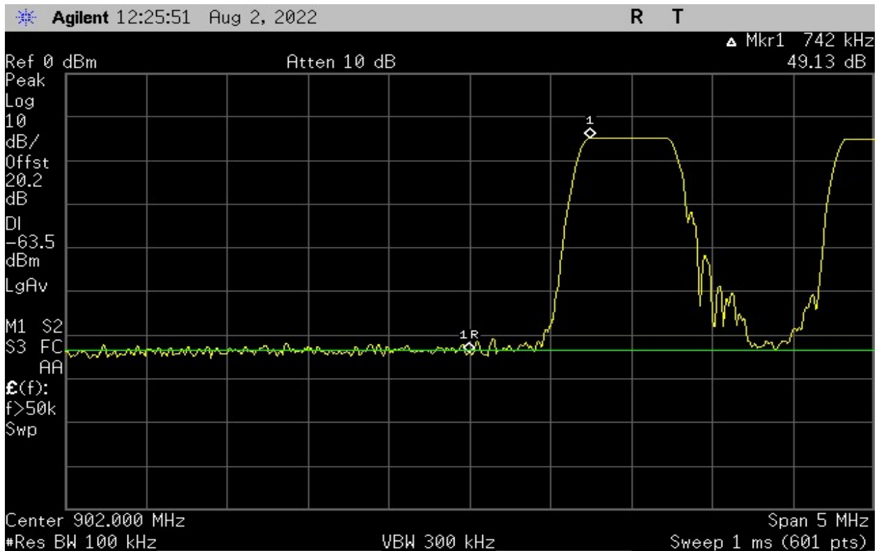
Plot 30 - Band Edge – Low Channel (500kHz BW) – Hopping On
