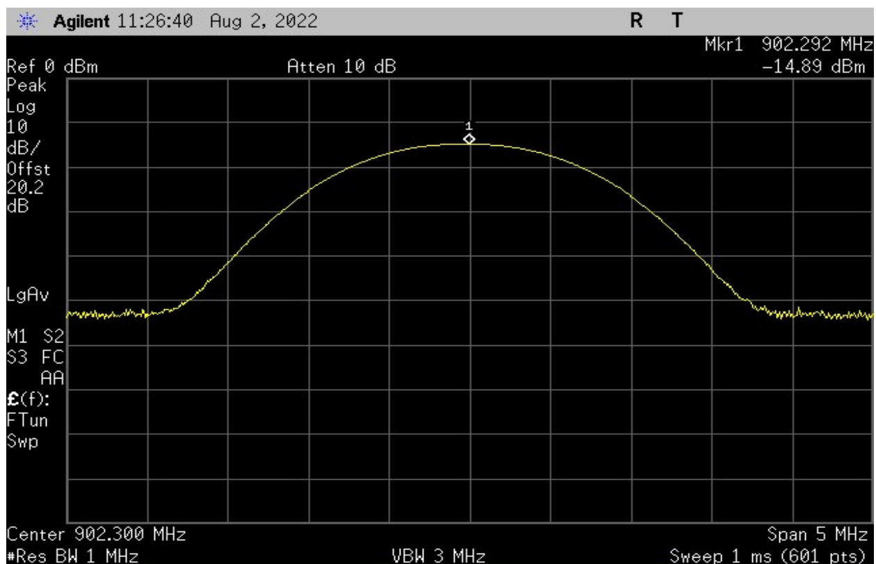
Plot 9 – Output Power – Lowest Channel
