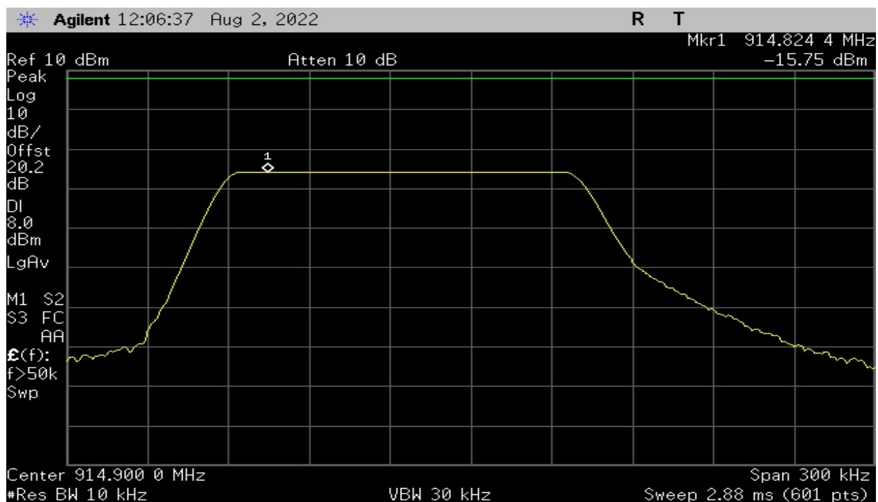
Plot 34 – Power Spectral Density – Highest Channel – 125kHz BW
