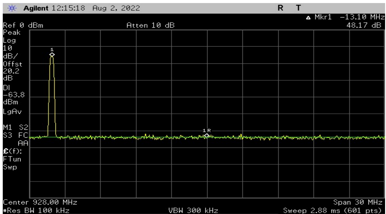
Plot 25 – Band Edge - High Channel (125kHz BW) – Hopping Off
