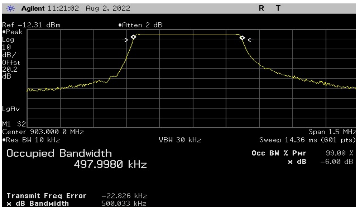
Plot 6 – Lowest Channel – 6dB BW (500kHz BW)
