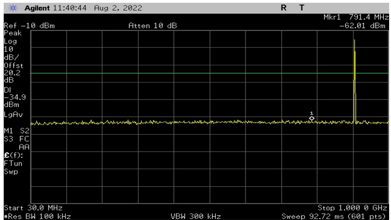
Plot 18 – Mid Band – 30MHz to 1GHz (Channel 32)
