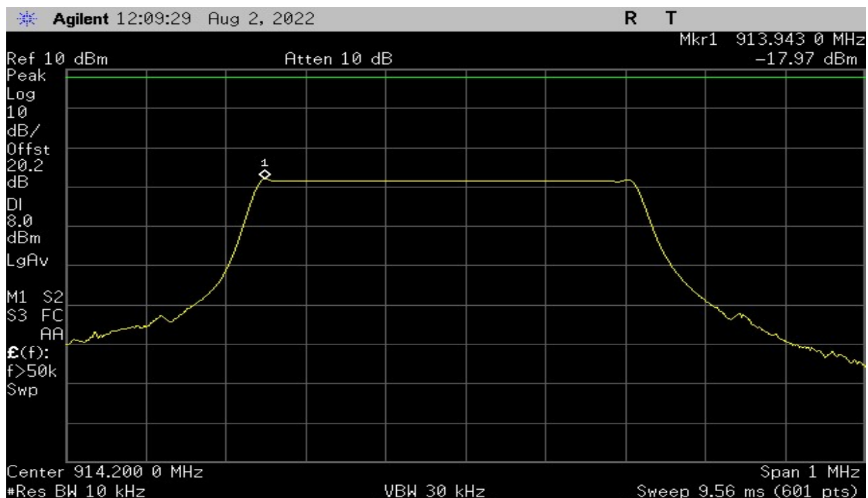
Plot 37 – Power Spectral Density – Highest Channel – 500kHz BW
