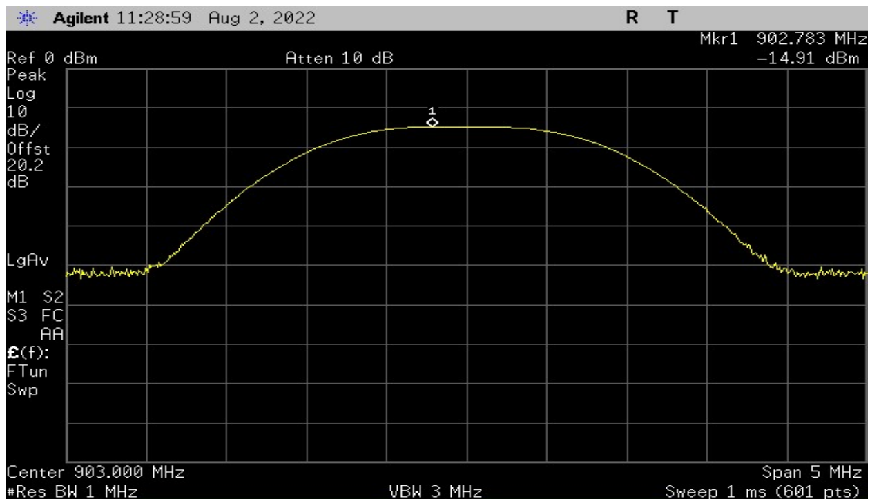
Plot 12 – Output Power – Lowest Channel (500kHz BW)
