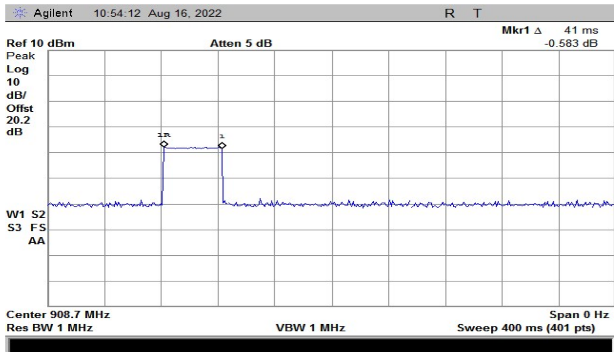
Plot 39 – # of Hops in 0.4 second period – 125kHz BW
