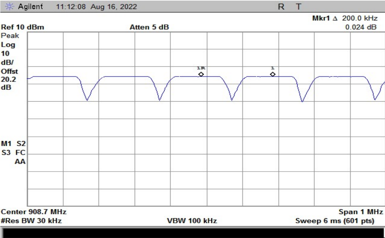
Plot 43 – Carrier Frequency Separation (Using Delta Marker Method) – 125kHz BW
