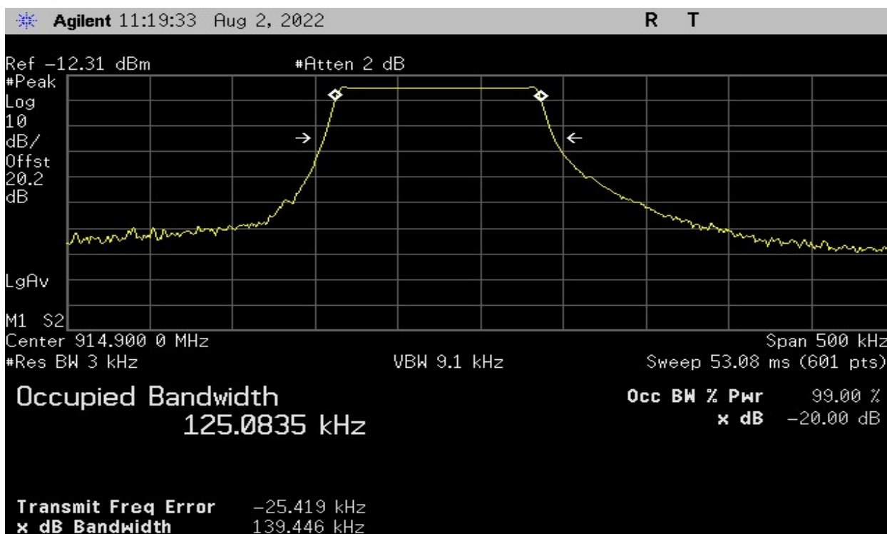
Plot 5 – Highest Channel – 20dB BW (125kHz BW)
