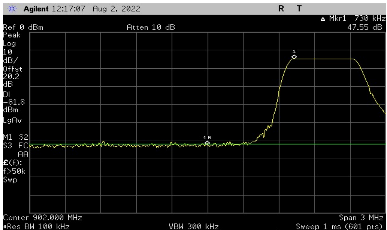
Plot 28 - Band Edge – Low Channel (500kHz BW) – Hopping Off
