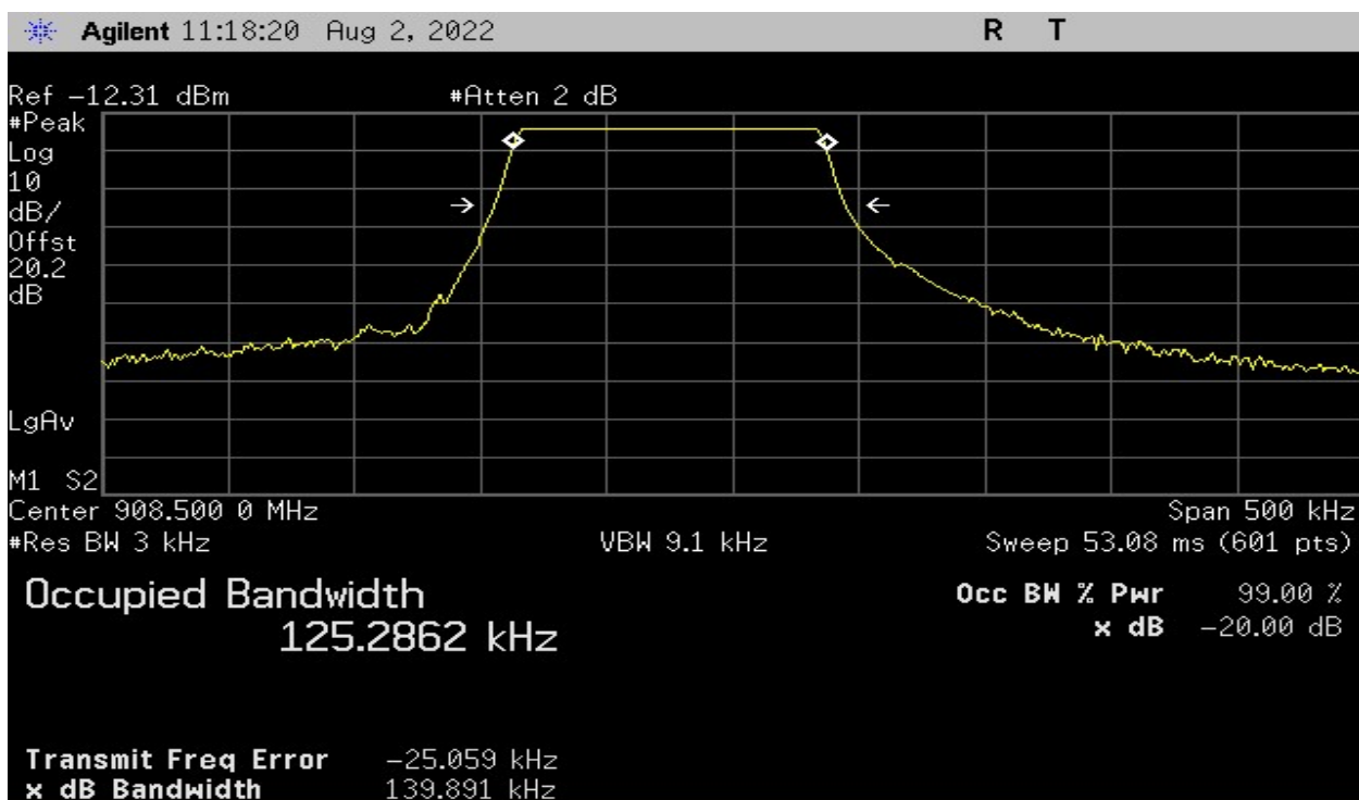
Plot 4 – Middle Channel – 20dB BW (125kHz BW)
