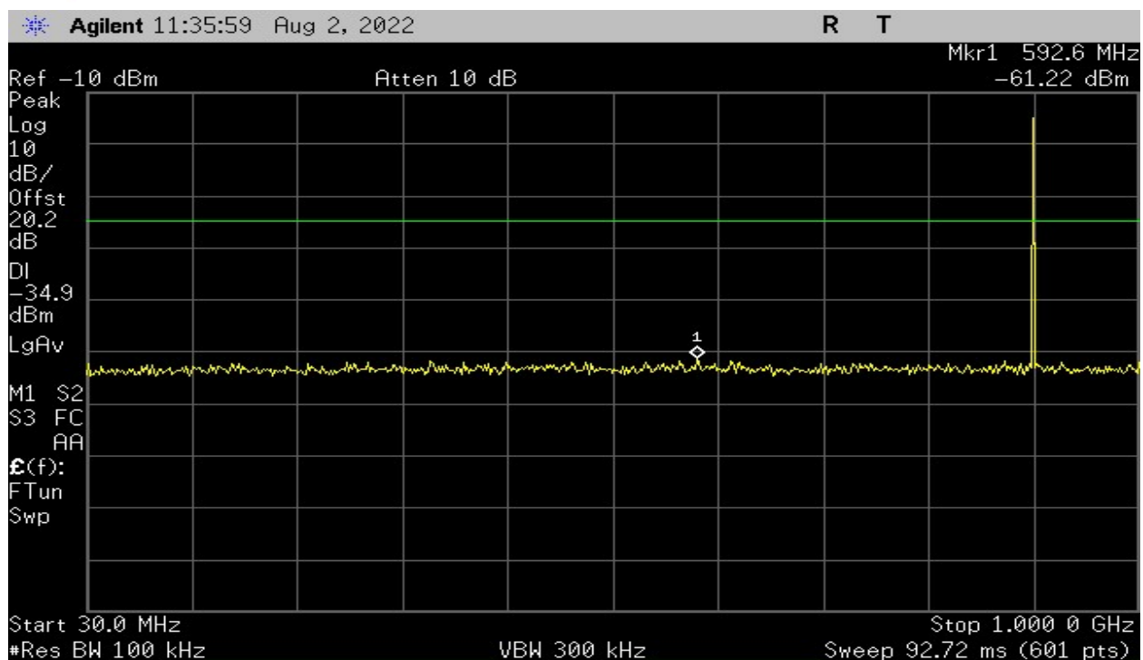
Plot 15 – Low Band – 30MHz to 1GHz (Channel 0)
