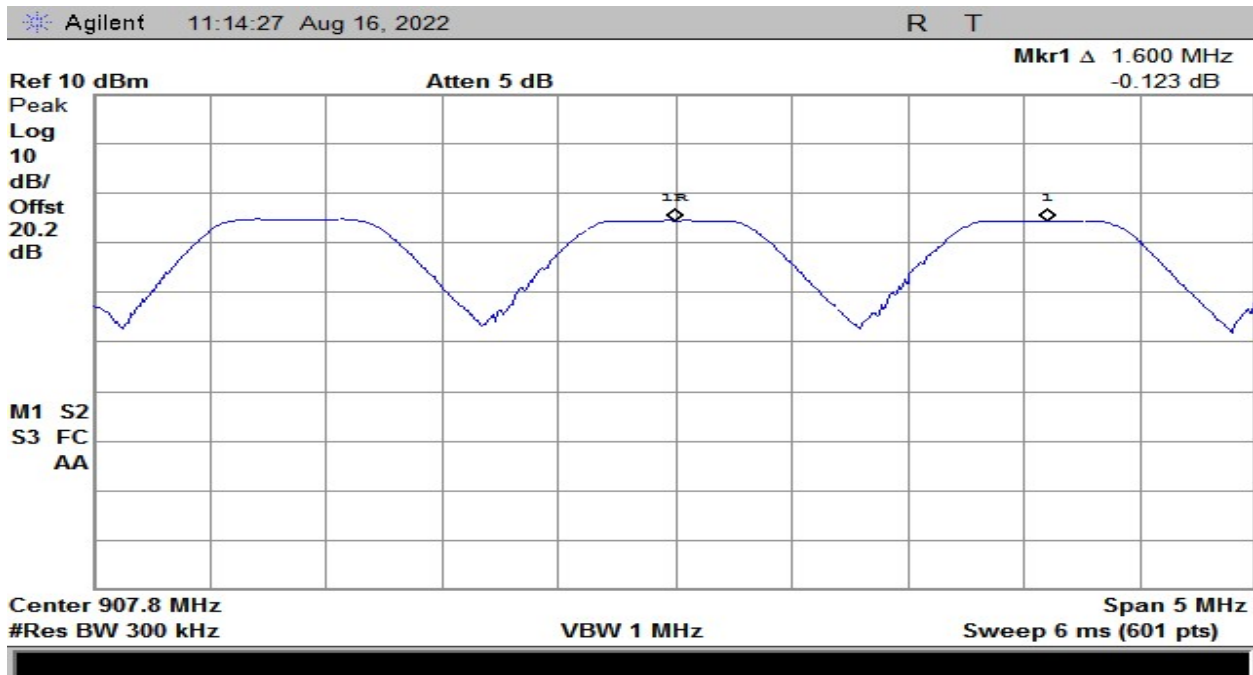
Plot 44 – Carrier Frequency Separation (Using Delta Marker Method) – 500kHz BW
