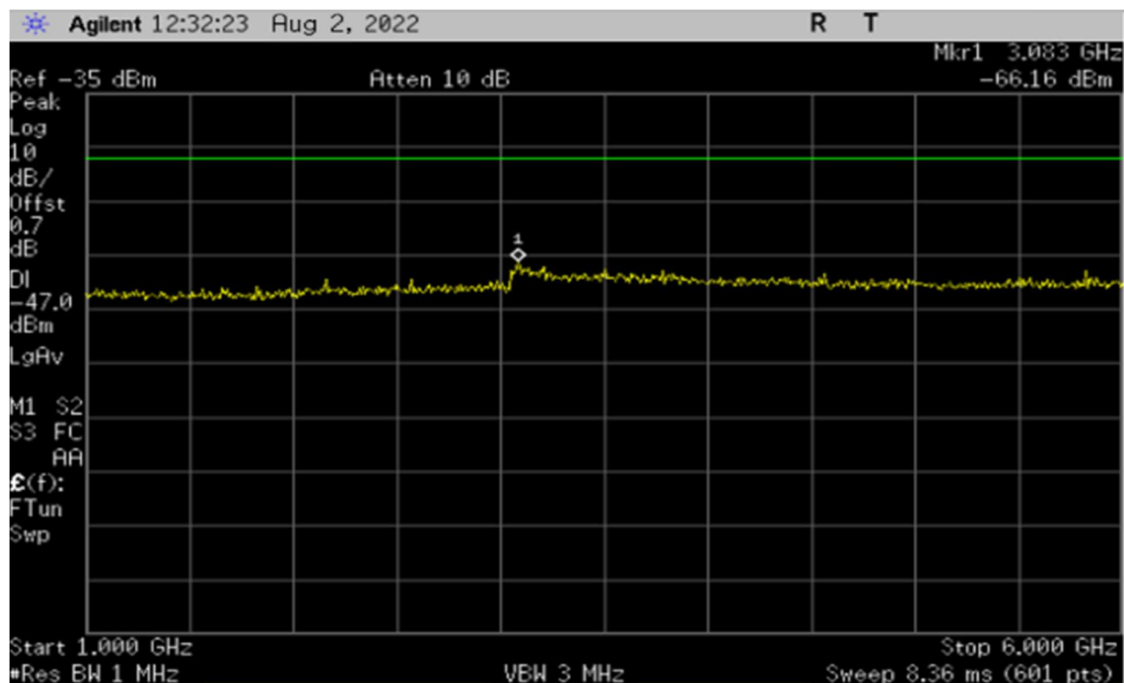
Plot 2 – Receiver Emissions (Conducted) – 1GHz to 6GHz (For Industry Canada RSS-GEN)
