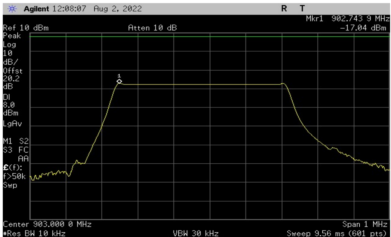
Plot 35 – Power Spectral Density – Lowest Channel – 500kHz BW
