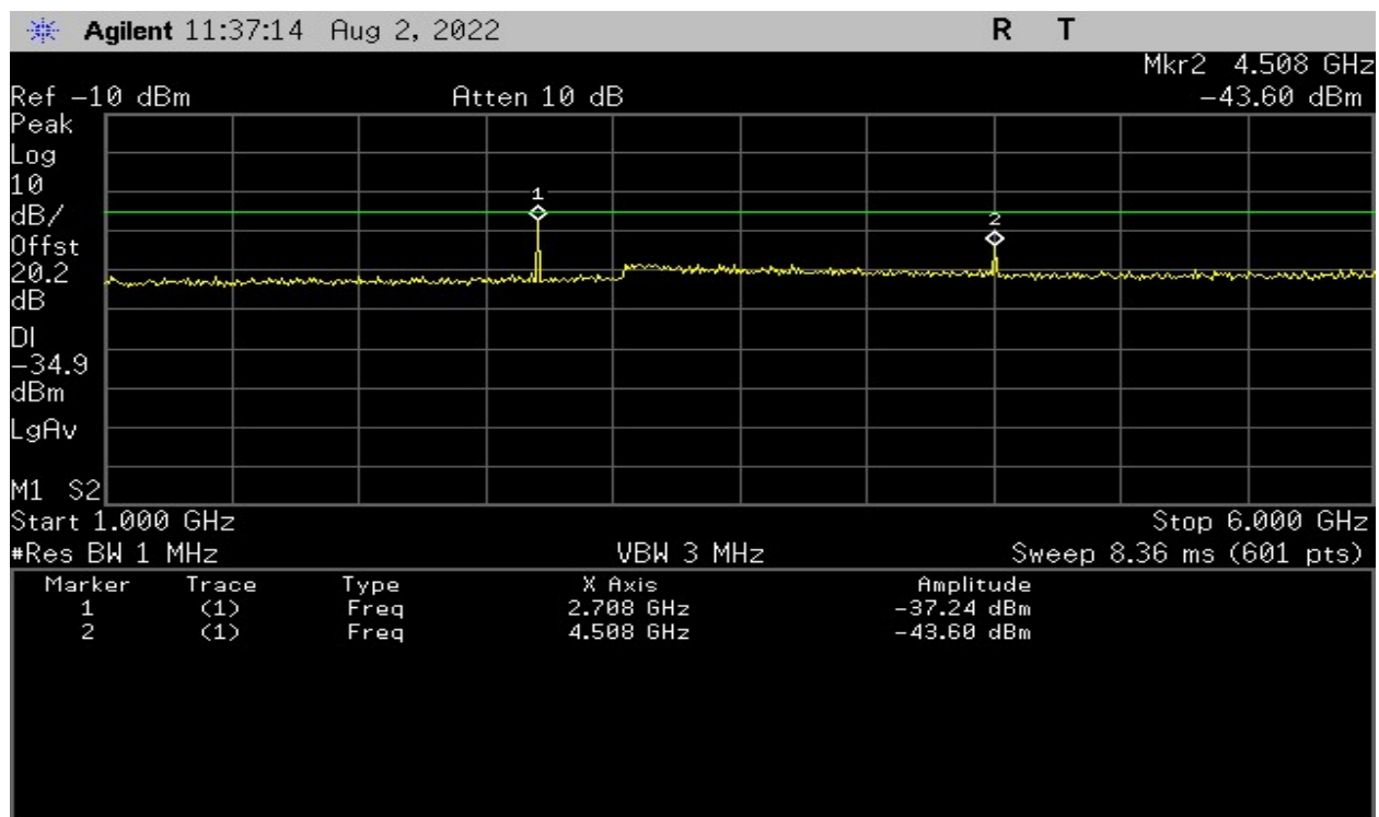
Plot 16 – Low Band – 1GHz to 6GHz (Channel 0)
