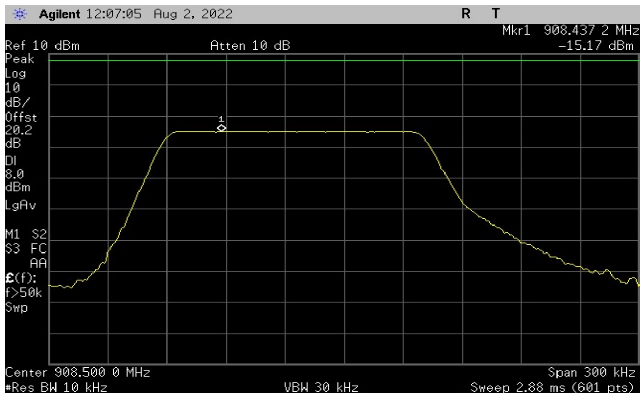
Plot 33 – Power Spectral Density – Middle Channel – 125kHz BW
