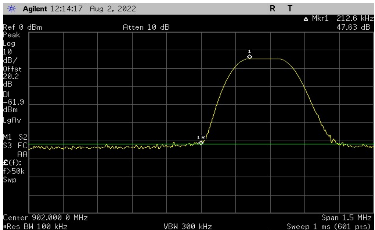
Plot 24 - Band Edge – Low Channel (125kHz BW) – Hopping Off
