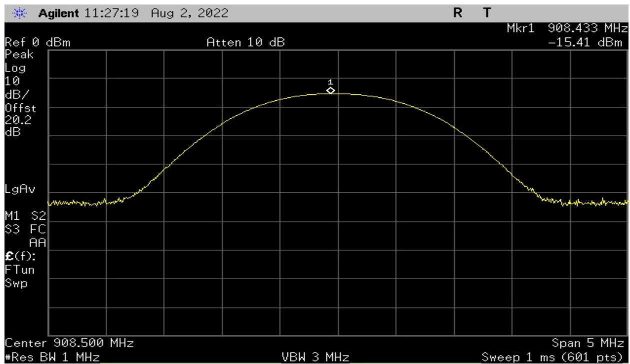
Plot 10 – Output Power – Middle Channel
