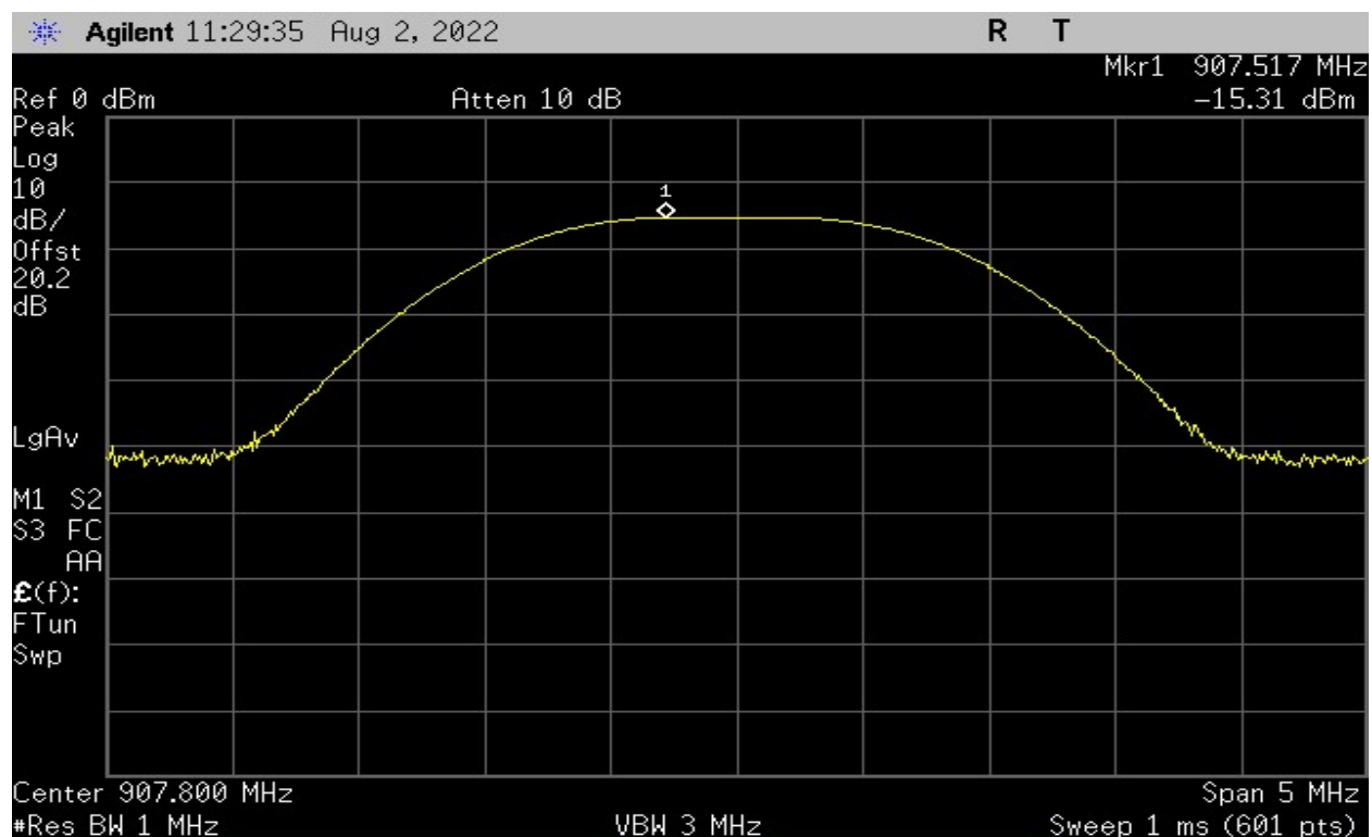
Plot 13 – Output Power – Middle Channel (500kHz BW)
