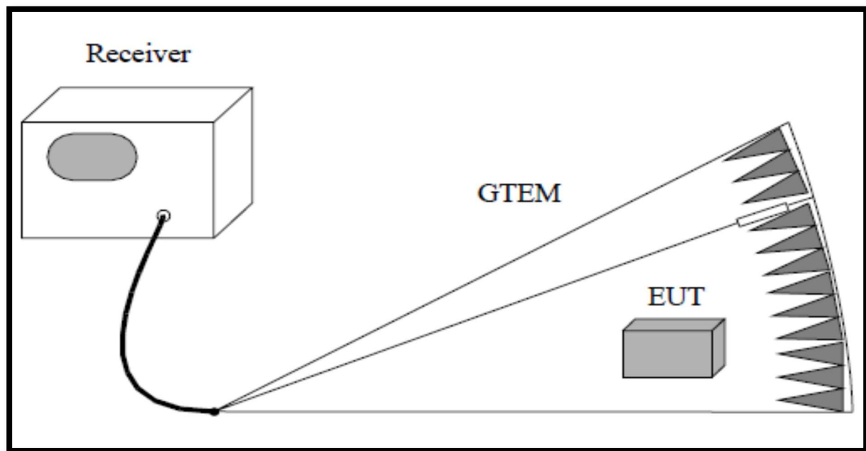
Figure 1. Radiated Emissions Test Setup (30MHz – 1GHz)
