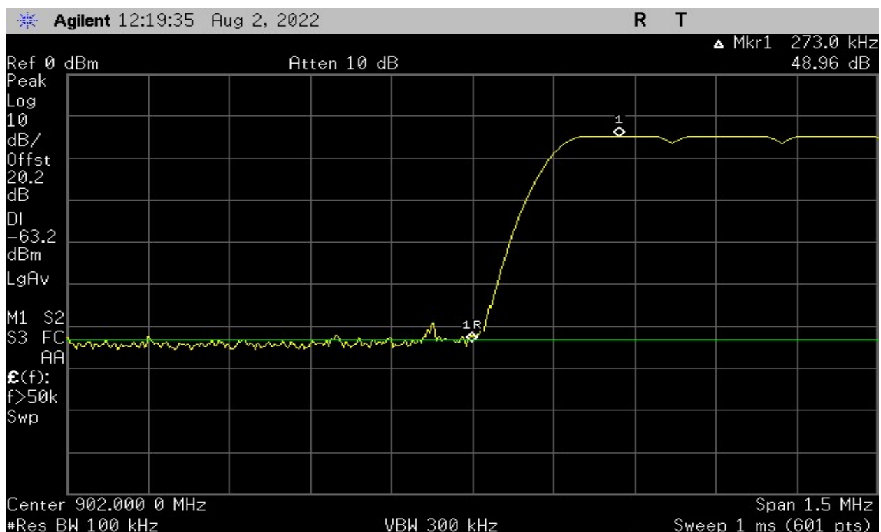
Plot 26 - Band Edge – Low Channel (125kHz BW) – Hopping On
