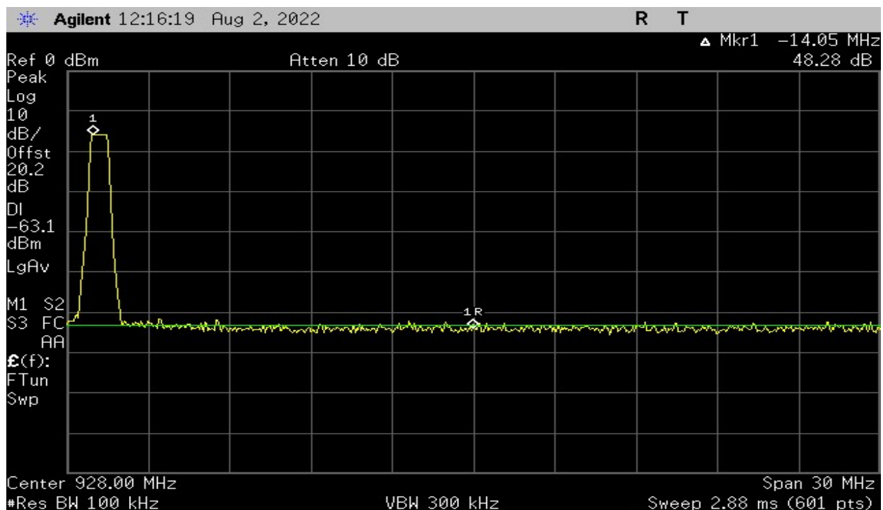
Plot 29 - Band Edge – High Channel (500 kHz BW) – Hopping Off
