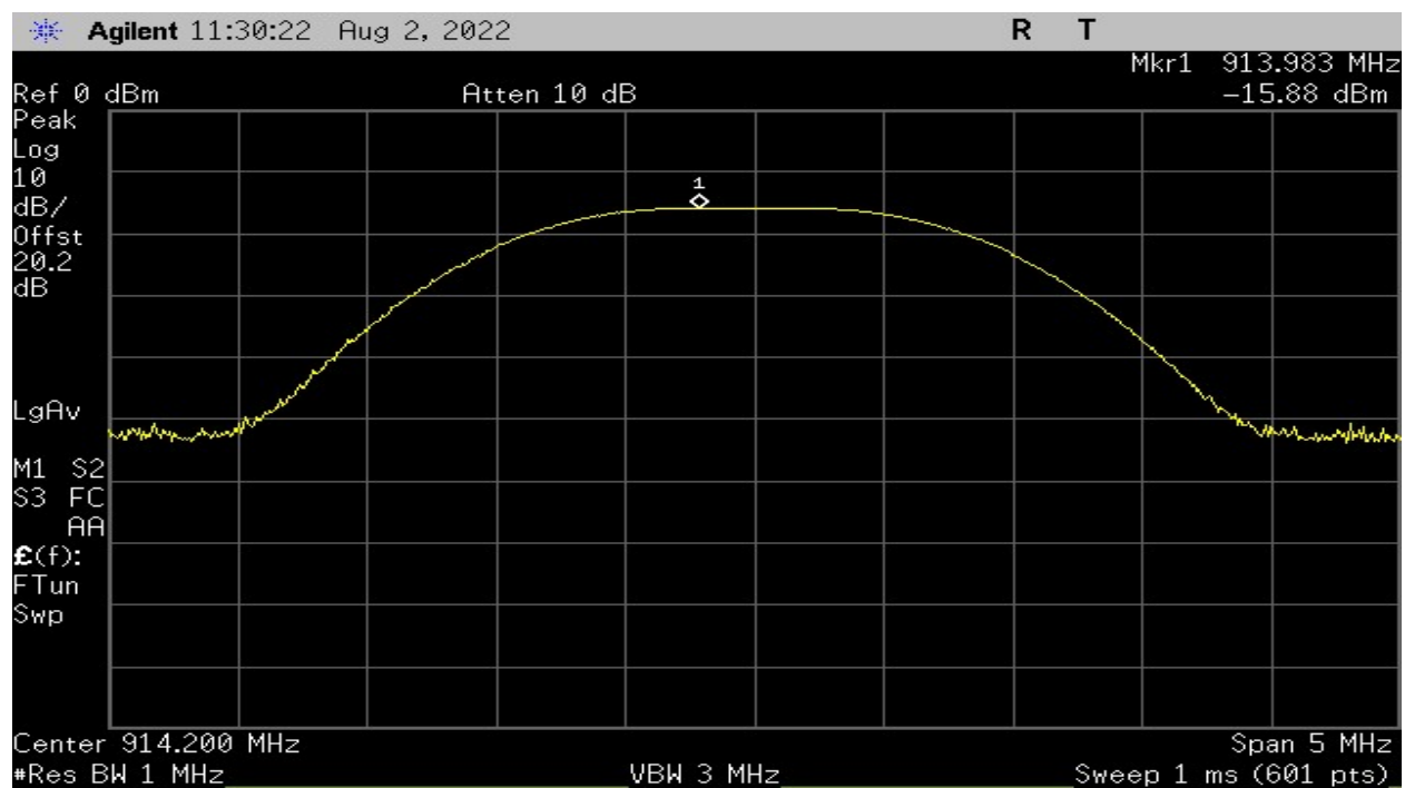
Plot 14 – Output Power – Highest Channel (500kHz)
