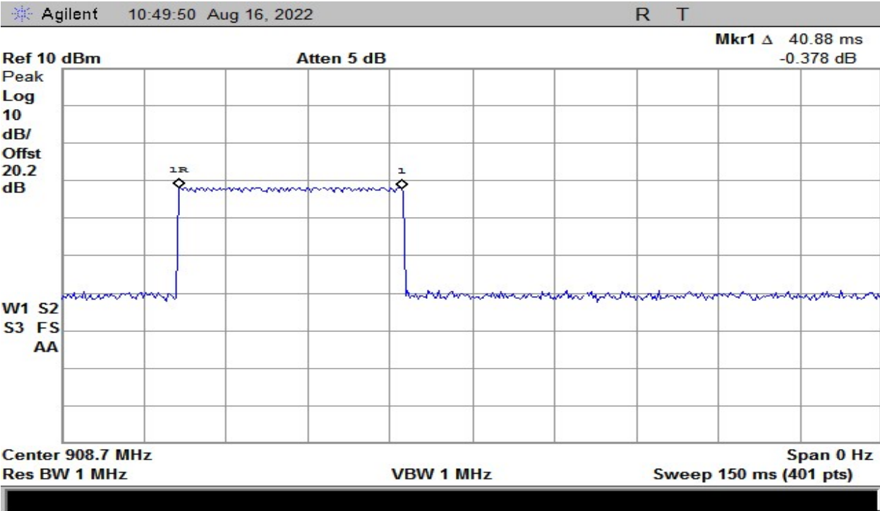
Plot 38 – Dwell Time (125kHz BW)
