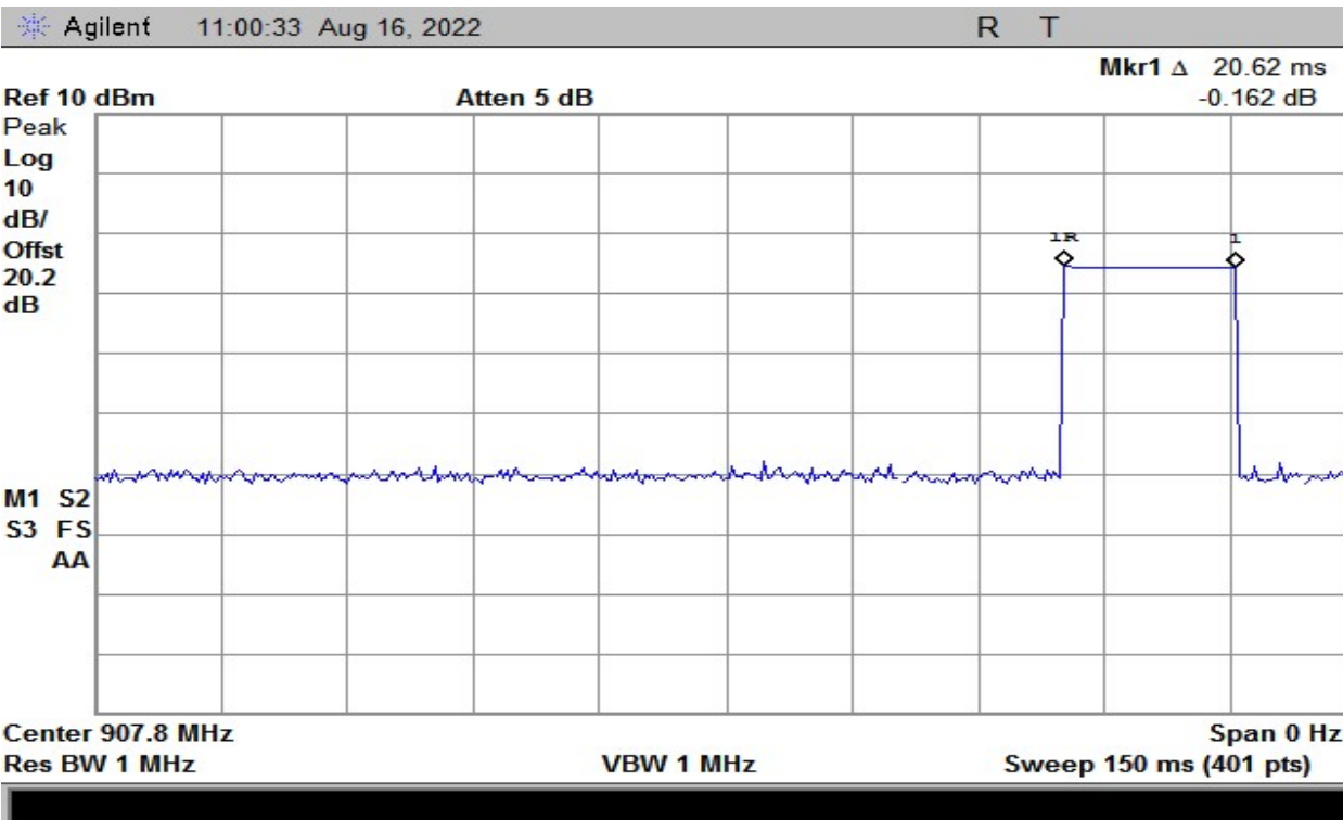
Plot 40 – Dwell Time (500kHz BW)
