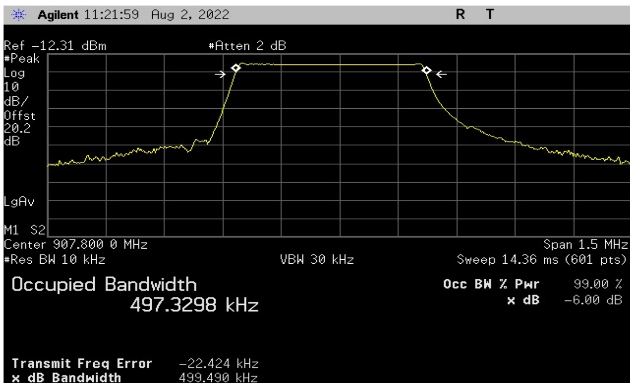
Plot 7 – Middle Channel – 6dB BW (500kHz BW)
