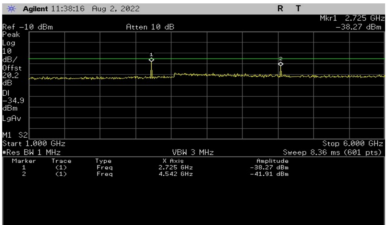
Plot 19 – Mid Band – 1GHz to 6GHz (Channel 32)
