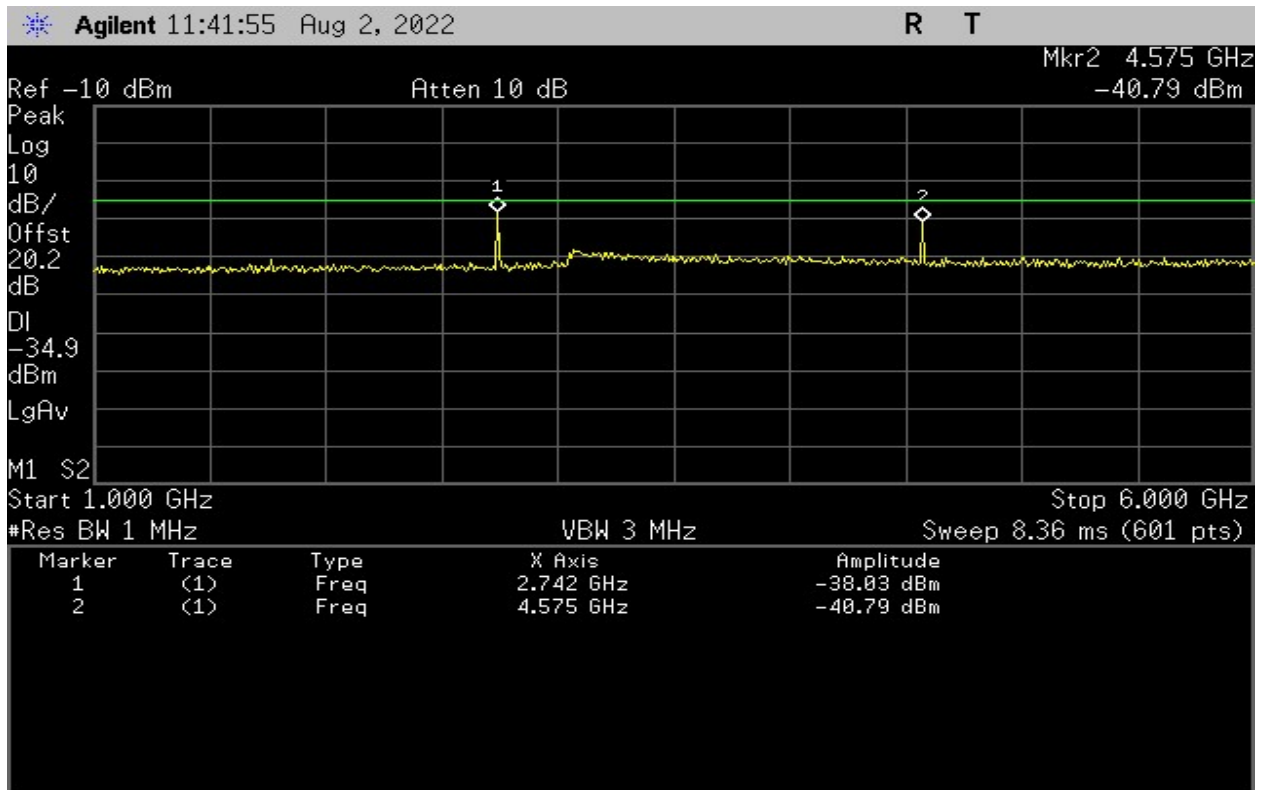
Plot 22 – High Band – 1GHz to 6GHz (Channel 71)
