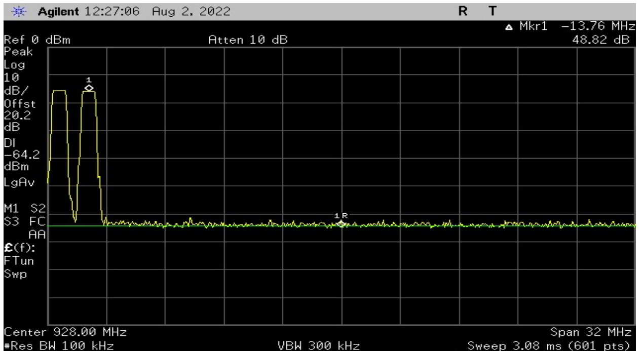
Plot 31 - Band Edge – High Channel (500 kHz BW) – Hopping On
