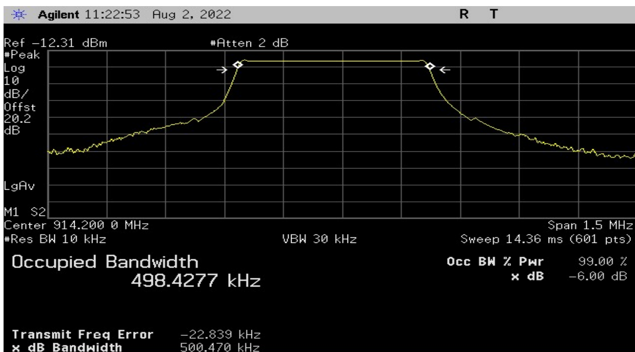
Plot 8 – Highest Channel – 6dB BW (500 kHz BW)
