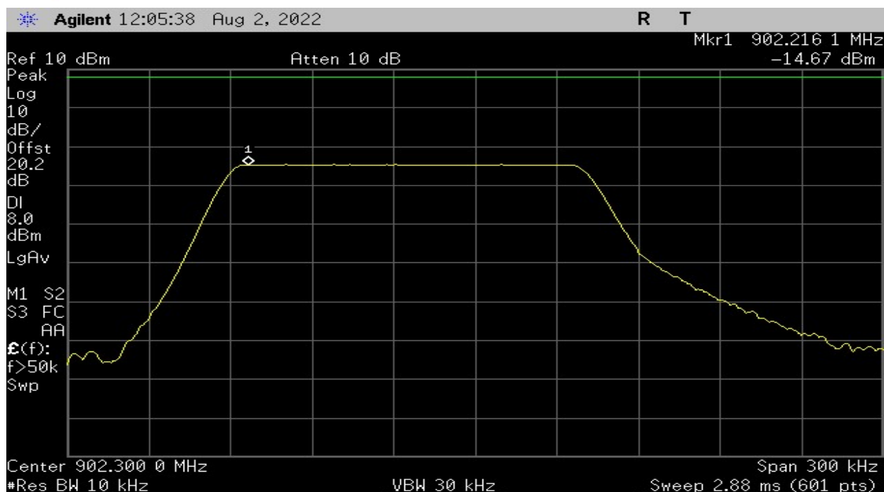
Plot 32 – Power Spectral Density – Lowest Channel – 125kHz BW
