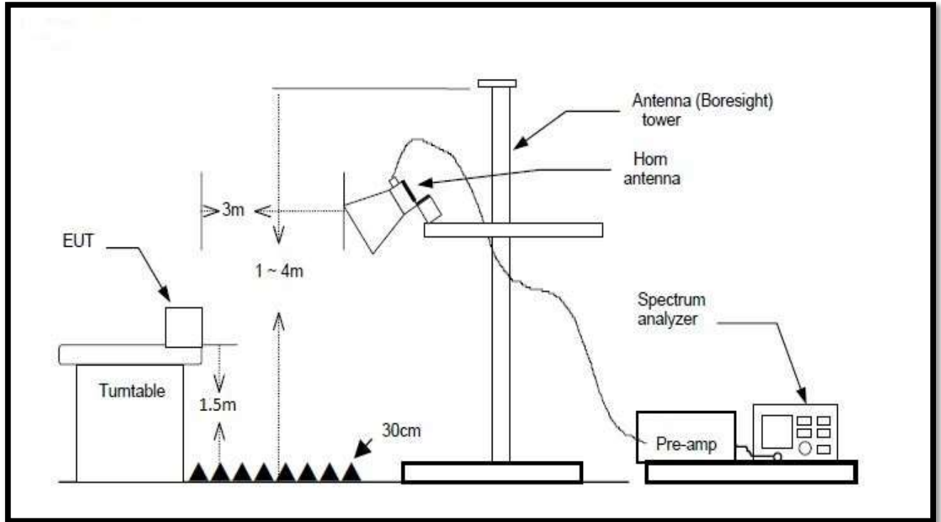
Figure 5. Radiated Emission Above 1GHz Test Setup
