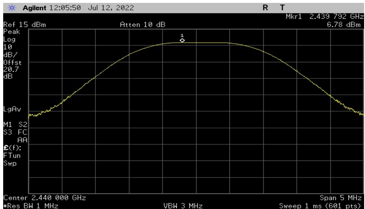
Plot 7 – Output Power – Middle Channel
