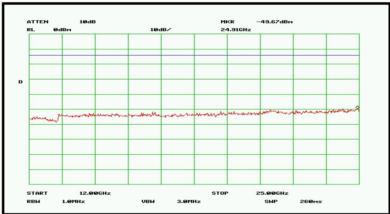
Plot 20 – High Band – 12GHz to 25GHz
