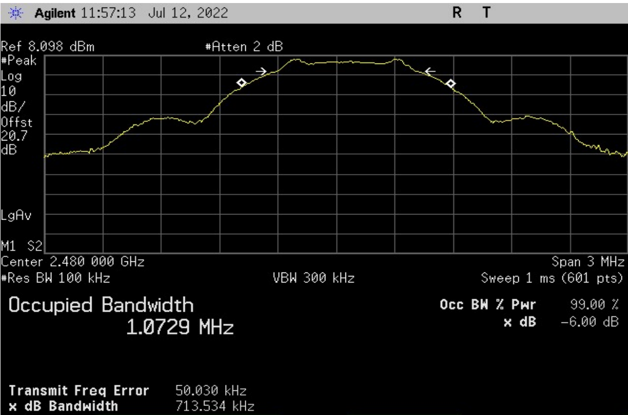
Plot 5 – Highest Channel – 6dB BW
