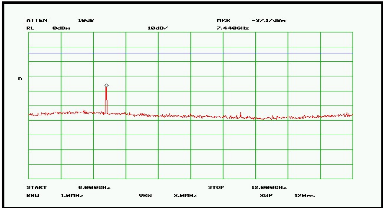
Plot 19 – High Band – 6GHz to 12GHz
