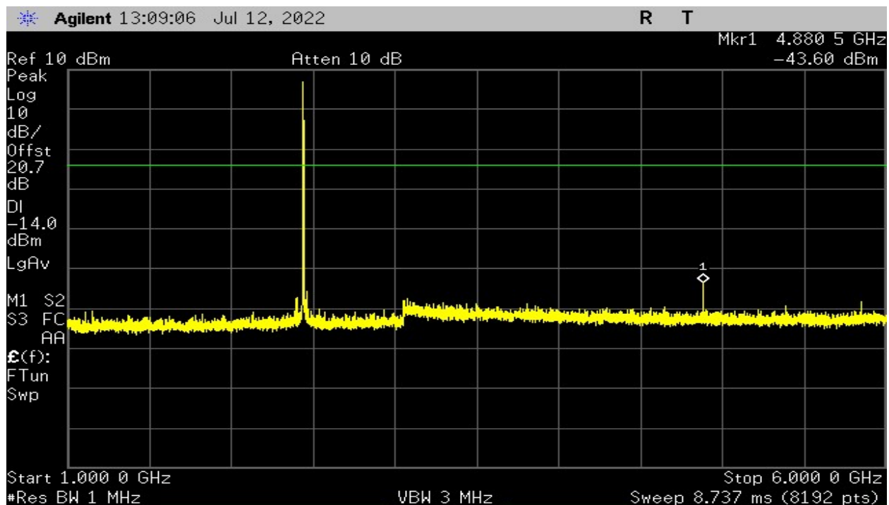
Plot 14 – Mid Band – 1GHz to 6GHz
