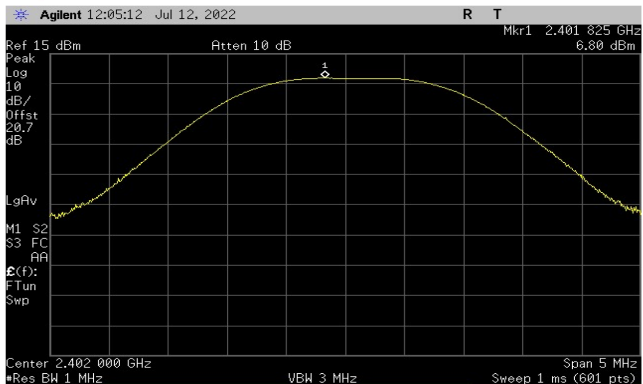
Plot 6 – Output Power – Lowest Channel
