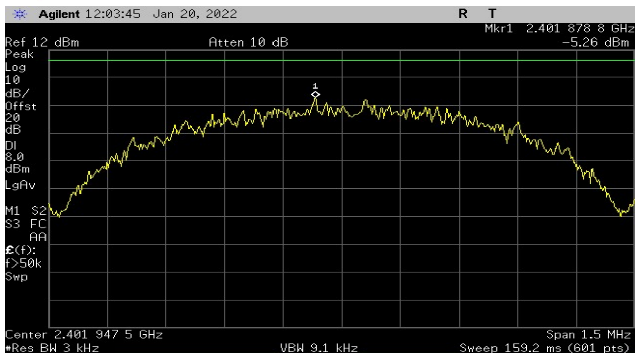
Plot 24 – Power Spectral Density – Lowest Channel
