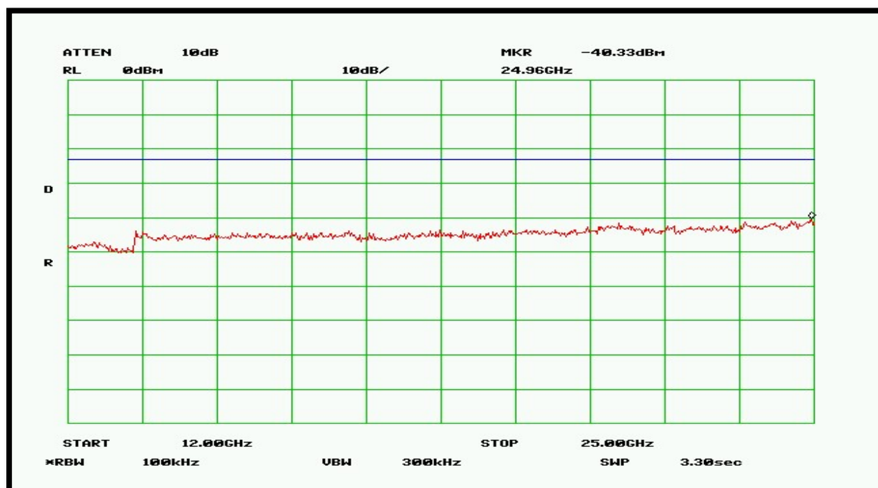
Plot 21 – High Band – 12GHz to 25GHz
