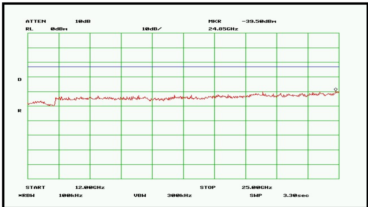
Plot 13 – Low Band – 12GHz to 25GHz
