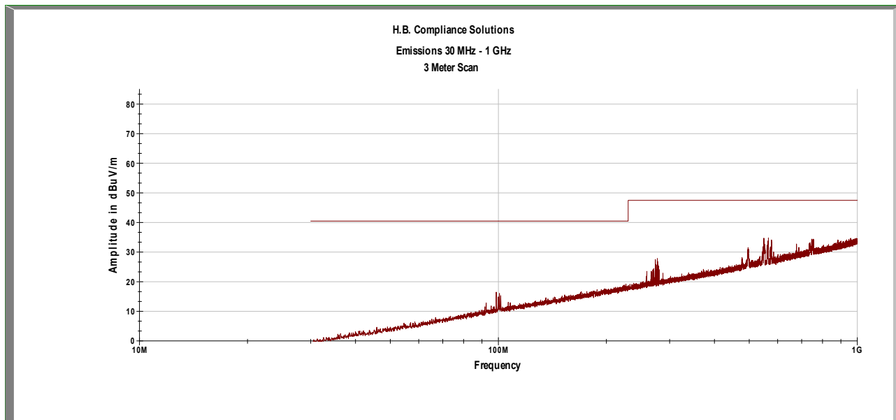
Plot 2 – Radiated Emissions – 30MHz to 1GHz – (Sensor)
