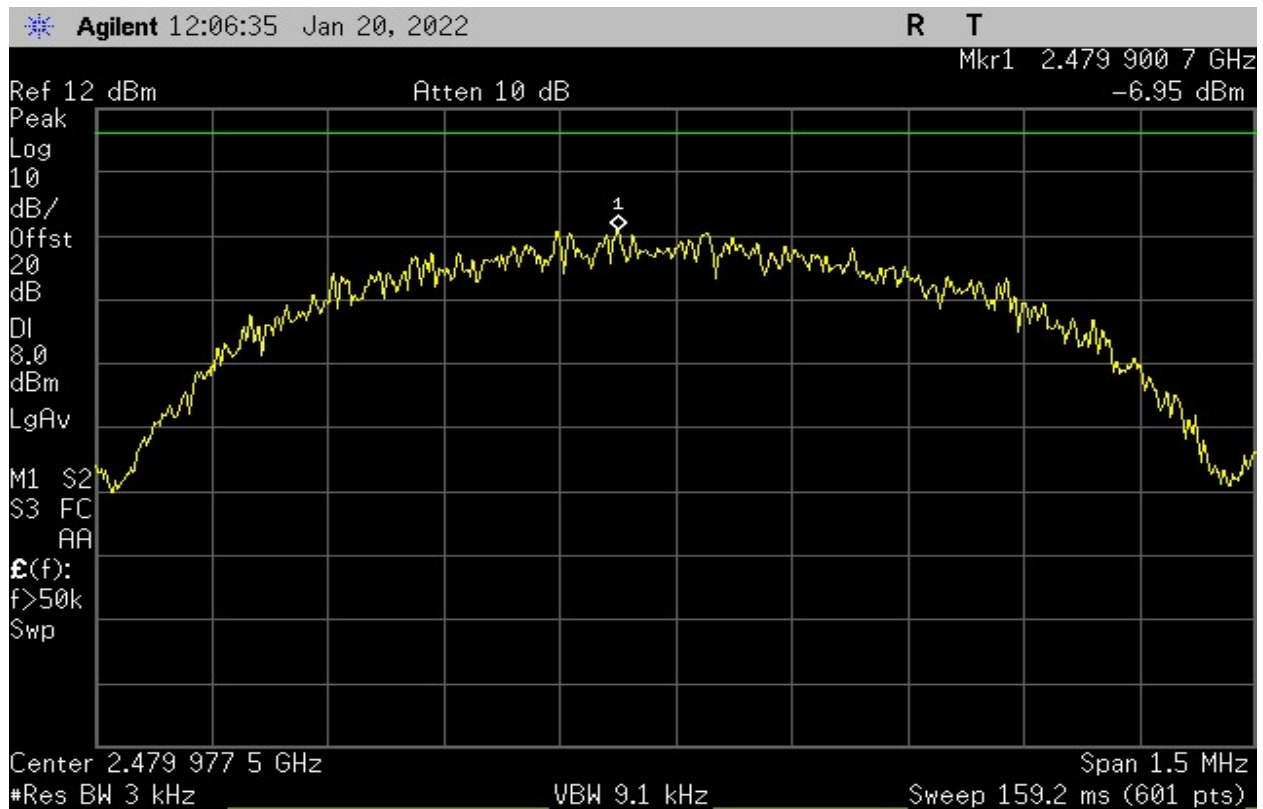
Plot 26 – Power Spectral Density – Highest Channel
