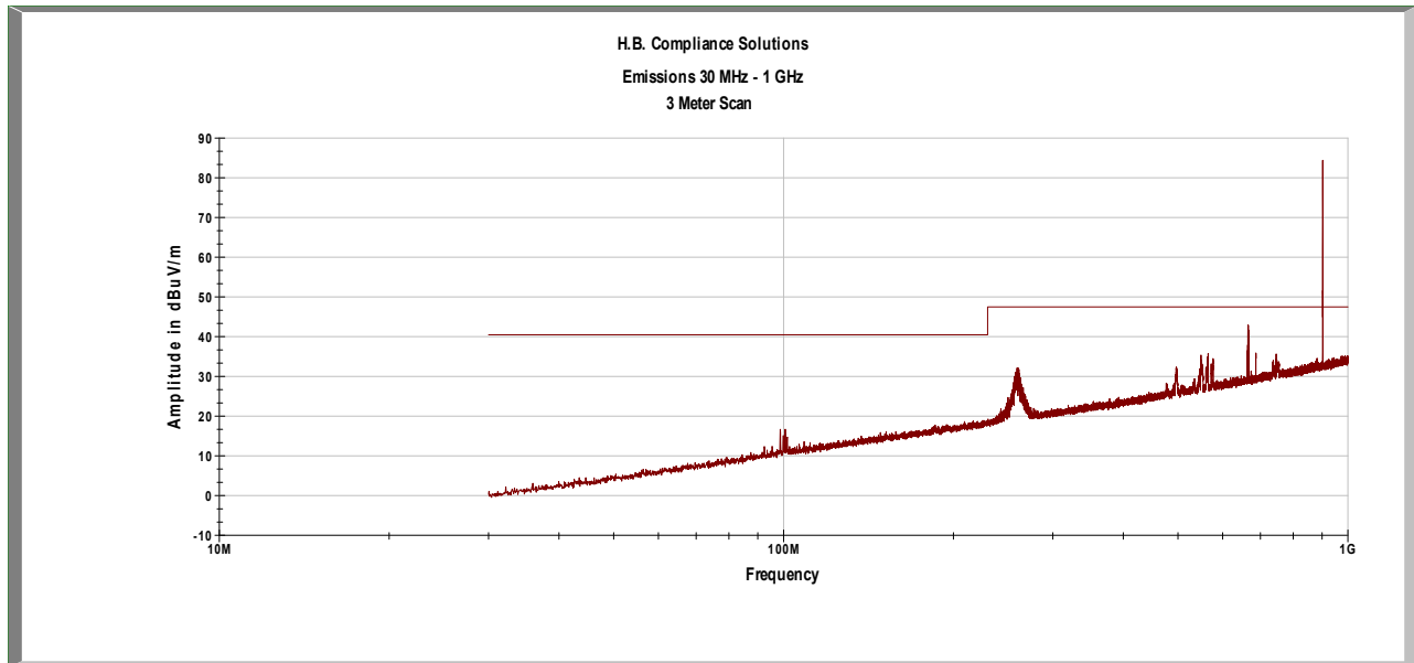
Plot 1 – Radiated Emissions – 30MHz to 1GHz – (Beacon)
