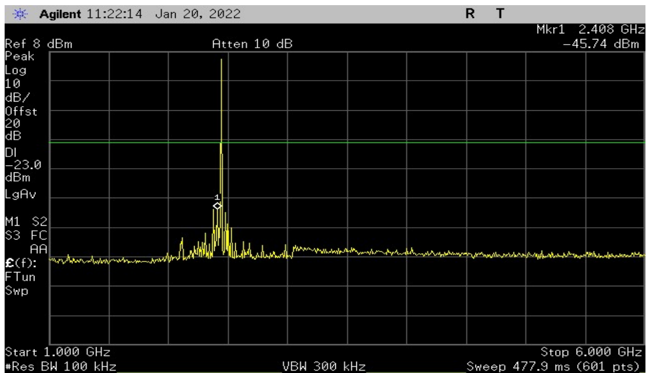
Plot 15 – Mid Band – 1GHz to 6GHz
