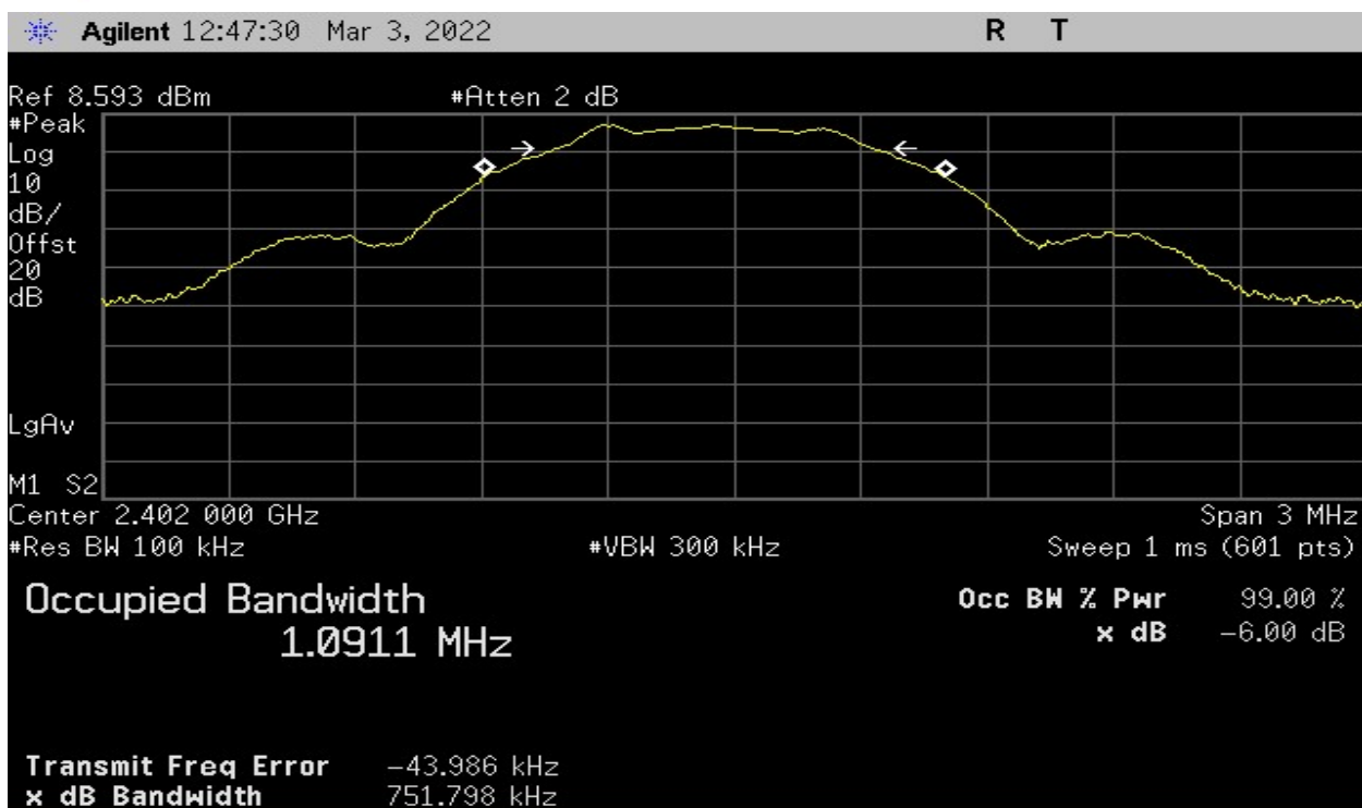
Plot 4 – Lowest Channel – 6dB BW
