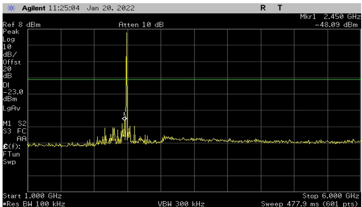
Plot 19 – High Band – 1GHz to 6GHz
