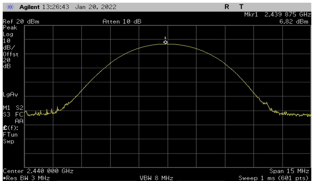
Plot 8 – Output Power – Middle Channel
