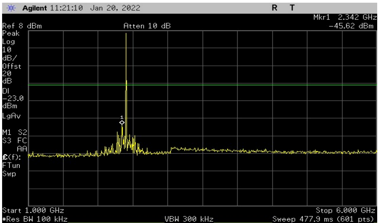
Plot 11 – Low Band – 1GHz to 6GHz
