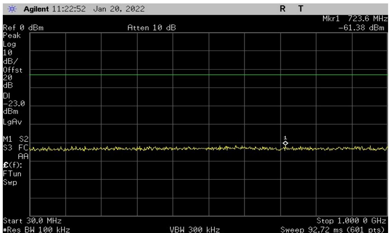
Plot 14 – Mid Band – 30MHz to 1000MHz
