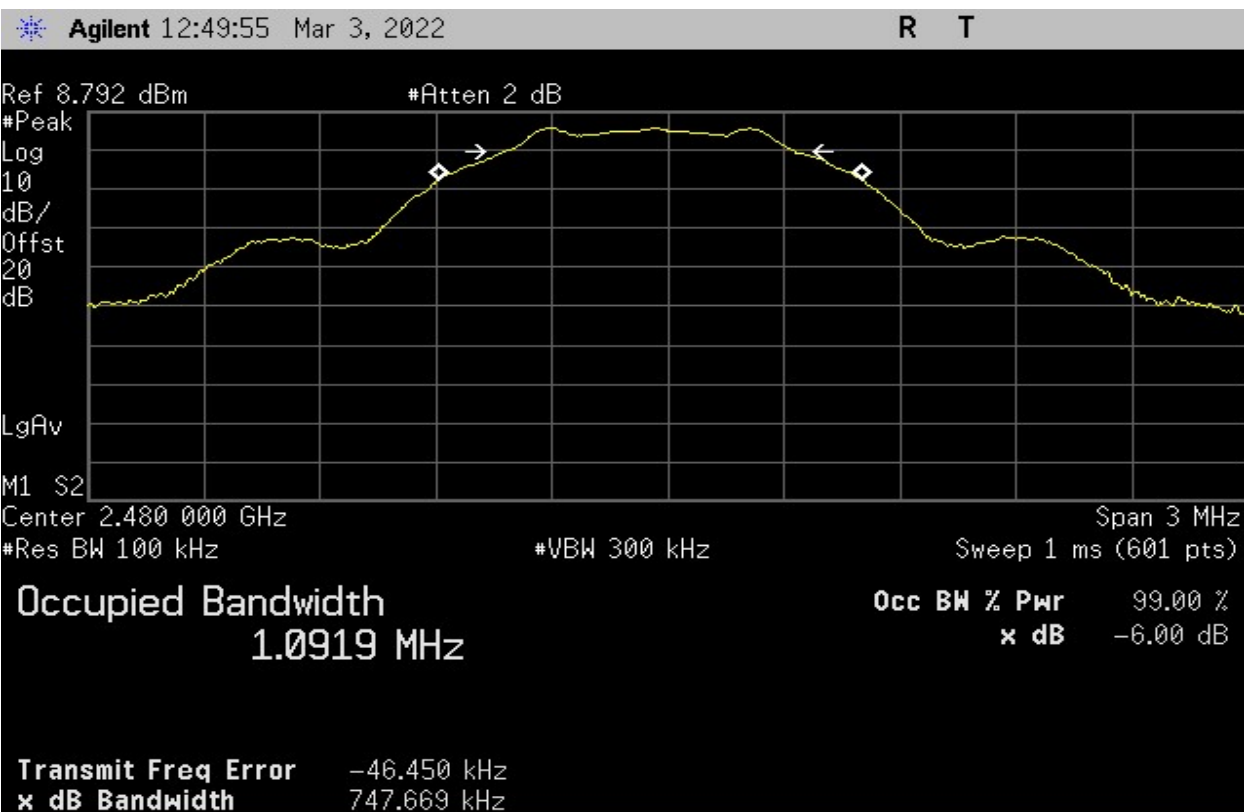
Plot 6 – Highest Channel – 6dB BW
