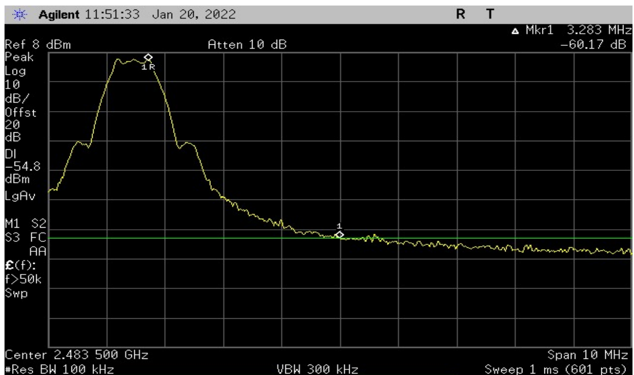
Plot 23 – Band Edge - High Channel
