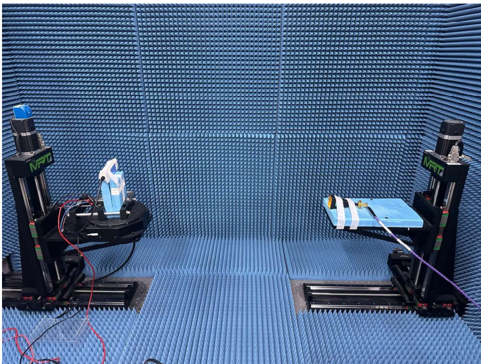
Test Set-up: Radiated spurious emission 40GHz to 50GHz
