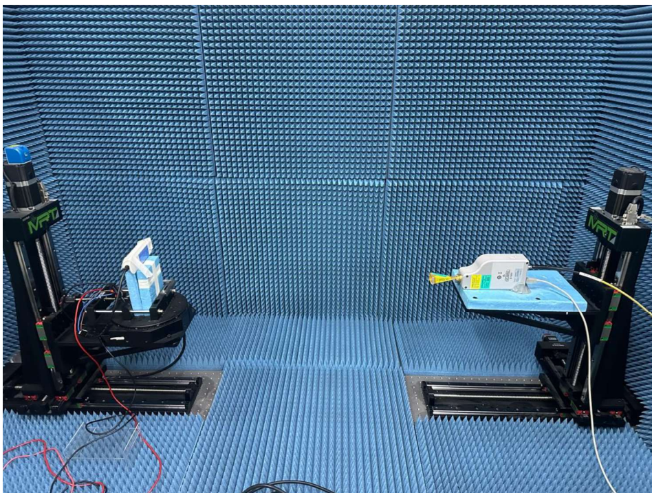
Test Set-up: Radiated spurious emission 75GHz to 100GHz
