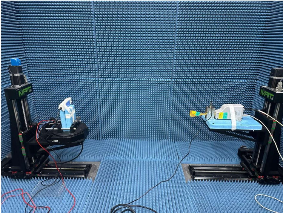
Test Set-up: Radiated spurious emission 50GHz to 75GHz
