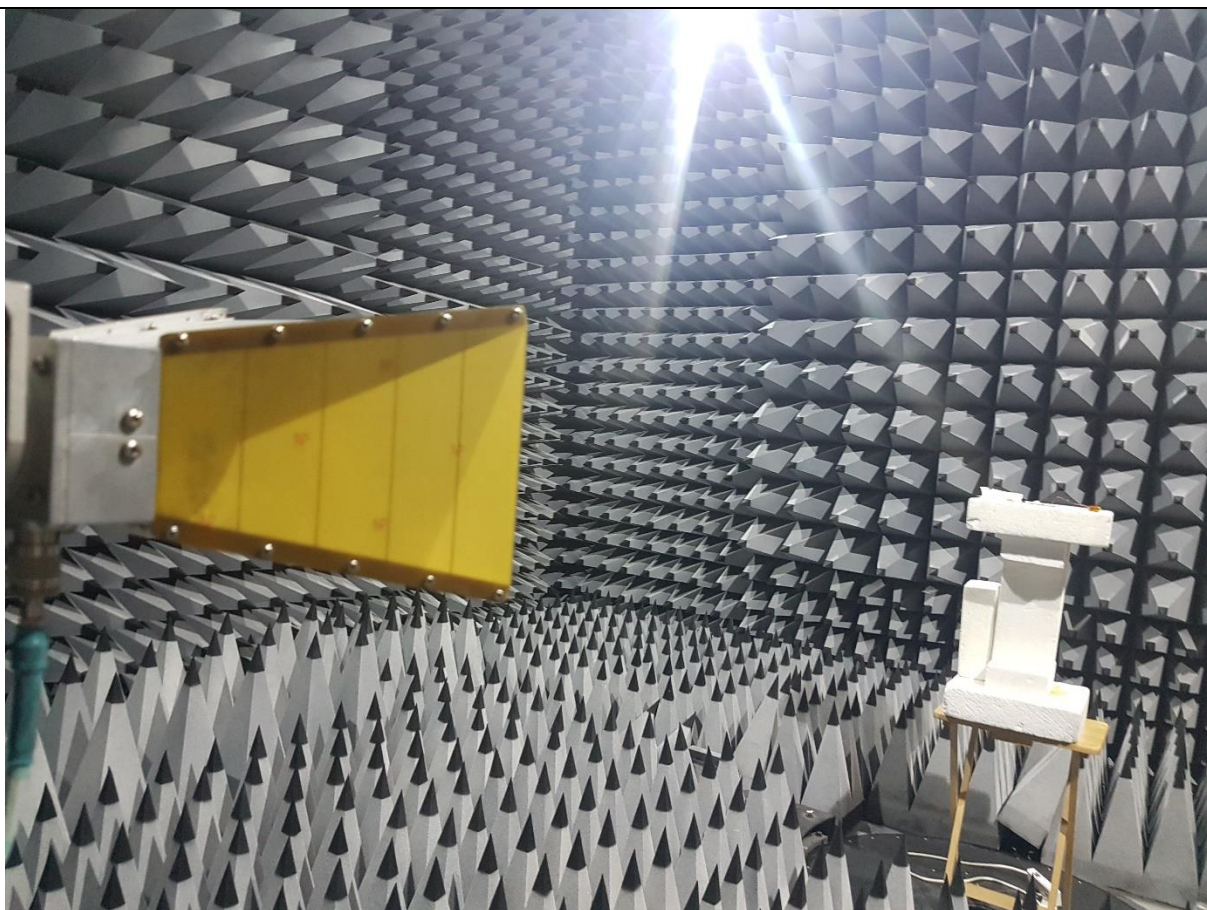
Fig 5 Radiated Emissions 1GHz -3.6GHz 3 metres
