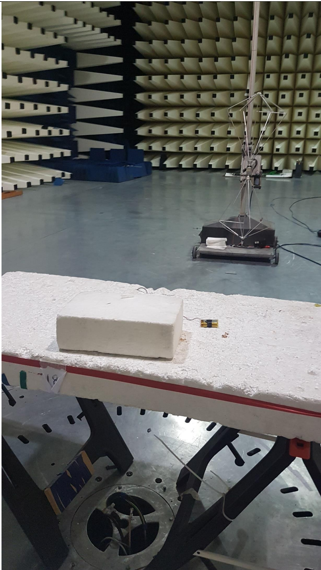
Fig 2 Radiated Emissions 30MHz - 300MHz 3 metres
