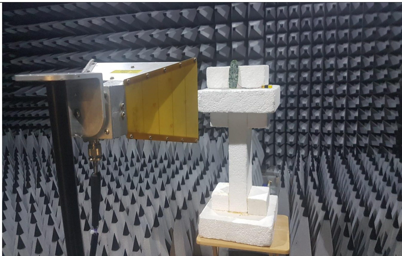
Fig 5 Radiated Emissions 1GHz -3.6GHz 3 metres
