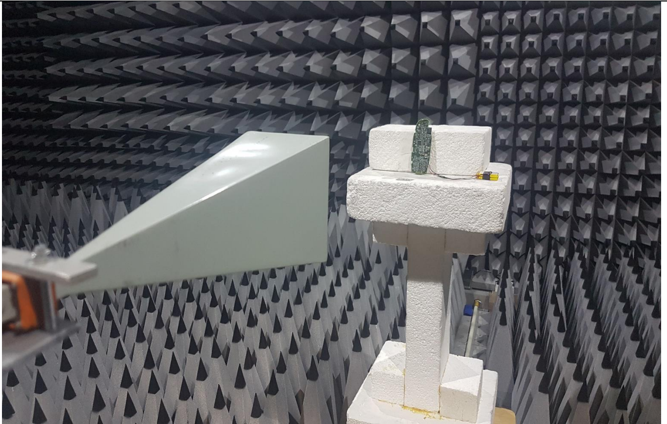
Fig 7 Radiated Emissions 18GHz -26GHz 1 metres
