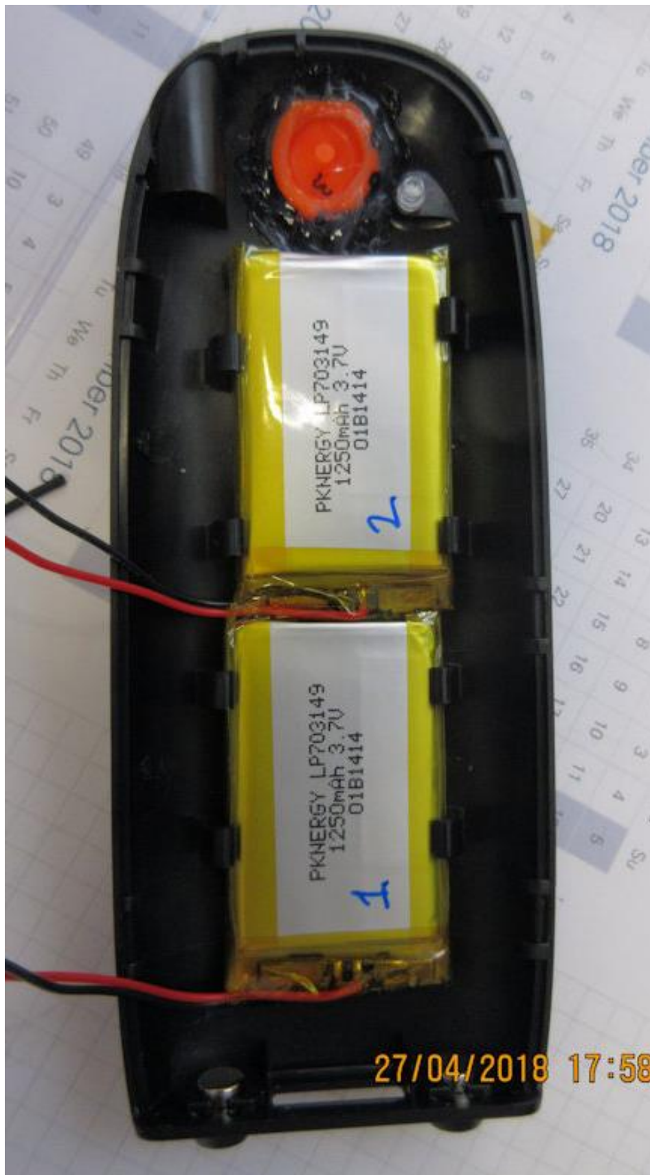
Internal battery location inside cover
