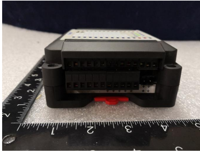
8.2 Front View
