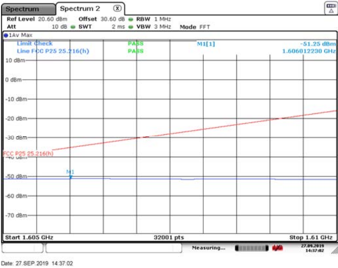
Figure 8.6-2: M. channel (QPSK)
