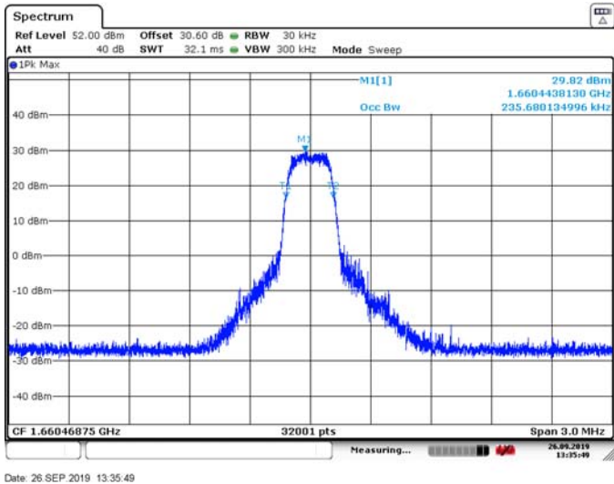
Figure 8.1-6: 99 % bandwidth on high channel(16APSK)
