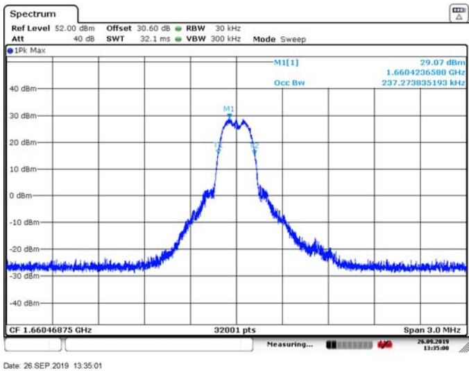
Figure 8.1-3: 99 % bandwidth on high channel(QPSK)
