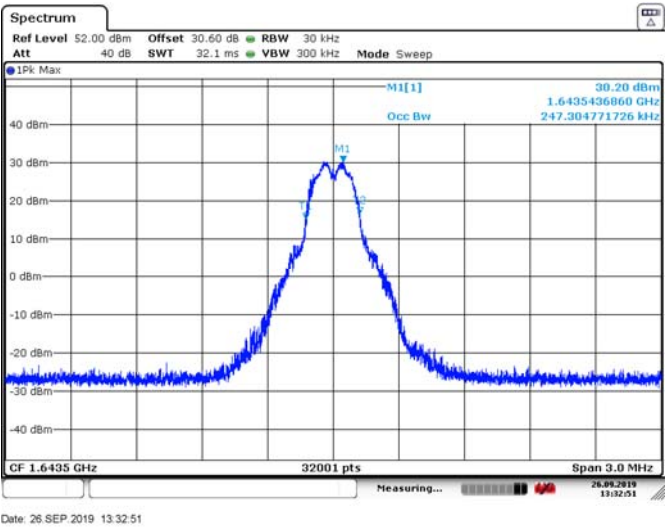
Figure 8.1-2: 99 % bandwidth on mid channel(QPSK)
