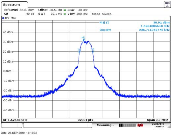
Figure 8.1-1: 99 % bandwidth on low channel (QPSK)
