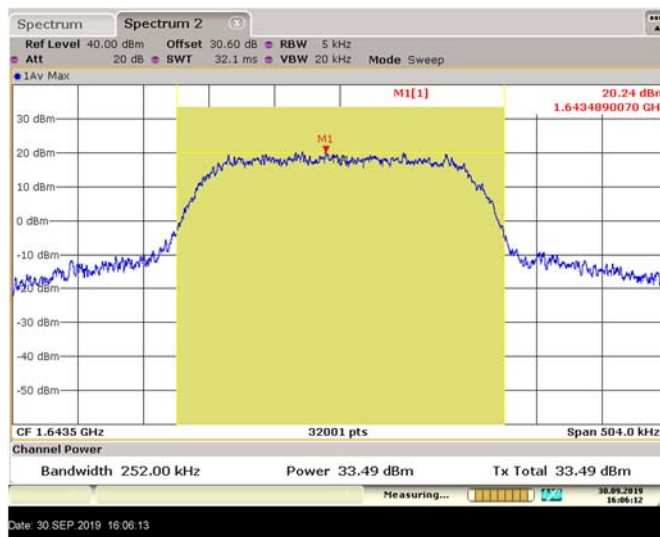
Figure 8.2-5: Power on mid channel (16APSK)
