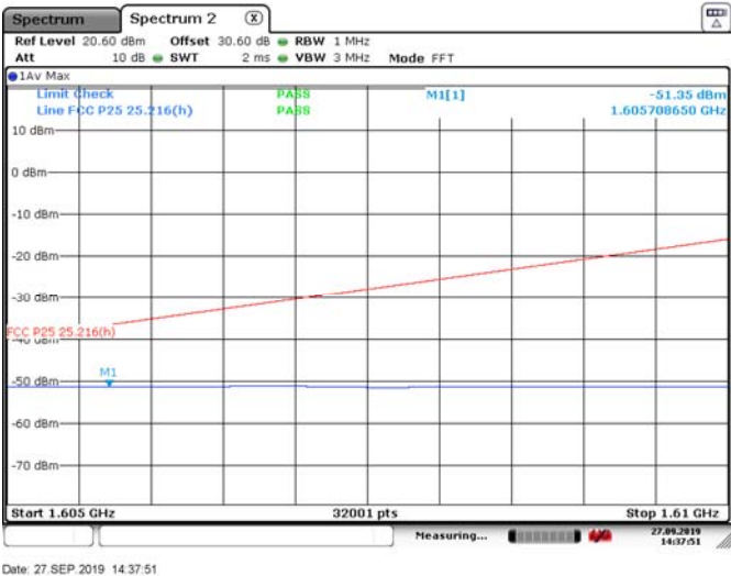
Figure 8.6-5: M channel (APSK)
