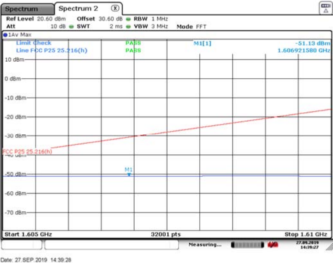
Figure 8.6-4: L channel (APSK)
