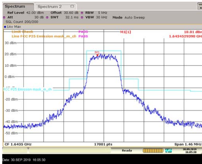
Figure 8.3-11: Emissions Mask M channel (APSK)
