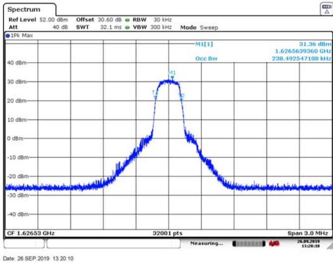
Figure 8.1-4: 99 % bandwidth on low channel (16APSK)
