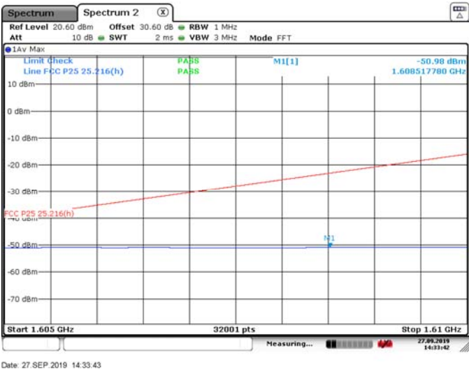
Figure 8.6-6: H channel (APSK)
