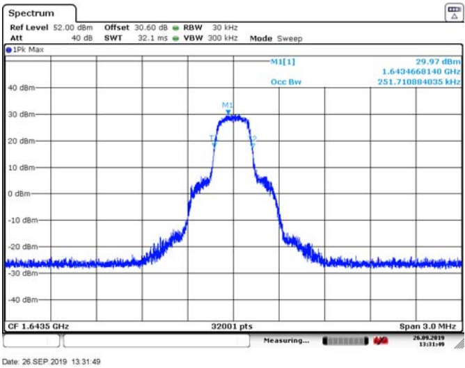
Figure 8.1-5: 99 % bandwidth on mid channel(16APSK)
