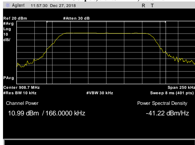
Plot 9. Power Output, 908.7 MHz, 10.99 dBm
