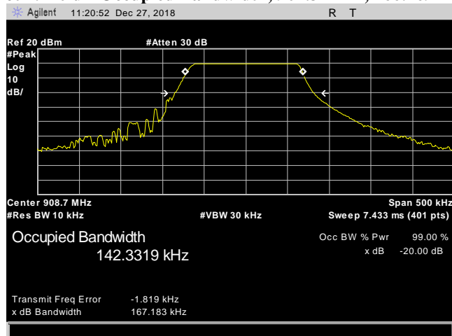
Plot 2. 20 dB Occupied Bandwidth, 908.7 MHz, 167.183 kHz
