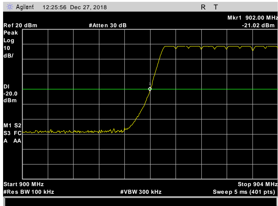
Plot 27. Conducted Band Edge, Hopping, Low Channel
