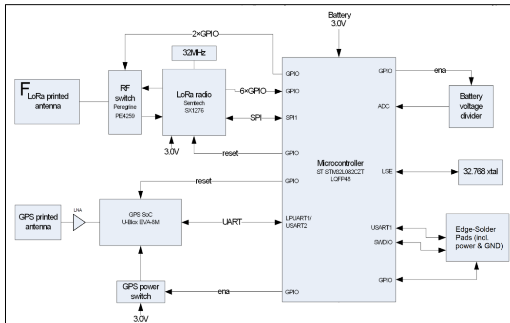
Figure 2. Block Diagram of Test Configuration
