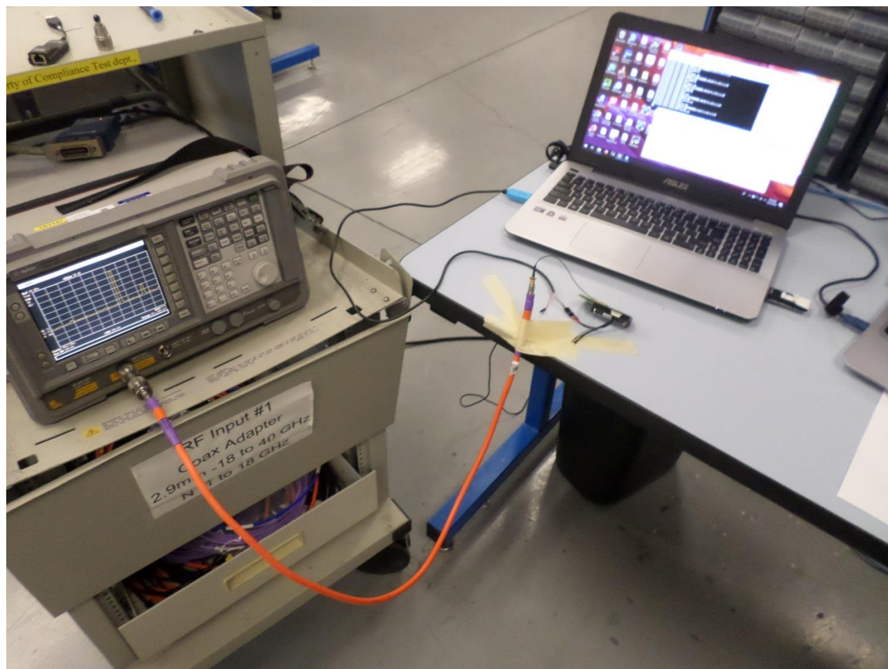
Photograph 7. Conducted Spurious Emissions, Test Setup
