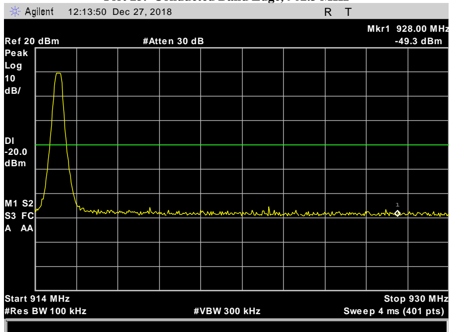
Plot 26. Conducted Band Edge, 914.9 MHz
