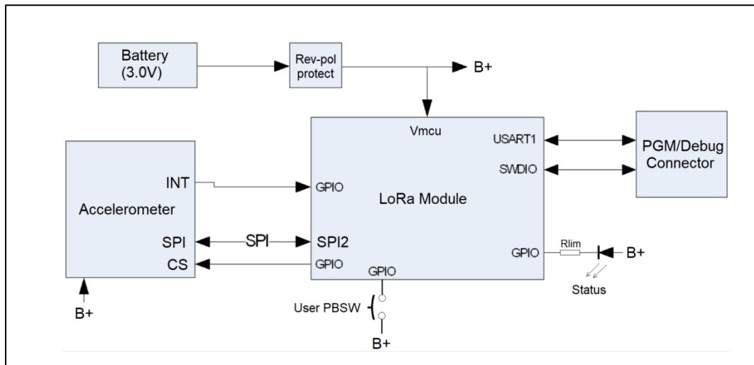
Figure 1: Asset Tracker: model: AAA Block Diagram containing LoRa Module
