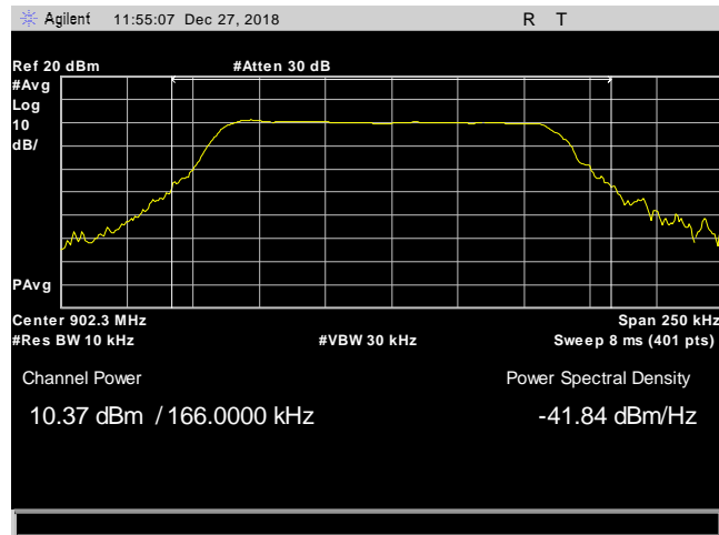
Plot 8. Power Output, 902.3 MHz, 10.37 dBm
