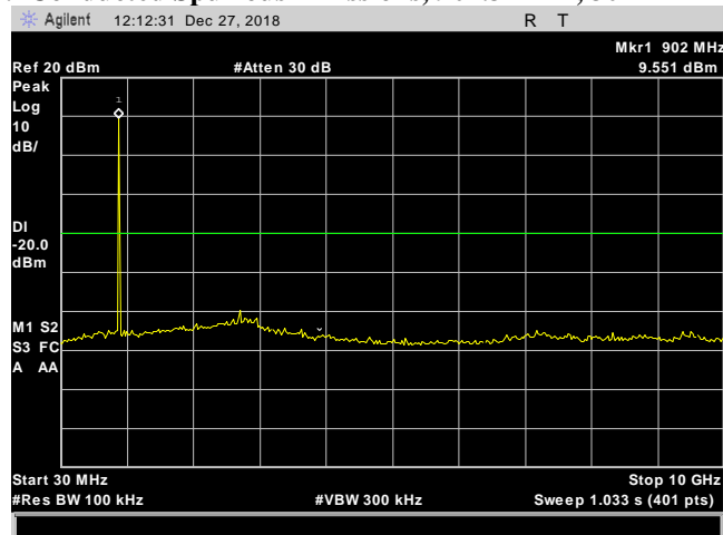
Plot 23. Conducted Spurious Emissions, 908.7 MHz, 30 MHz – 10 GHz
