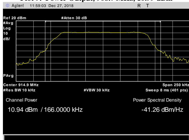
Plot 10. Power Output, 914.9 MHz, 10.94 dBm
