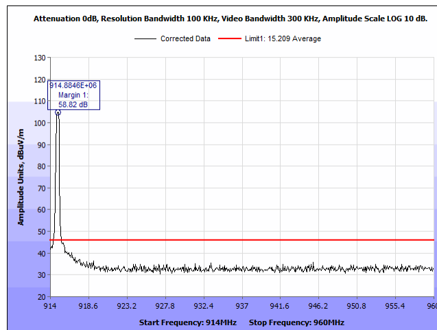
Plot 21. Radiated Restricted Band Edge, 914.9 MHz, Bandedge
