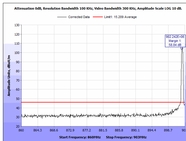
Plot 20. Radiated Restricted Band Edge, 902.3 MHz, Bandedge
