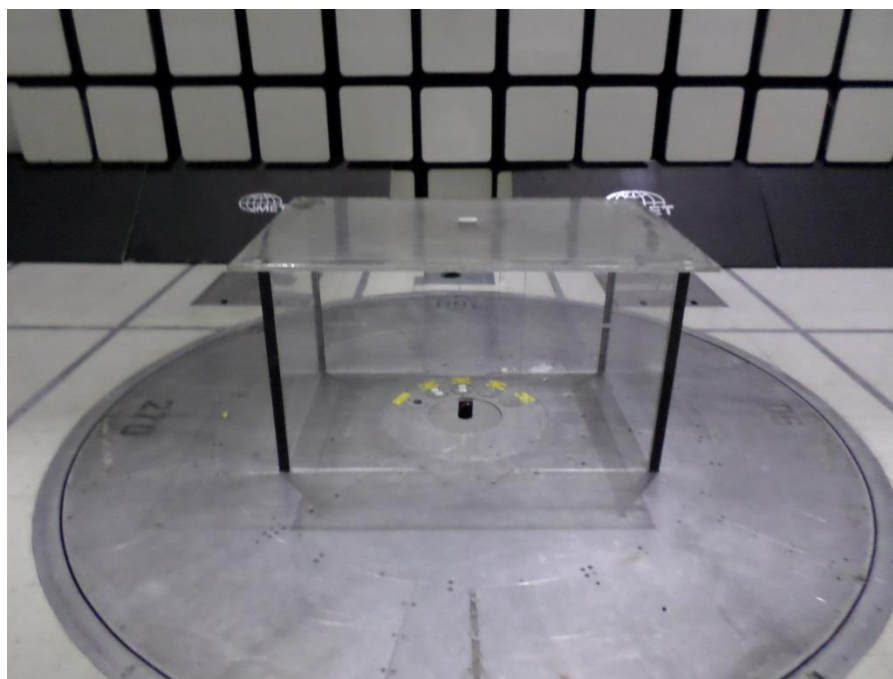
Photograph 2. Radiated Spurious Emissions, Below 1 GHz, Front, Test Setup
