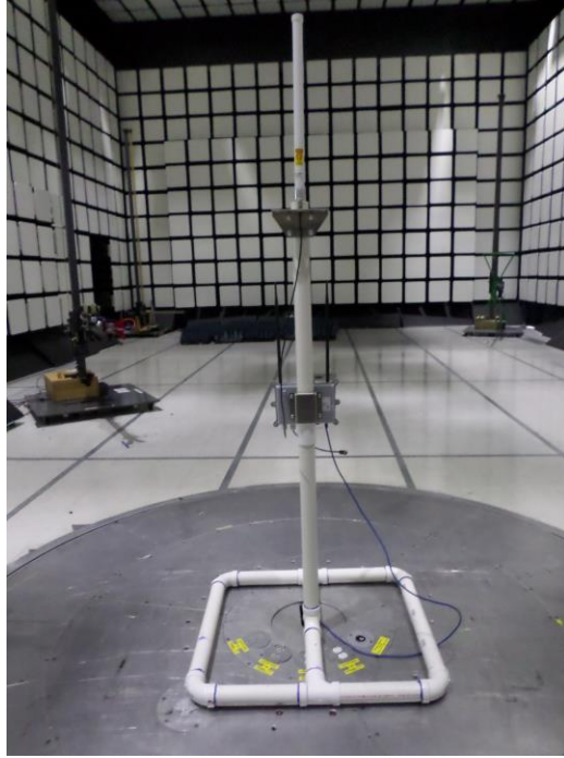
Photograph 6. Radiated Emissions, Setup Below 1GHz, Rear
