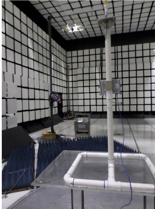
Photograph 8. Radiated Emissions, Setup Above 18 GHz, Rear
