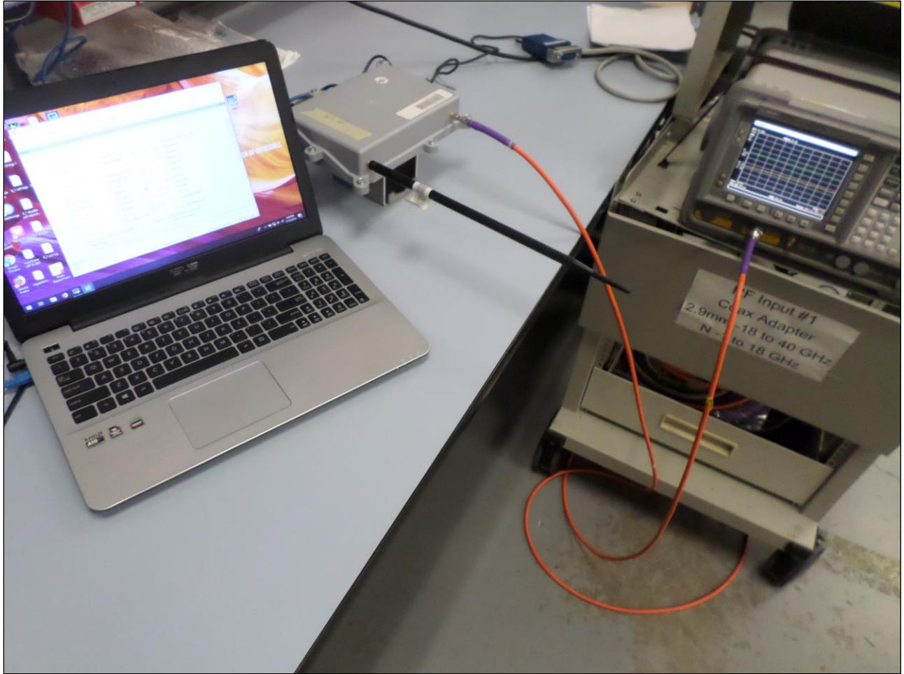
Photograph 3. Conducted Testing Setup
