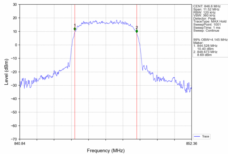
Band5_HSDPA_HCH_846.6MHz_Subtest 1_NTNV
