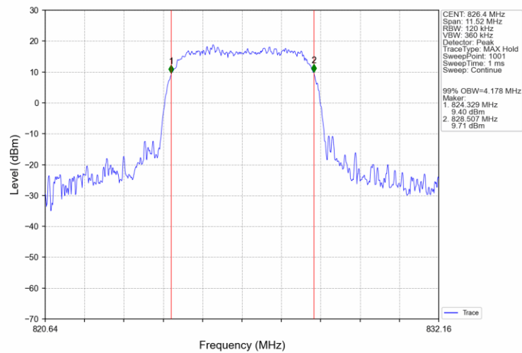
Band5_HSDPA_LCH_826.4MHz_Subtest 1_NTNV
