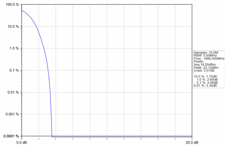
Band2_RMC_MCH_1880MHz_12.2kbps RMC_NTNV
