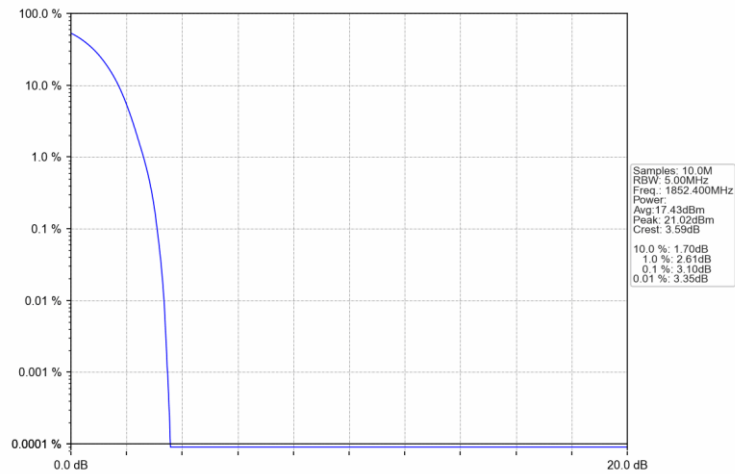
Band2_RMC_LCH_1852.4MHz_12.2kbps RMC_NTNV
