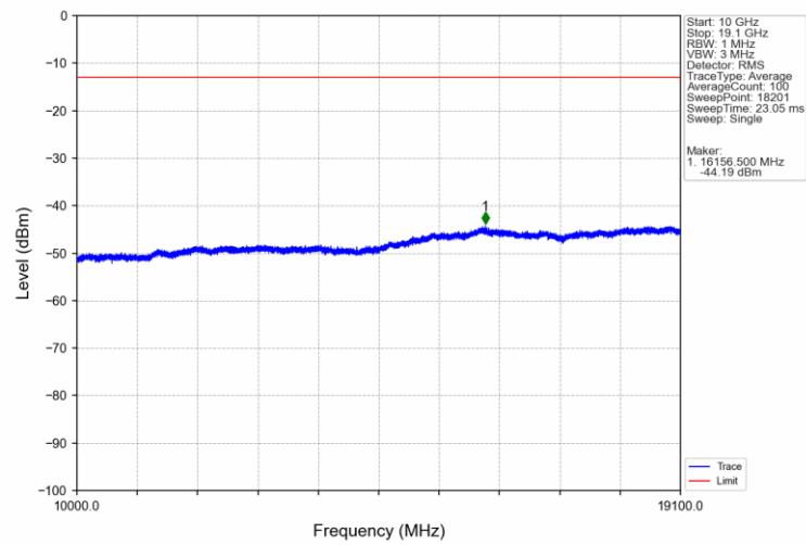
Band2_RMC_LCH_1852.4MHz_12.2kbps RMC_NTNV
