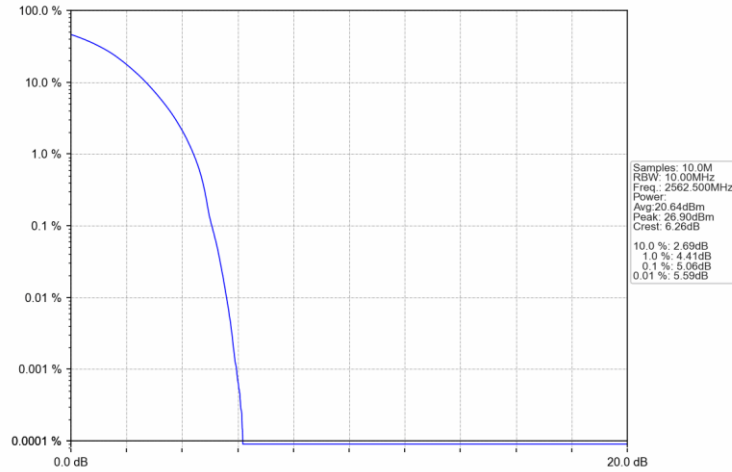
Band7_15MHz_QPSK_HCH_2562.5MHz_RB_75_0_NTNV
