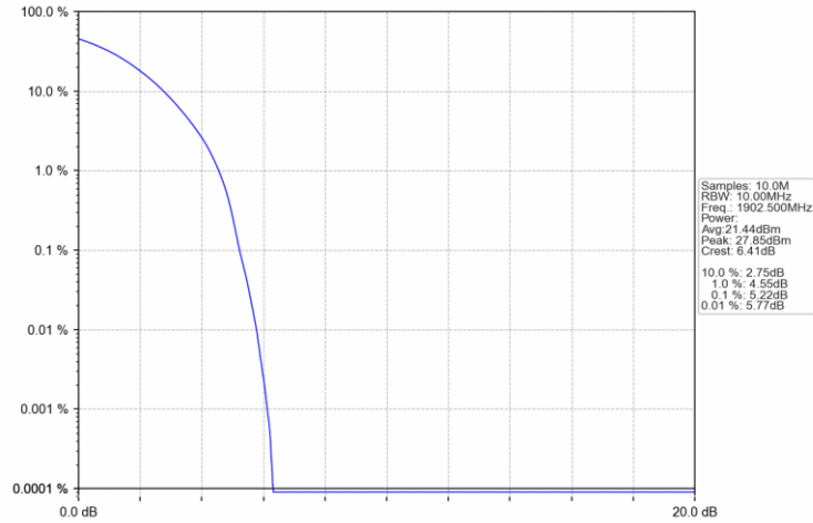
Band2_15MHz_QPSK_HCH_1902.5MHz_RB_75_0_NTNV
