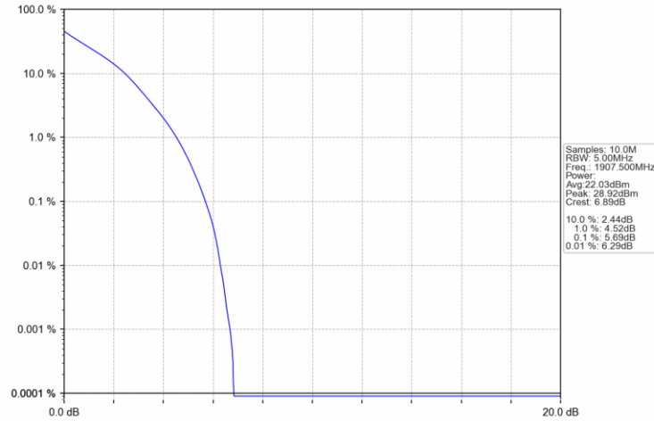
Band2_5MHz_QPSK_HCH_1907.5MHz_RB_25_0_NTNV
