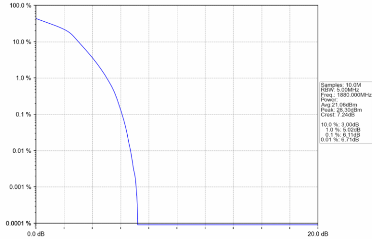
Band2_1.4MHz_16QAM_MCH_1880MHz_RB_6_0_NTNV
