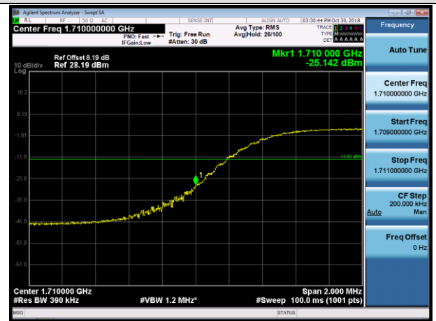
LCH_16QAM_50RB#0
