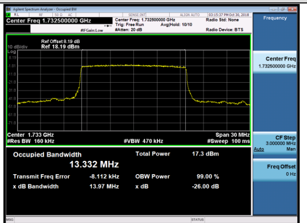
MCH_16QAM_75RB#0
