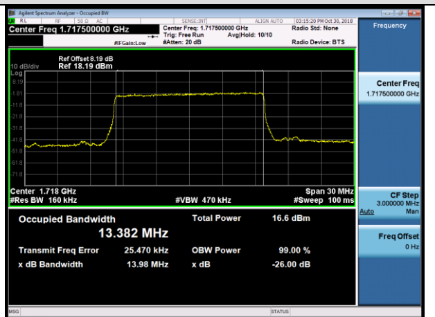
LCH_16QAM_75RB#0
