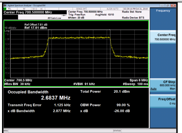
LCH_16QAM_15RB#0
