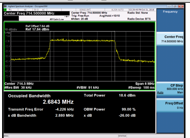
HCH_16QAM_15RB#0
