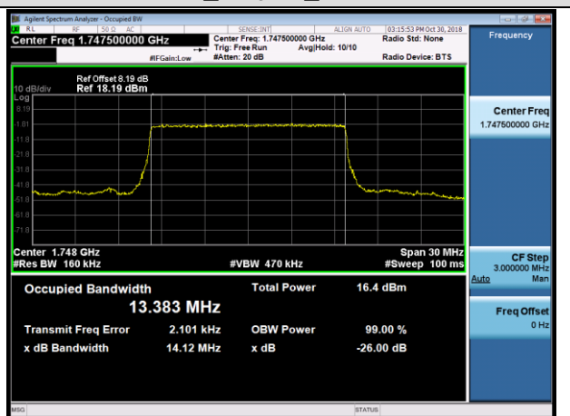
HCH_16QAM_75RB#0
