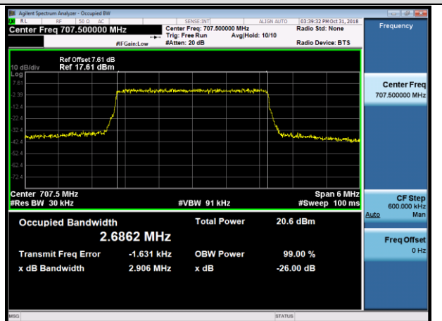
MCH_16QAM_15RB#0
