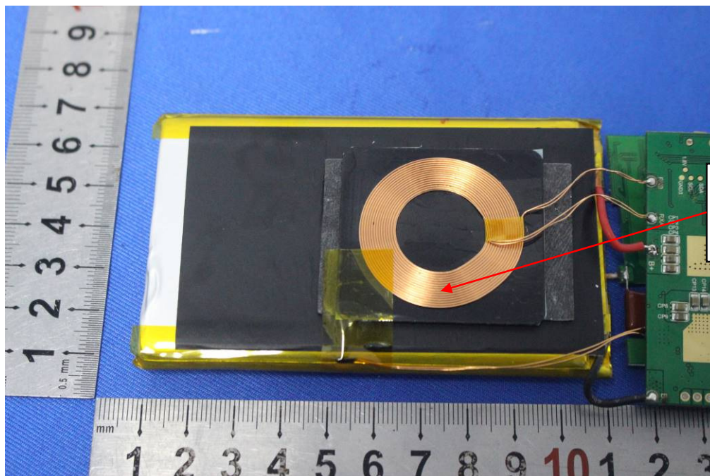
Receiver antenna
