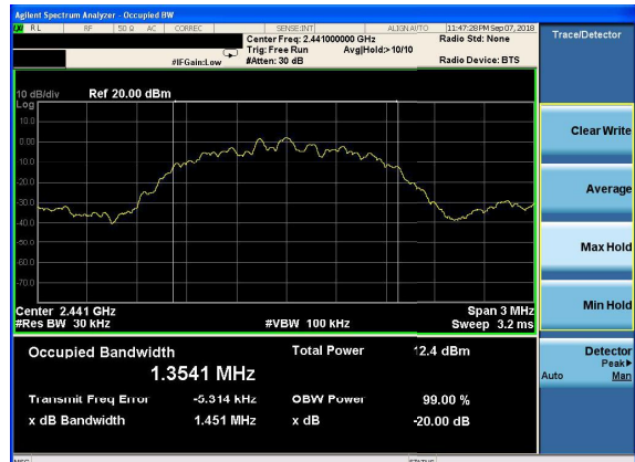
20dB Bandwidth plot on channel 39 (2Mbps)
