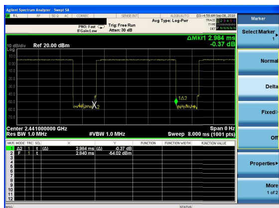
Package Transfer Time Plot CH39-3DH5
