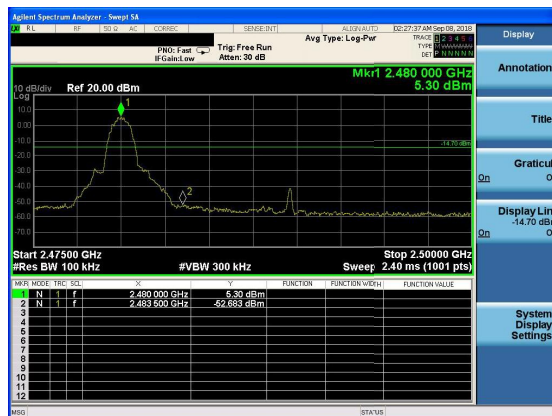
8-DPSK: Band Edge-High Channel
