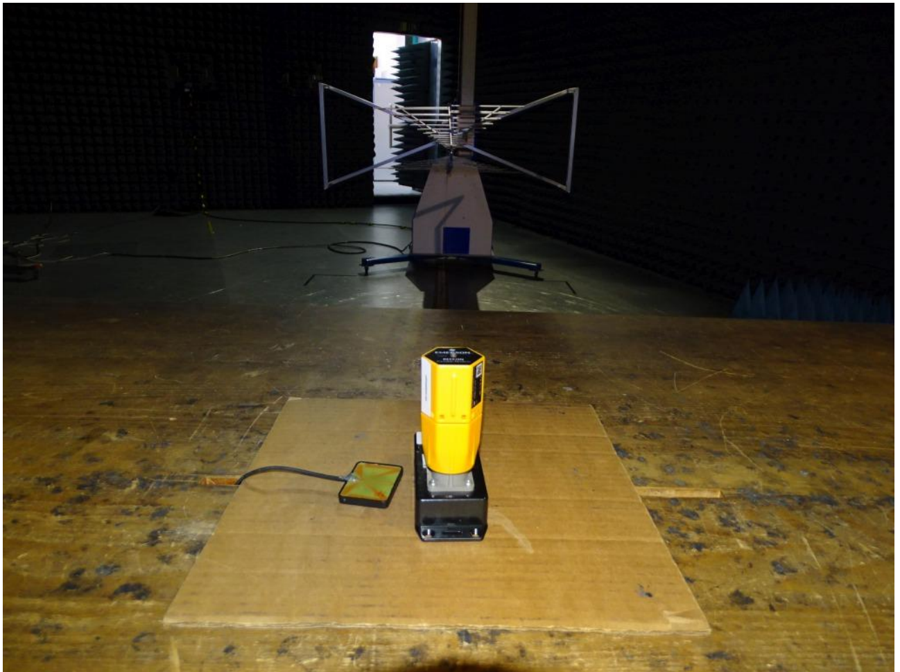
Photo 3: Test setup for radiated measurements below 1 GHz, detailed view, rear side , EUT vertical
