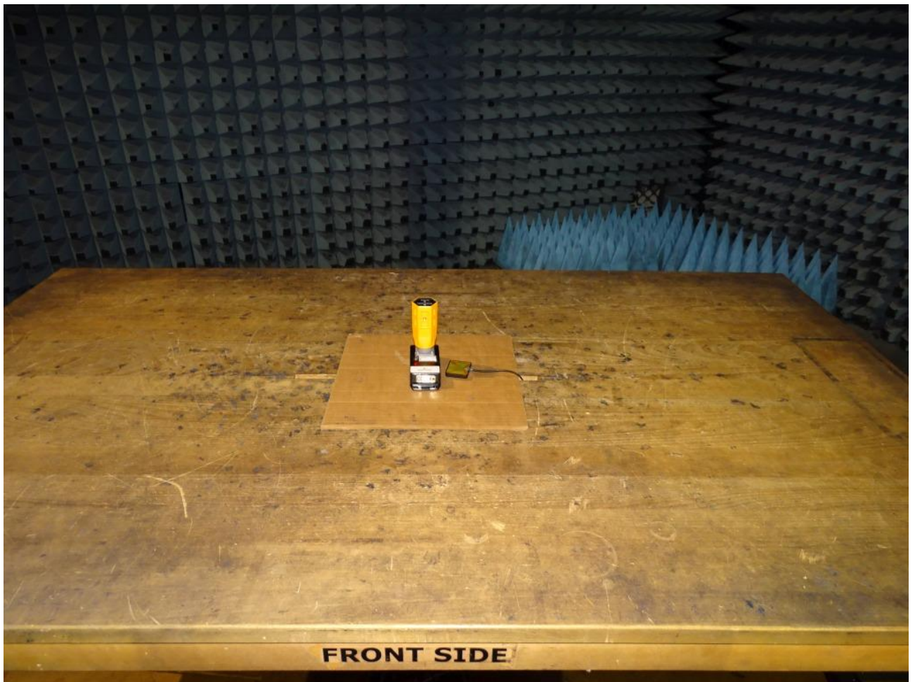
Photo 1: Test setup for radiated measurements below 1 GHz, front side view
