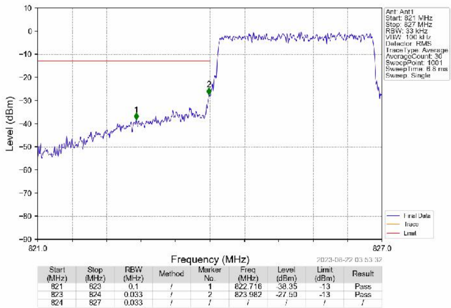
Band5_3MHz_16QAM_LCH_825.5MHz_RB_15_0_NTNV
