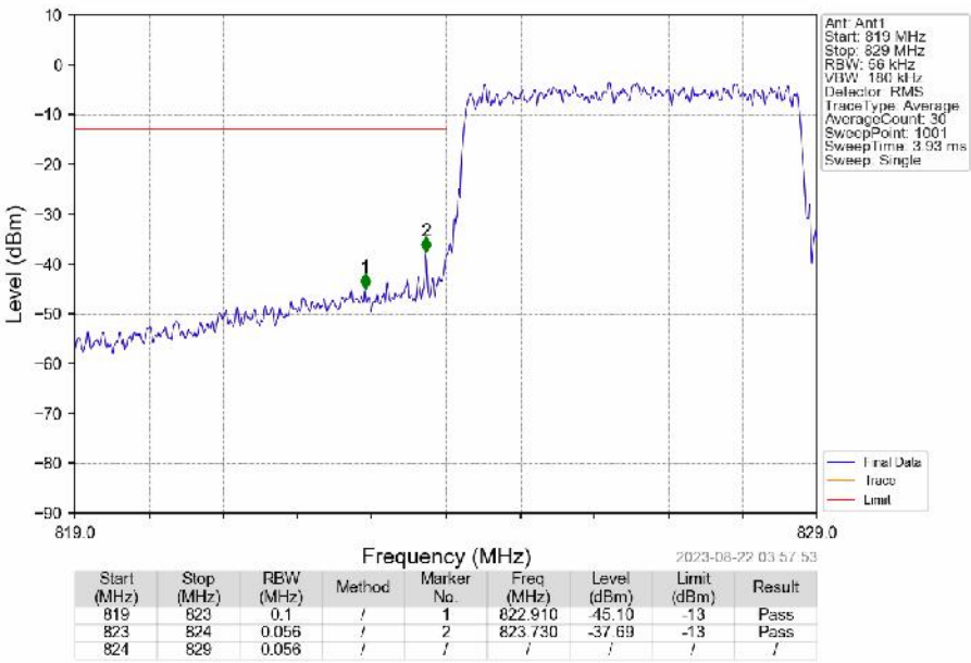
Band5_5MHz_16QAM_LCH_826.5MHz_RB_25_0_NTNV
