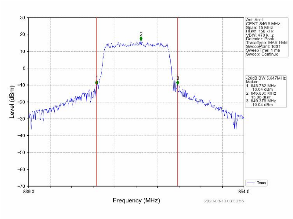
Band5_5MHz_16QAM_HCH_846.5MHz_RB_25_0_NTNV
