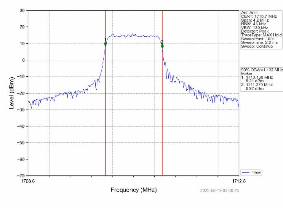
Band4_1.4MHz_16QAM_LCH_1710.7MHz_RB_6_0_NTNV
