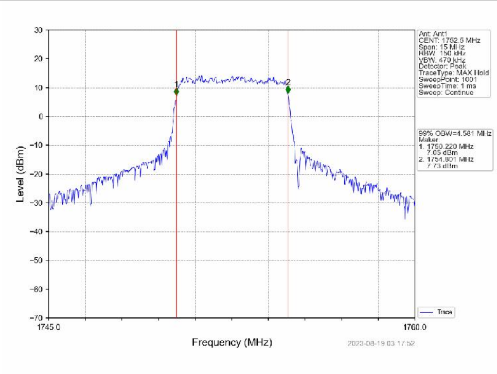
Band4_5MHz_16QAM_HCH_1752.5MHz_RB_25_0_NTNV
