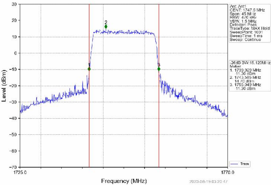
Band4_15MHz_16QAM_HCH_1747.5MHz_RB_75_0_NTNV
