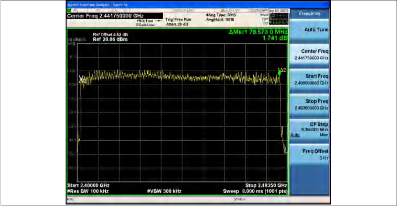
Number_of_Hopping_Channel (Hopping)_NVNT_ANT1_2-DH5_Hopping
