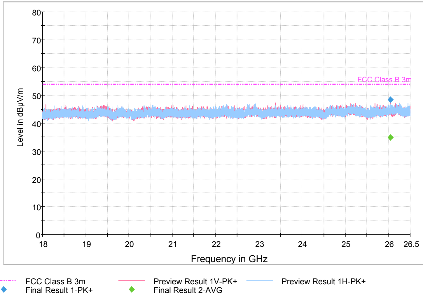
FCC Class B Radiated Scan 18GHz-26.5GHz 3m PK AVG
