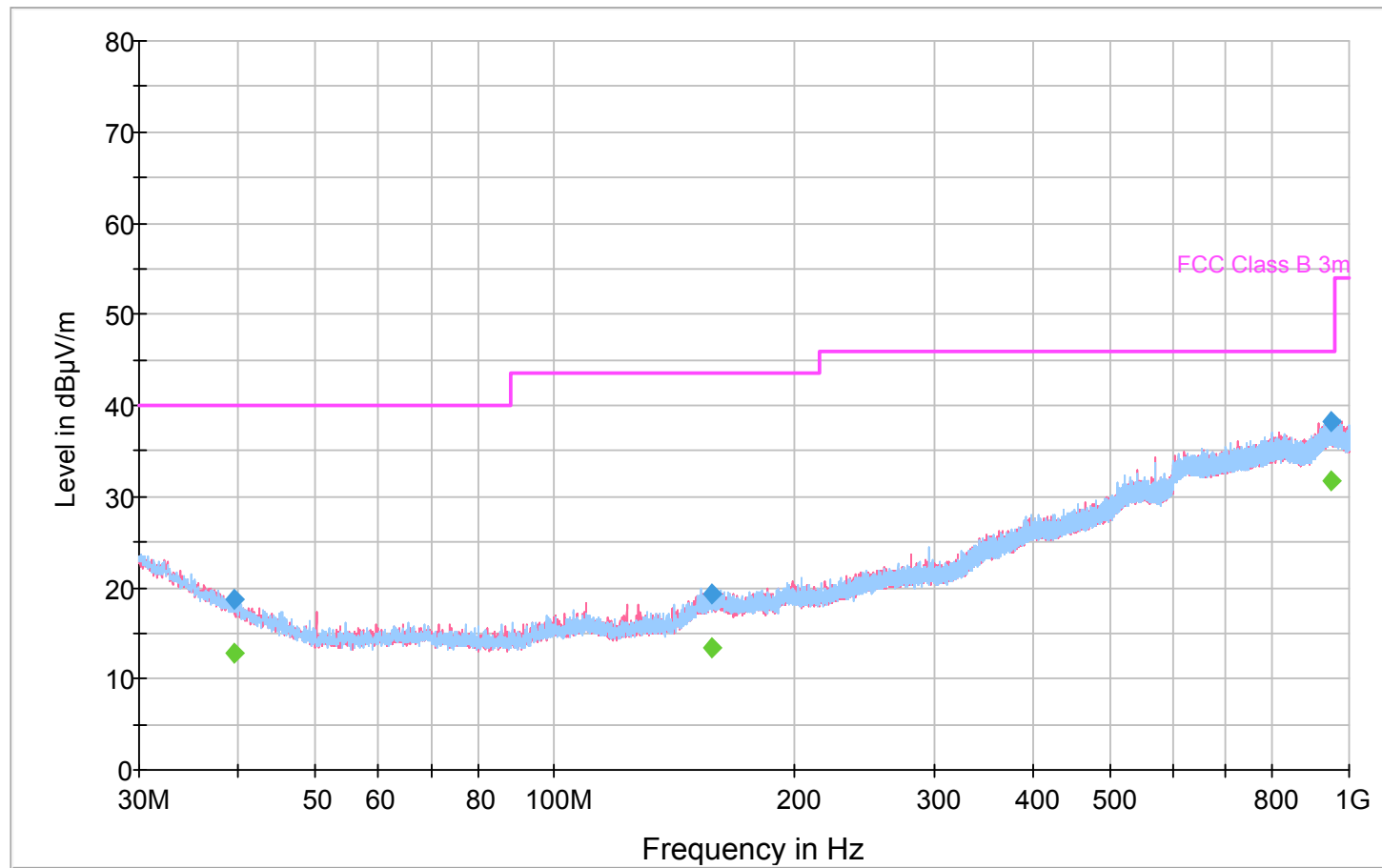
FCC Class B Radiated Scan 3m PK QP2
