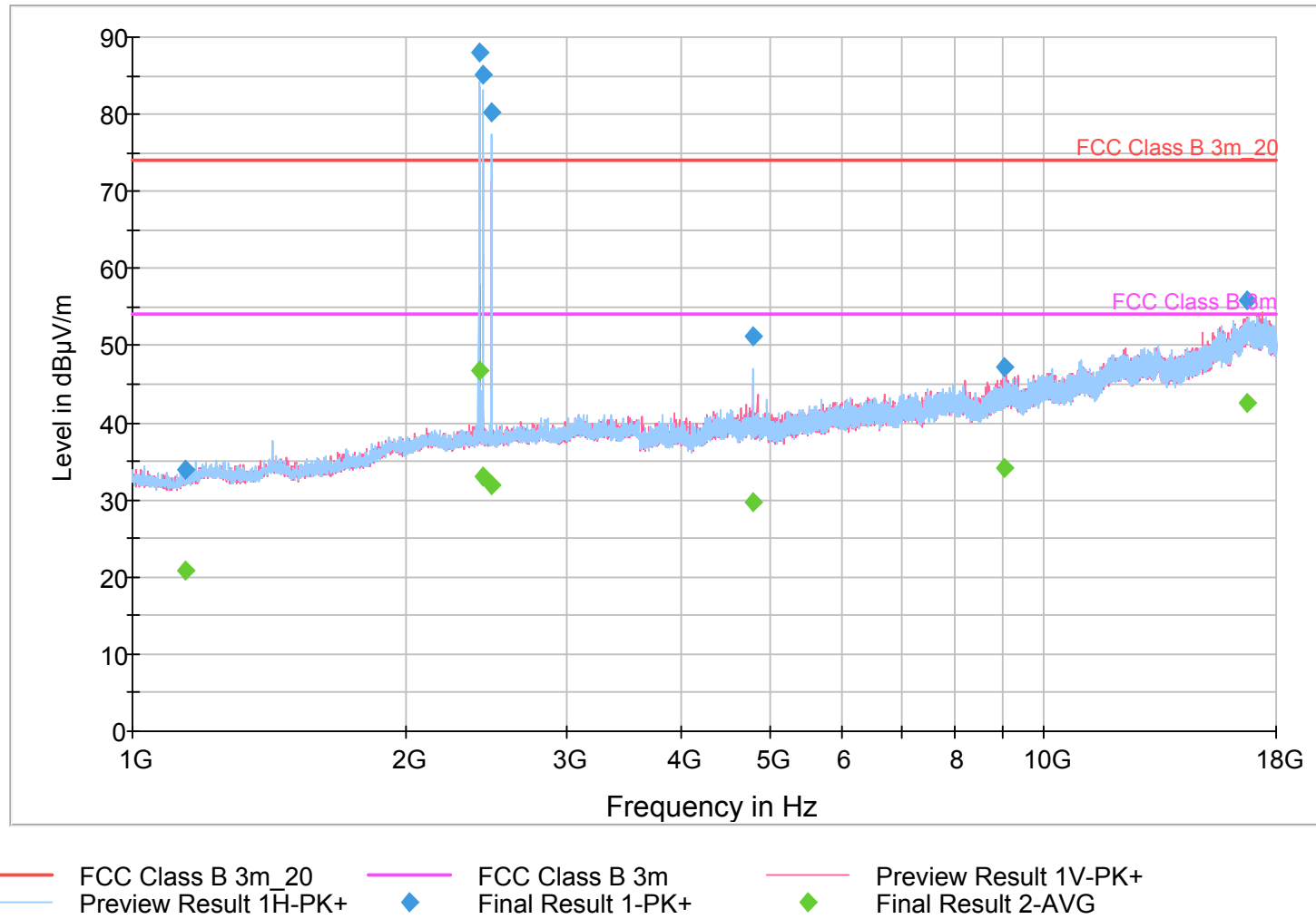
FCC Class B Radiated Sweep 1GHz-18GHz 3m PK AVG
