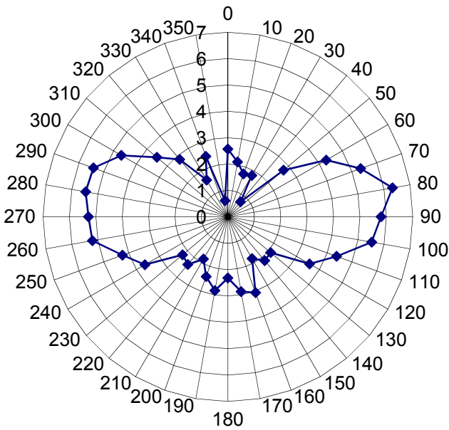
9350 MHz - Vertical– Gain (dBi)
